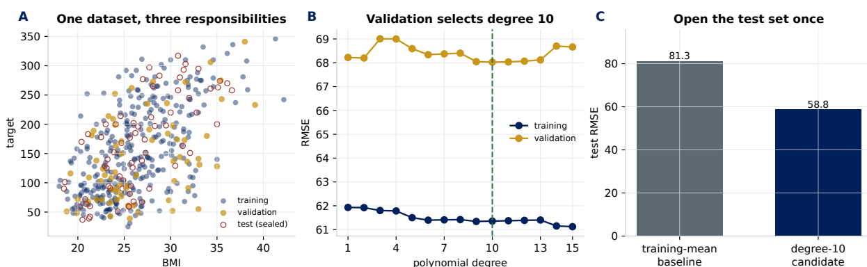
Figure 11.1: Training estimates parameters, validation supports adaptive choices, and test data estimate the performance of the completed procedure. Re-running model selection after viewing panel C would turn the test set into development data.
