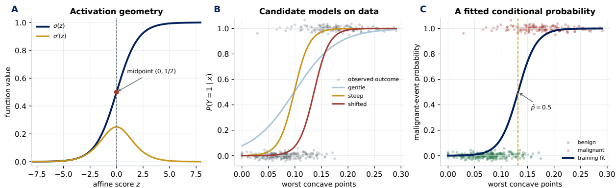
Figure 14.2: From activation to data. A: The sigmoid maps every real score to (0, 1) ; its derivative is largest at the midpoint and vanishes in the saturated tails. B: Several sigmoid curves can be placed over the same binary observations, so shape must be learned rather than selected by eye. C: A one-feature logistic model fitted on a training split of the Wisconsin Diagnostic Breast Cancer data produces a conditional malignant-event probability. Vertical jitter only reveals overlapping binary outcomes; it is not a new response value.
