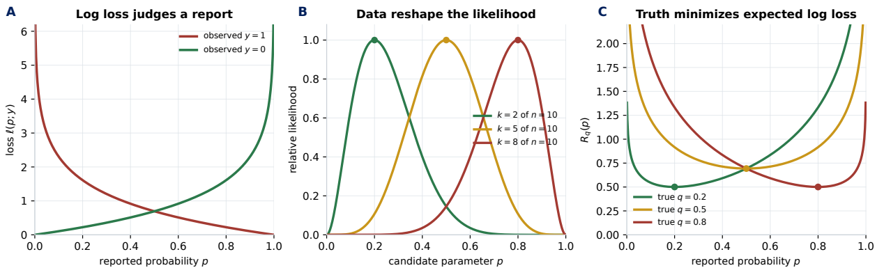
Figure 14.3: Three views of the Bernoulli model. A: Per-observation log loss rewards probability assigned to the observed outcome and sharply penalizes confident errors. B: With k events in ten trials, the likelihood is maximized at \hat{p} = k/10 ; its width records finite-sample uncertainty. Curves are normalized only for visual comparison. C: If the true event probability is q , expected log loss is uniquely minimized by reporting p = q .
