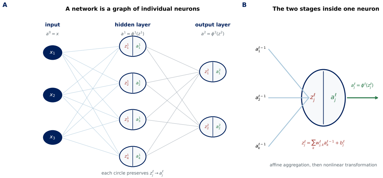
Figure 17.1: A layered network shown without hiding the individual neurons. Panel A distinguishes the affine preactivation z_j^\ell from the postactivation a_j^\ell at every hidden and output node. Panel B enlarges one neuron: incoming postactivations are aggregated affinely and then transformed. Matrix notation evaluates these same scalar operations in parallel.
