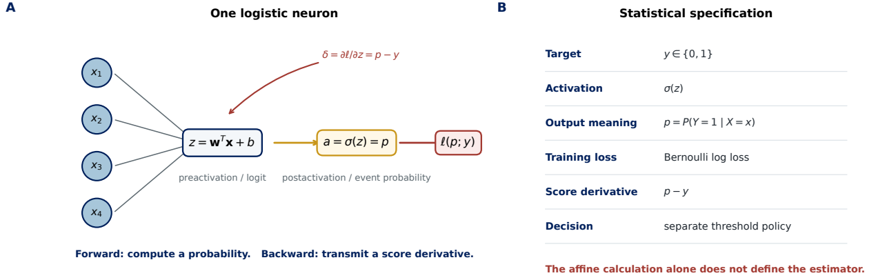
Figure 14.1: The logistic single-neuron contract. A : A forward pass forms the preactivation z = w^T x + b and the postactivation a = \sigma(z) = p . Bernoulli log loss returns the score derivative \delta = \partial \ell / \partial z = p - y during the backward calculation. B : The computational graph becomes a statistical estimator only after its target, activation, loss, output meaning, and decision boundary are specified.
