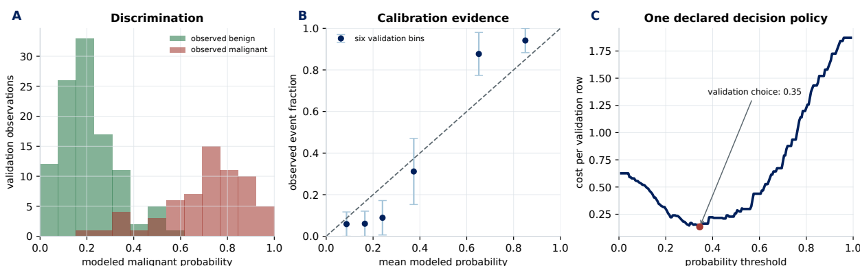
Figure 14.4: Three forms of validation evidence from the repository’s breast cancer table. A: Class-conditional probability histograms describe discrimination. B: Binned event fractions with 95 percent Wilson intervals provide limited calibration evidence; the intervals expose the small validation sample. C: A threshold is chosen for one explicitly hypothetical cost model in which a false negative costs five times a false positive. Changing that cost model can change the action rule without changing the fitted probability model.
