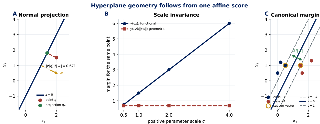
Figure 15.1: The derivation of maximum-margin geometry for z(x) = 2x_1 - x_2 - 1 . A: Orthogonal projection onto z = 0 follows the normal w and gives distance |z(q)|/\|w\|_2 . B: rescaling (w, b) changes functional margin but not normalized geometric margin. C: canonical scaling places the closest observations on z = \pm 1 ; the perpendicular distance between these supporting levels is 2/\|w\|_2 . The figure is generated by the same NumPy and Matplotlib construction used in Lecture 11 notebook 01.
