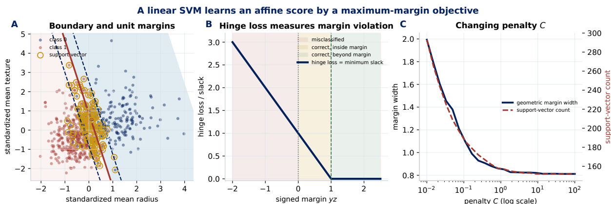
Figure 15.2: A linear SVM fitted to versioned diagnostic measurements. Left: decision boundary, unit margins, and support vectors. Center: the three geometric regions of signed margin and the hinge loss each produces. Right: regularization changes margin width and the number of active observations.
