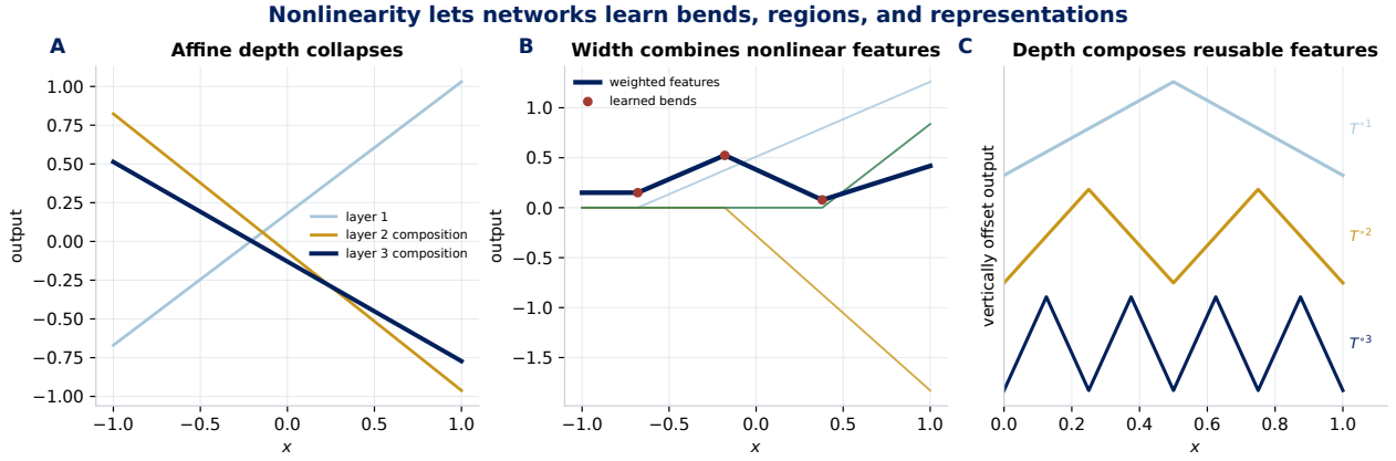
Figure 17.2: Where expressive power enters. Panel A confirms that composing affine layers still produces one affine function. Panel B combines several ReLU hinge features to create a piecewise-linear function with multiple learned bends. Panel C composes the same tent feature: depth reuses an earlier computation and increases the number of linear regions. Expressive capacity is useful only when supported by data, regularization, and held-out evidence.
