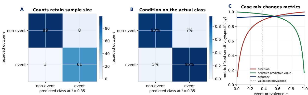
Figure 14.5: A confusion matrix is contextual evidence, not a permanent model attribute. A: Counts retain the validation sample size at the threshold selected under the explicitly hypothetical five-to-one error cost. B: Row normalization conditions on the recorded actual class and exposes sensitivity and specificity. C: Holding those two rates fixed while changing prevalence still changes precision, negative predictive value, and accuracy. The vertical line marks only this validation sample's prevalence; it is not a deployment estimate.
