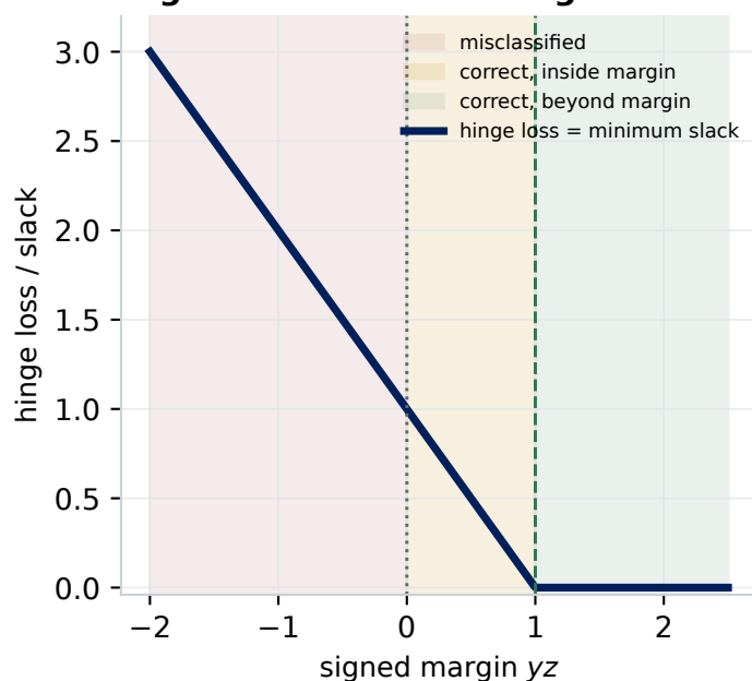
Hinge loss measures margin violation
