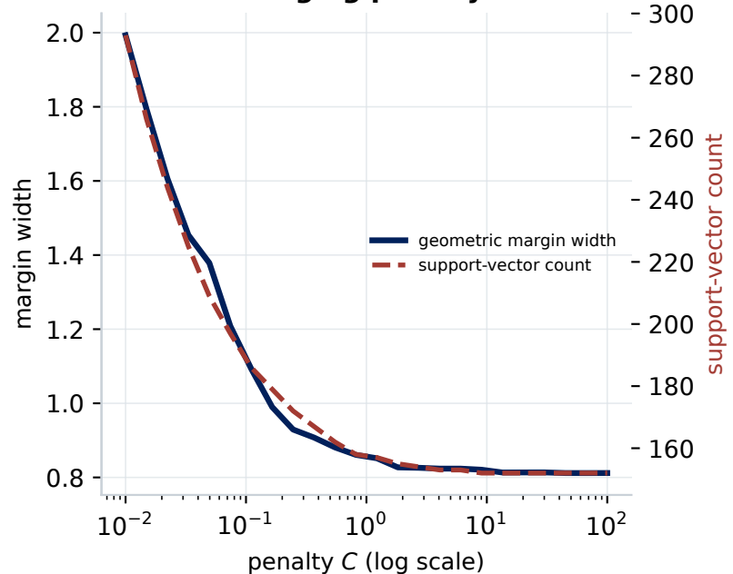
Changing penalty C
