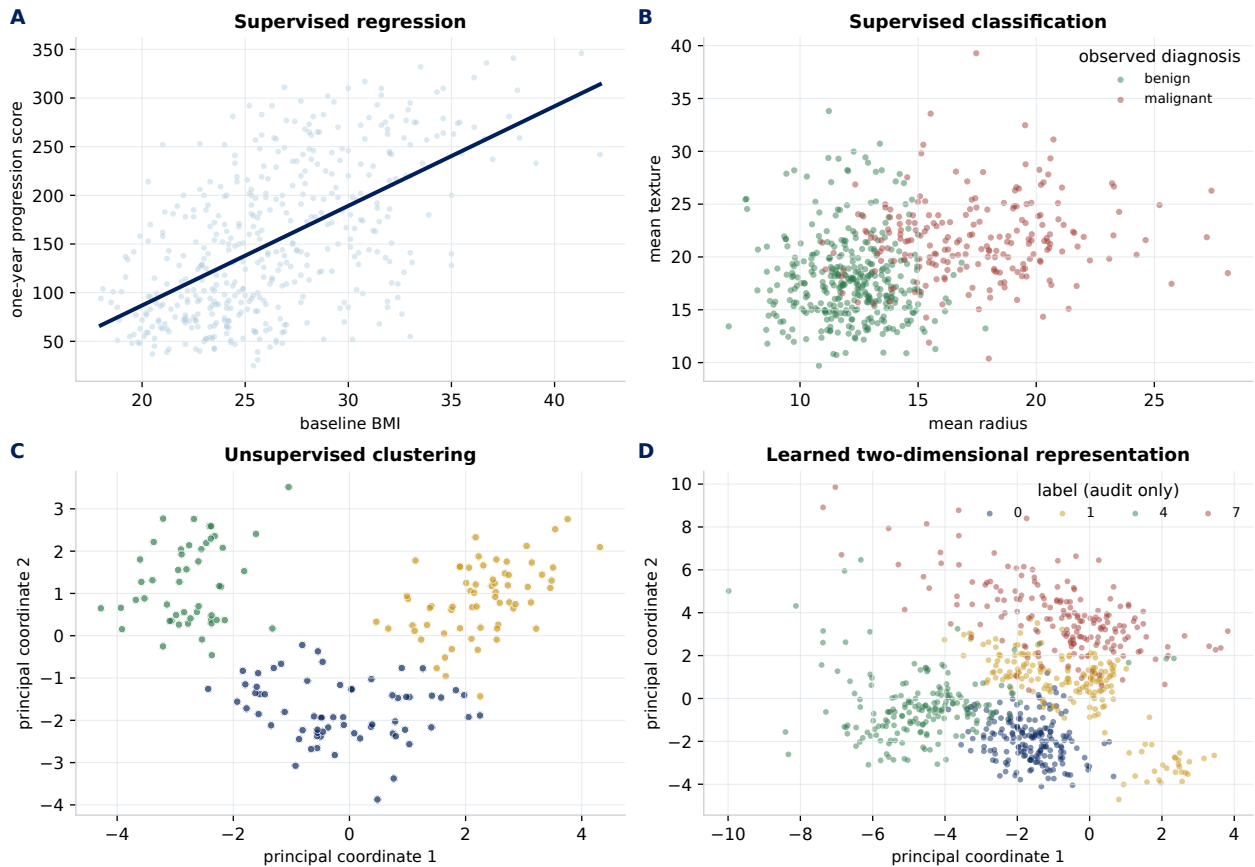
Figure 10.1: Four learning structures constructed from documented observations in the local course database. The plotting program queries SQLite, fits the displayed estimators, and writes this vector graphic. Regenerate it with uv run python textbook/figures/generate_part_ii_figures.py .
