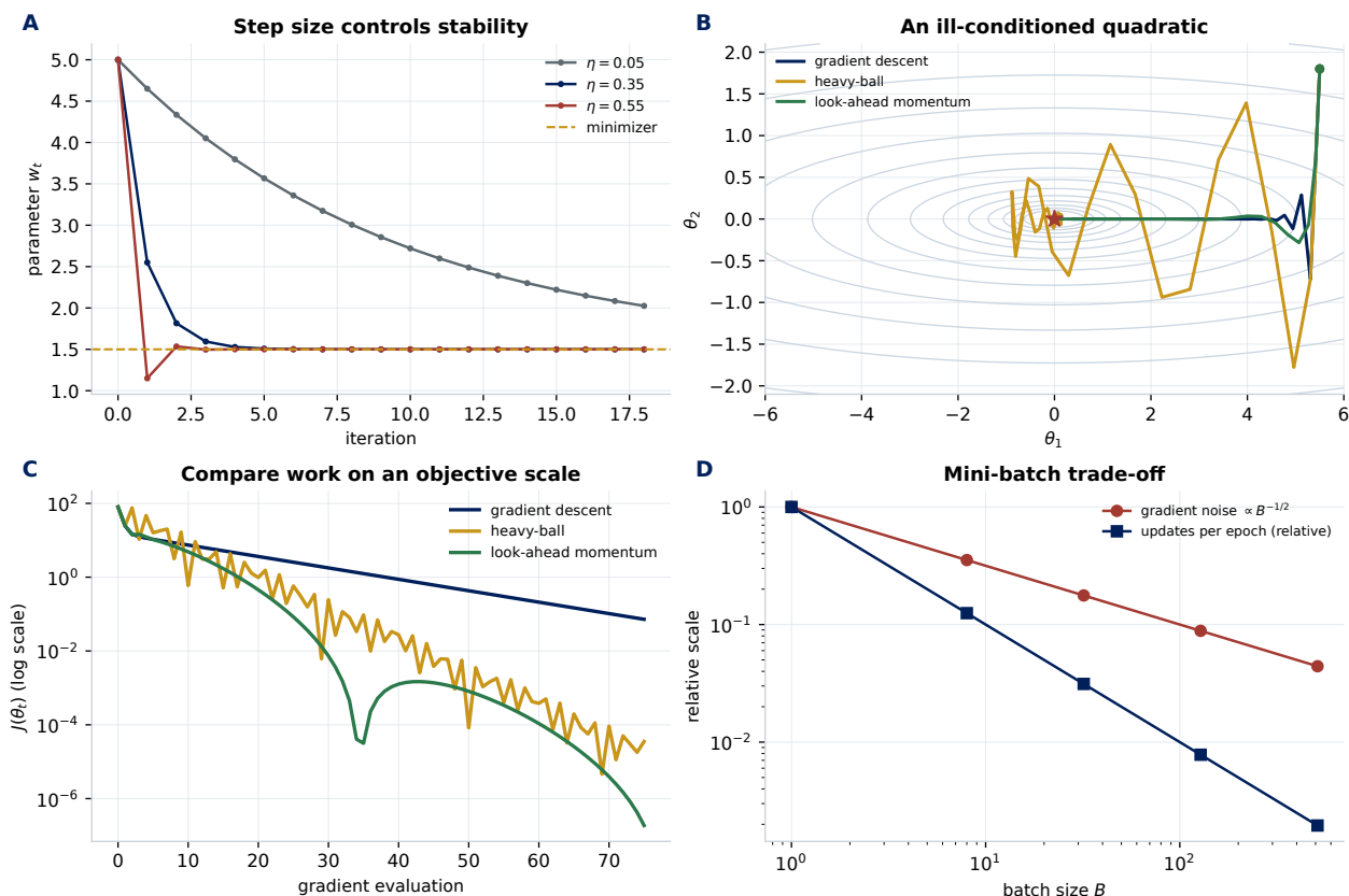
Figure 13.1: First-order optimization diagnostics generated from executable quadratic examples. Panel A isolates step-size stability; panels B and C compare paths and objective progress; panel D shows the idealized variance and update-frequency trade-off induced by batch size.
