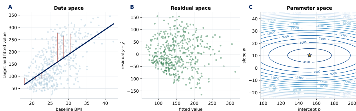
Figure 12.1: One-feature ordinary least squares on the course diabetes table. The coefficients are computed with numpy.linalg.lstsq ; the same predictions generate the data-space line, residual plot, and MSE contours.
