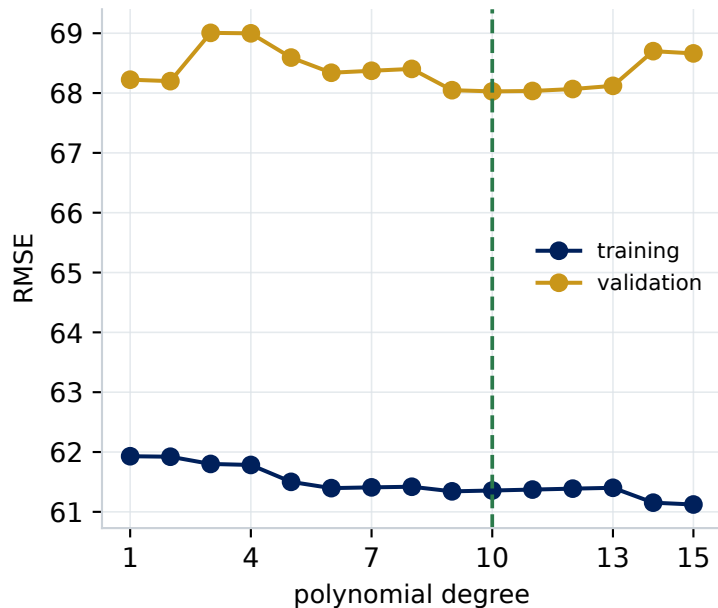
B Validation selects degree 10
