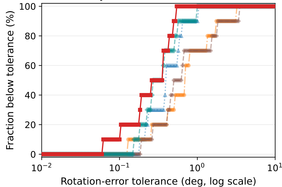
(a) Ordinary 3D, 80% outliers
