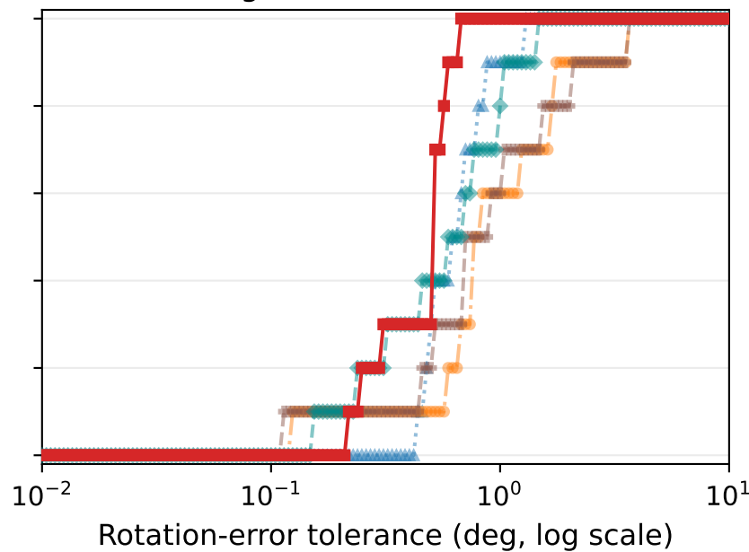
(b) Quasi-singular, 80% outliers
