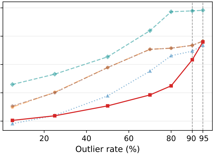
(c) Planar
