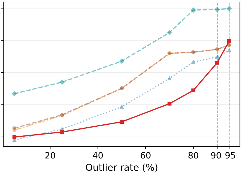
(b) Quasi-singular
