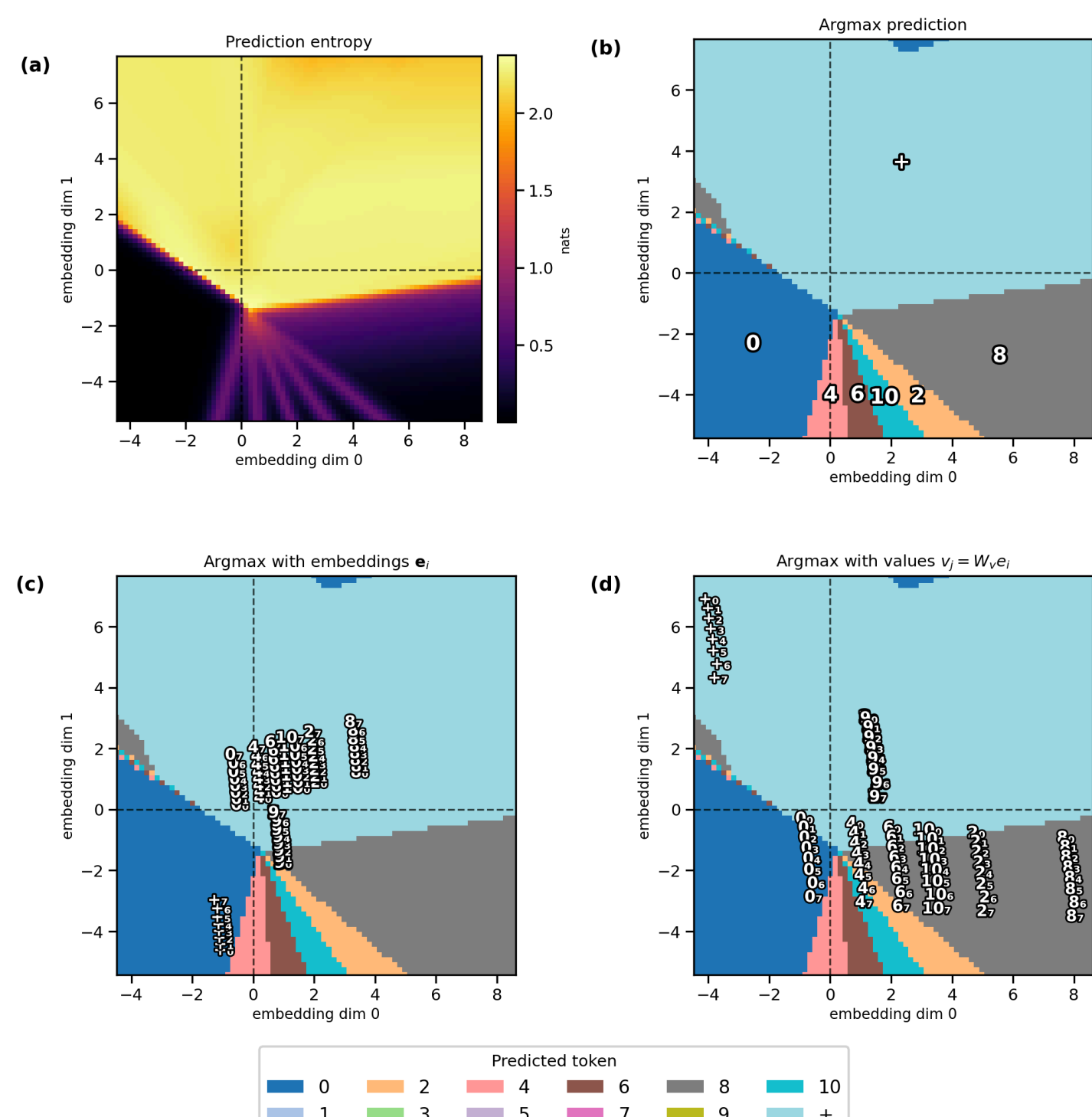
Figure 10. Output landscape summary (summary of Figure 9). (a) Entropy of the output distribution (hats); high in the indifference region (top half), near zero in even-number target zones (bottom half). (b) Argmax prediction map: color and annotation indicate which token has the highest predicted probability at each point. (c) Argmax map with combined embeddings e_i overlaid. (d) Argmax map with value-transformed vectors v_i overlaid.
