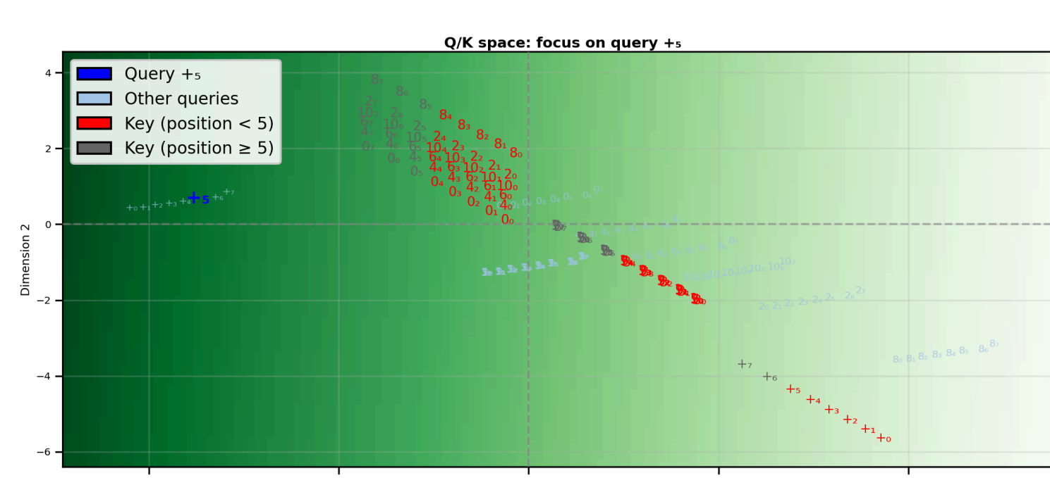
Figure 7. Query-key geometry in Q/K space. Top : joint query-key space (blue: queries; red: keys; labels show token and position). Bottom : Focus on the query +_5 (blue); background color indicates the dot product of the +_5 query with every point in space. Keys with position \geq 5 are grayed due to the causal mask.
