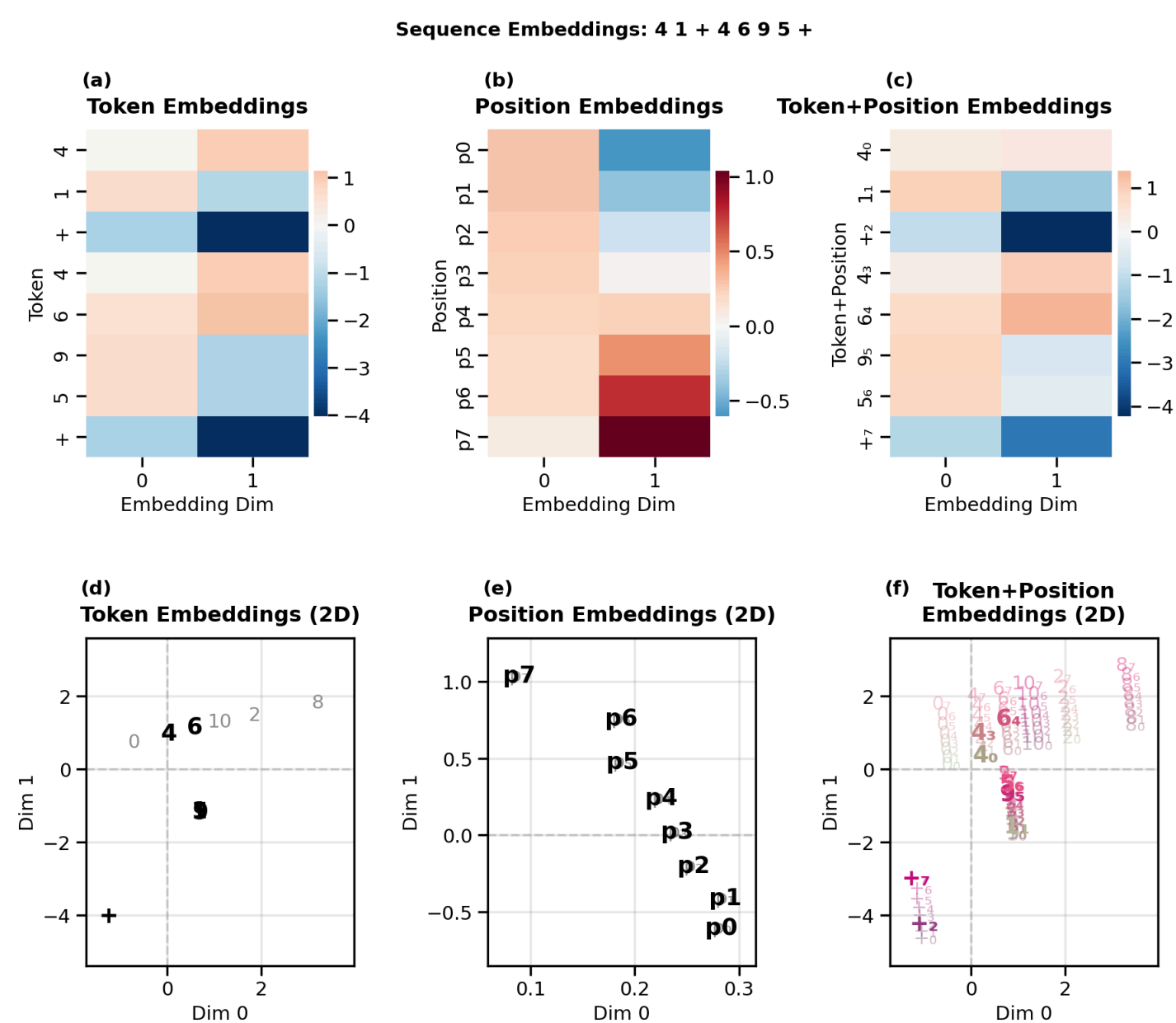
Figure 11. Embeddings for the demo sequence 4 1 + 4 6 9 5 +. a-c : Embedding heatmaps for tokens, positions and token+position. d-f : 2D scatter plot views of tokens, positions, and token+position embeddings, shown over a backdrop of all possible tokens, positions, and token+position embeddings (light gray).
