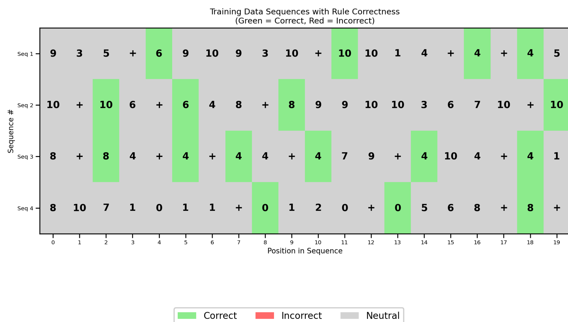
Figure 2. Sample training sequences with rule correctness (the most recent even number). Green: constrained position (immediately after +) with the correct next token (the most recent even number). Gray: unconstrained position (any token is valid).
