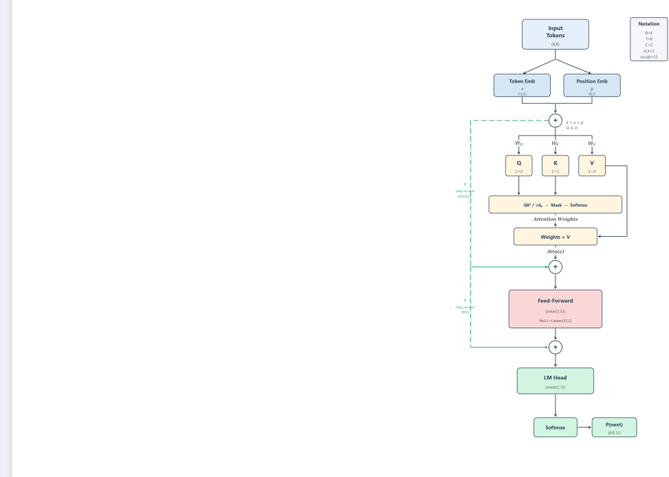
Figure 1. Architecture of the minimal transformer. Every component operates entirely in \mathbb{R}^2 .
