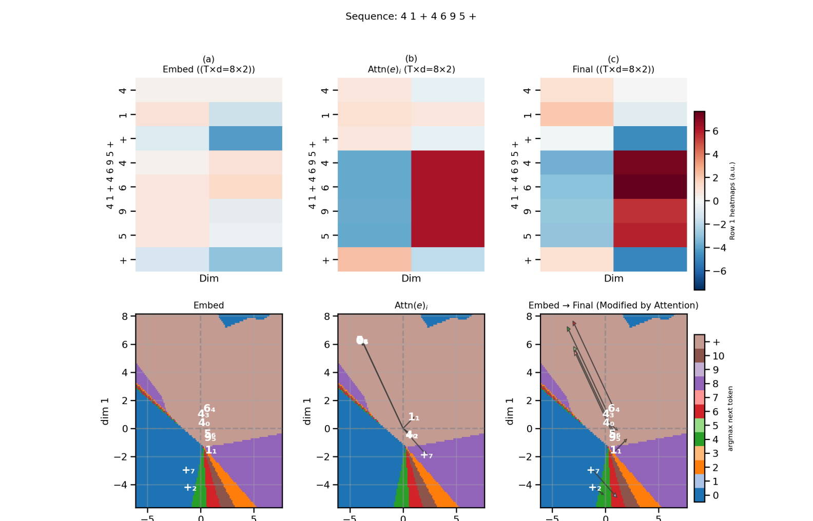
Figure 15. Predicting the next token by summing the input embeddings and attention vectors. (a) Top: Heatmaps illustrating the 2D values for the input embeddings (e) for each token in the test sequence. Bottom: Input embeddings in the 2D output space, where the background colors represent the most likely next-token prediction. (b) Top: The attention vectors (Attn(e)). Bottom: The attention weights shown as arrows from the origin. (c) Top: The sum of the input embeddings and the attention vectors ( z ) as heatmap. Bottom: Input embeddings (white annotations) are moved by the attention vectors (arrows) to the correct region for predicting the next token.
