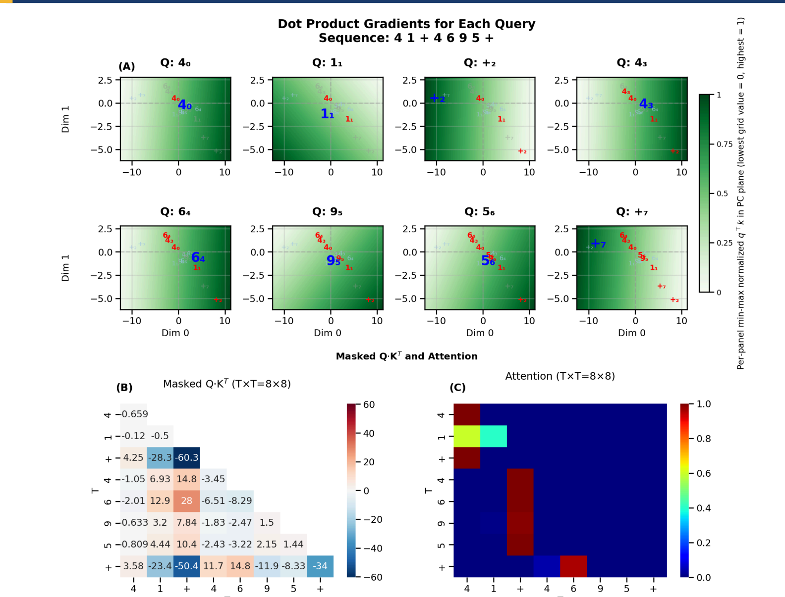
Figure 13. Attention computation for the demo sequence. (a) The background of each panel displays the dot product of a specific query (blue) in the test sequence with every point in space (green = high, white = low). The unmasked (red) and masked (gray) keys are overlaid on this space to show their dot products with the selected query. (b) The masked Q \cdot K^T matrix. (c) the attention matrix after normalization by \sqrt{d_k} and applying softmax.
