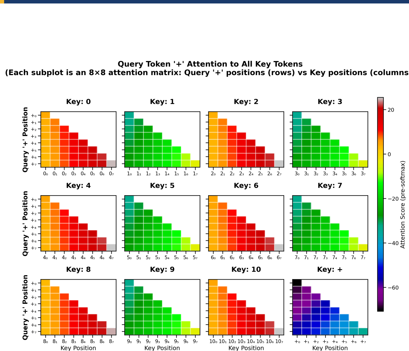
Figure 8. Pre-softmax query-key scores QK^T , restricted to + queries. Each subplot shows an 8 \times 8 matrix of dot products: + query positions (rows) vs. key positions (columns) for a particular key token.
