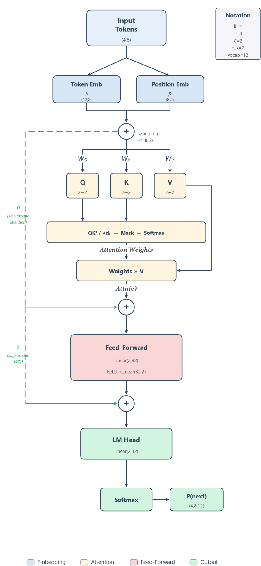
Figure 1. Architecture of the minimal transformer. Every component operates entirely in \mathbb{R}^2 .
