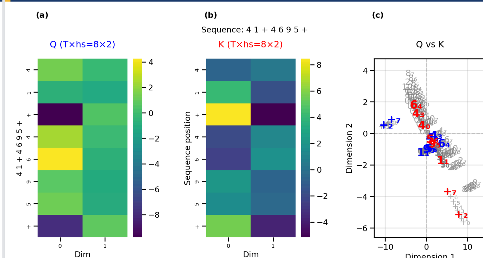
Figure 12. Q and K for the demo sequence. (a) Q heatmap. (b) K heatmap. (c) scatterplot of queries (blue), and keys (red) for tokens within our test sequence against a backdrop of all 96 possible queries and keys (gray).
