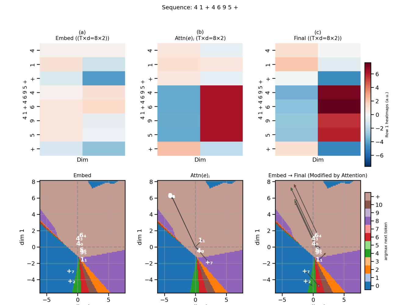
Figure 15. Predicting the next token by summing the input embeddings and attention vectors. (a) Top: Heatmaps illustrating the 2D values for the input embeddings (e) for each token in the test sequence. Bottom: Input embeddings in the 2D output space, where the background colors represent the most likely next-token prediction. (b) Top: The attention weights shown as arrows from the origin. Bottom: The attention weights shown as arrows from the origin. (c) Top: The sum of the input embeddings and the attention vectors (z) as heatmap. Bottom: Input embeddings (white annotations) are moved by the attention vectors (arrows) to the correct region for predicting the next token.
