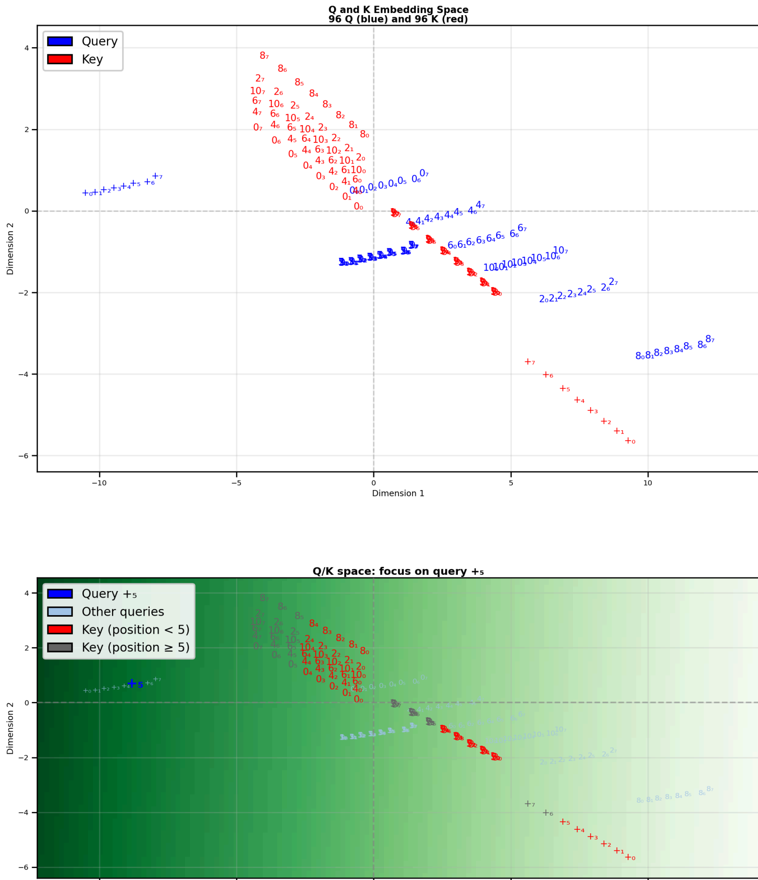
Figure 7. Query-key geometry in Q/K space. Top: joint query-key space (blue: queries; red: keys; labels show token and position). Bottom: Focus on the query +_5 (blue); background color indicates the dot product of the +_5 query with every point in space. Keys with position \geq 5 are grayed due to the causal mask.
