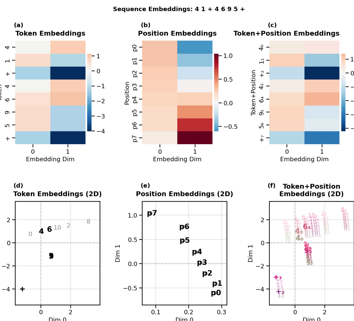
Figure 11. Embeddings for the demo sequence 4 1 + 4 6 9 5 +. a-c: Embedding heatmaps for tokens, positions and token+position. d-f: 2D scatter plot views of tokens, positions, and token+position combinations, shown over a backdrop of all possible tokens, positions, and token+position embeddings (light gray).
