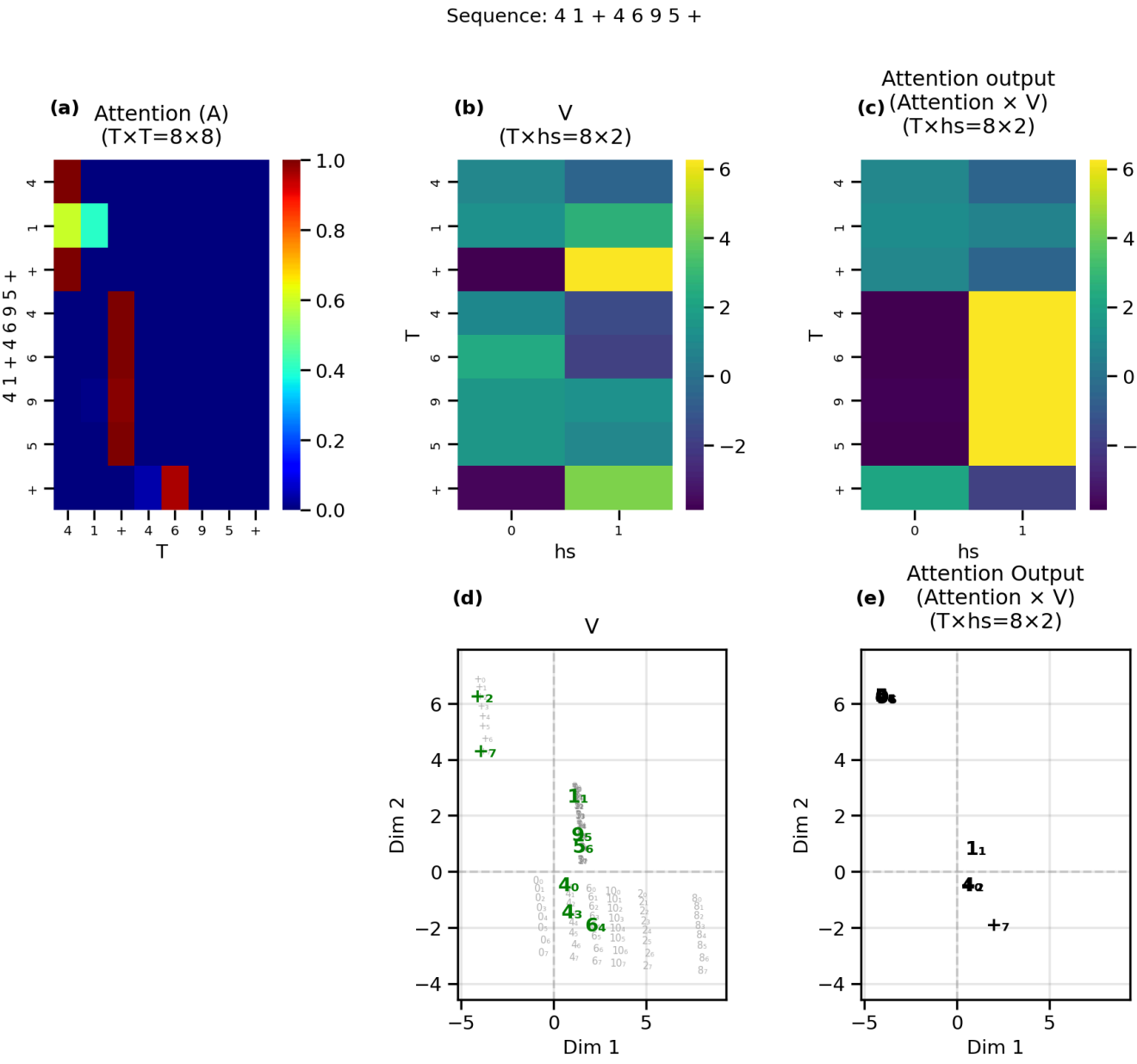
Figure 14. Values and attention output for the demo sequence. (a) Attention weight matrix as in Figure 13c. (b) Values for each digit shown as heatmaps. (c) Attention outputs shown as heatmaps. (d) Values shown as scatter plot. (e) Attention output shown as scatter plot.
