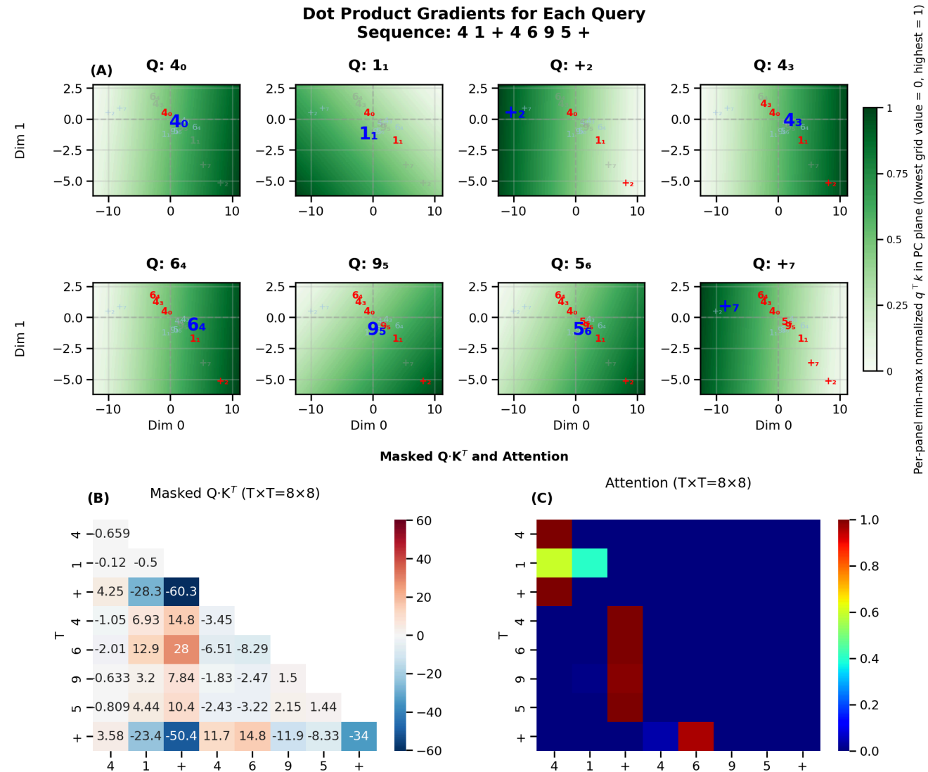
Figure 13. Attention computation for the demo sequence. (a) The background of each panel displays the dot product of a specific query (blue) in the test sequence with every point in space (green = high, white = low). The unmasked (red) and masked (gray) keys are overlaid on this space to show their dot products with the selected query. (b) The masked Q \cdot K^T matrix, (c) the attention matrix after normalization by \sqrt{d_k} and applying softmax.
