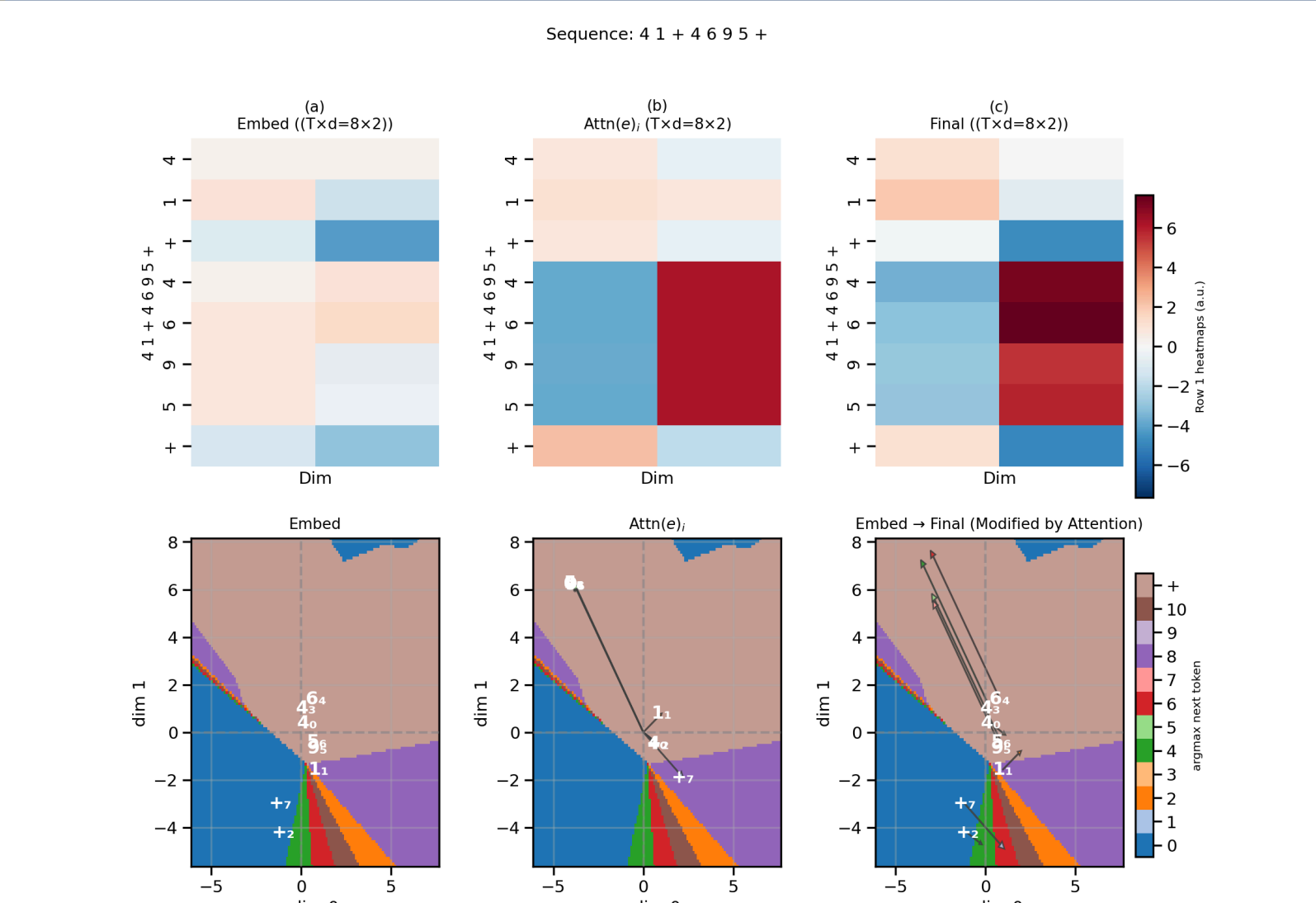
Figure 15. Predicting the next token by summing the input embeddings and attention vectors. (a) Top: Heatmaps illustrating the 2D values for the input embeddings (e) for each token in the test sequence. Bottom: Input embeddings in the 2D output space, where the background colors represent the most likely next-token prediction. (b) Top: The attention vectors (Attn(e)). Bottom: The attention weights shown as arrows from the origin. (c) Top: The sum of the input embeddings and the attention vectors (z) as heatmap. Bottom: Input embeddings (white annotations) are moved by the attention vectors (arrows) to the correct region for predicting the next token.
