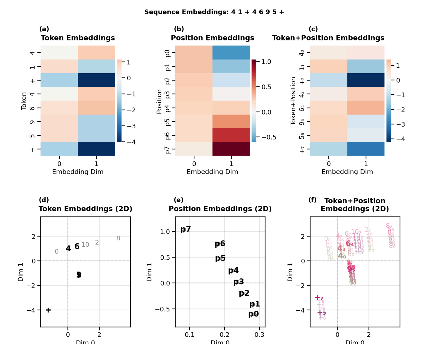
Figure 11. Embeddings for the demo sequence 4 1 + 4 6 9 5 +. a-c: Embedding heatmaps for tokens, positions and token+position. d-f: 2D scatter plot views of tokens, positions, and token+position combinations, shown over a backdrop of all possible tokens, positions, and token+position embeddings (light gray).
