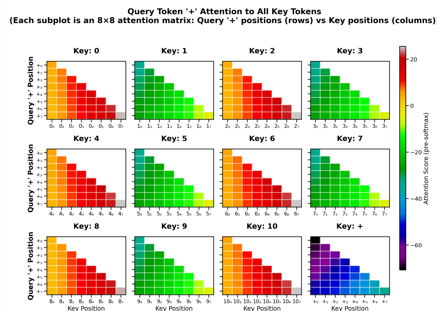
Figure 8. Pre-softmax query-key scores QK^T , restricted to + queries. Each subplot shows an 8 \times 8 matrix of dot products: + query positions (rows) vs. key positions (columns) for a particular key token.
