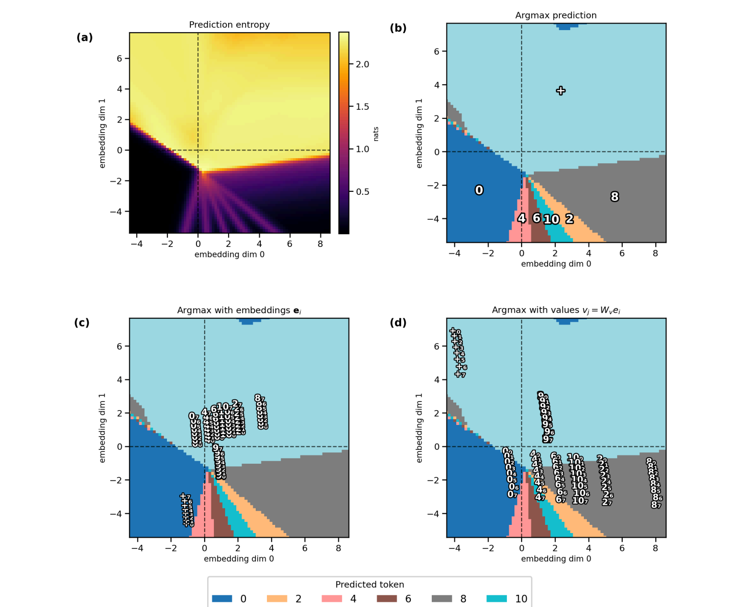
Figure 10. Output landscape summary (summary of Figure 9). (a) Entropy of the output distribution (nats); high in the indifference region (top half), near zero in even-number target zones (bottom half). (b) Argmax prediction map: color and annotation indicate which token has the highest predicted probability at each point. (c) Argmax map with combined embeddings e_i overlaid. (d) Argmax map with value-transformed vectors v_i overlaid.
