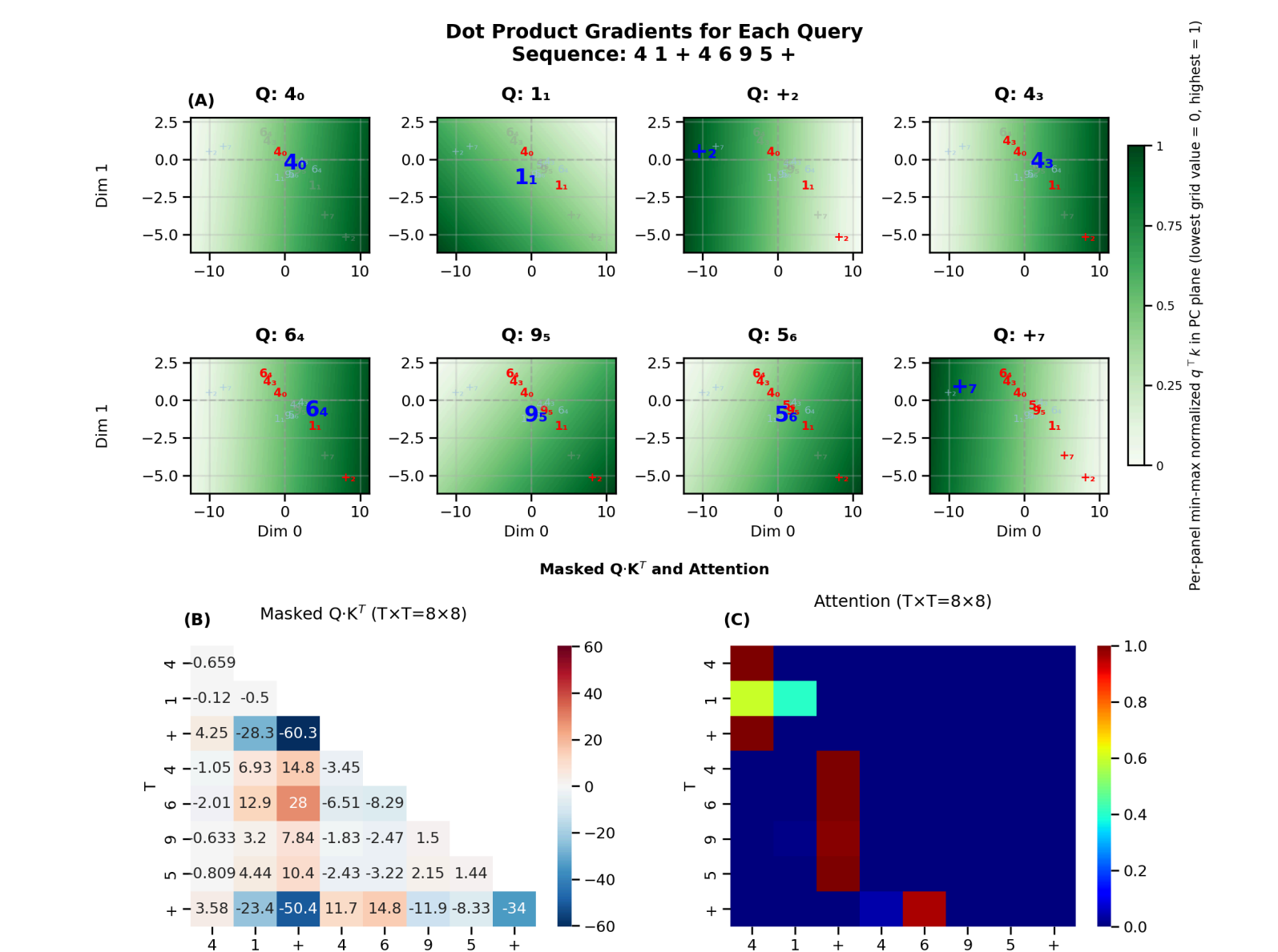
Figure 13. Attention computation for the demo sequence. (a) The background of each panel displays the dot product of a specific query (blue) in the test sequence with every point in space (green = high, white = low). The unmasked (red) and masked (gray) keys are overlaid on this space to show their dot products with the selected query. (b) The masked Q \cdot K^T matrix, (c) the attention matrix after normalization by \sqrt{d_k} and applying softmax.
