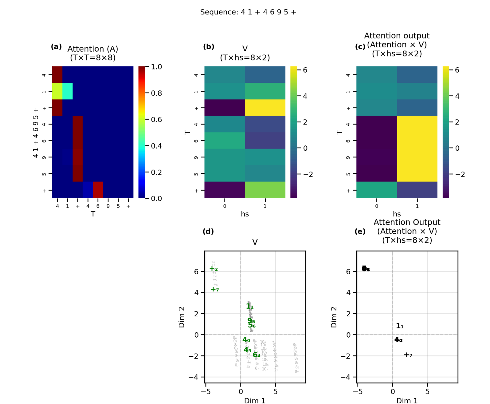
Figure 14. Values and attention output for the demo sequence. (a) Attention weight matrix as in Figure 13c, (b) Values for each digit shown as heatmaps. (c) Attention outputs shown as heatmaps. (d) Values shown as scatter plot. (e) Attention output shown as scatter plot.
