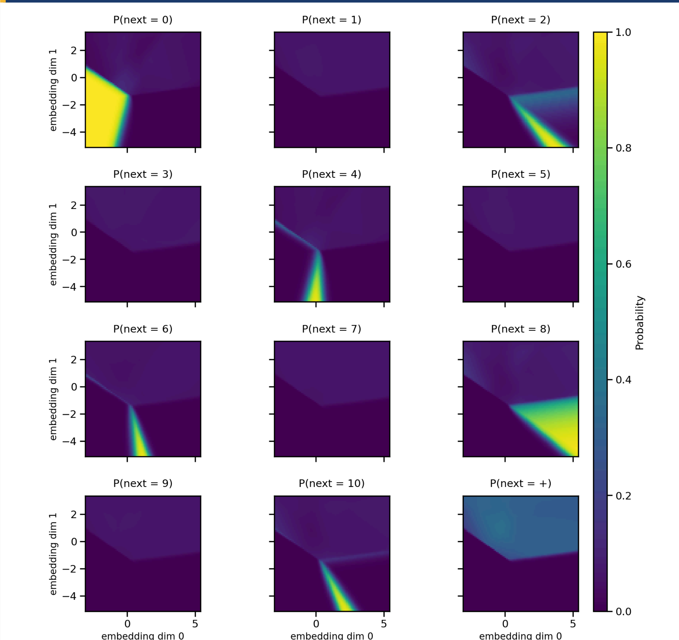
Figure 9. Output probability landscape (per-unit view). Each subplot shows the softmax probability P(\text{next} = \text{token}) over the 2D plane for one output token (digits 0-10 and the + operator).
