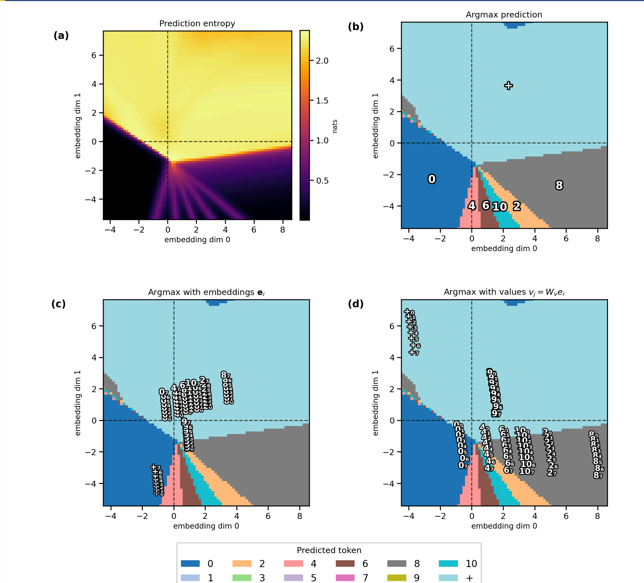
Figure 10. Output landscape summary (summary of Figure 9). (a) Entropy of the output distribution (nats); high in the indifference region (top half), near zero in even-number target zones (bottom half). (b) Argmax prediction map: color and annotation indicate which token... has the highest predicted probability at each point. (c) Argmax map with combined embeddings e_i overlaid. (d) Argmax map with value-transformed vectors v_i overlaid.
