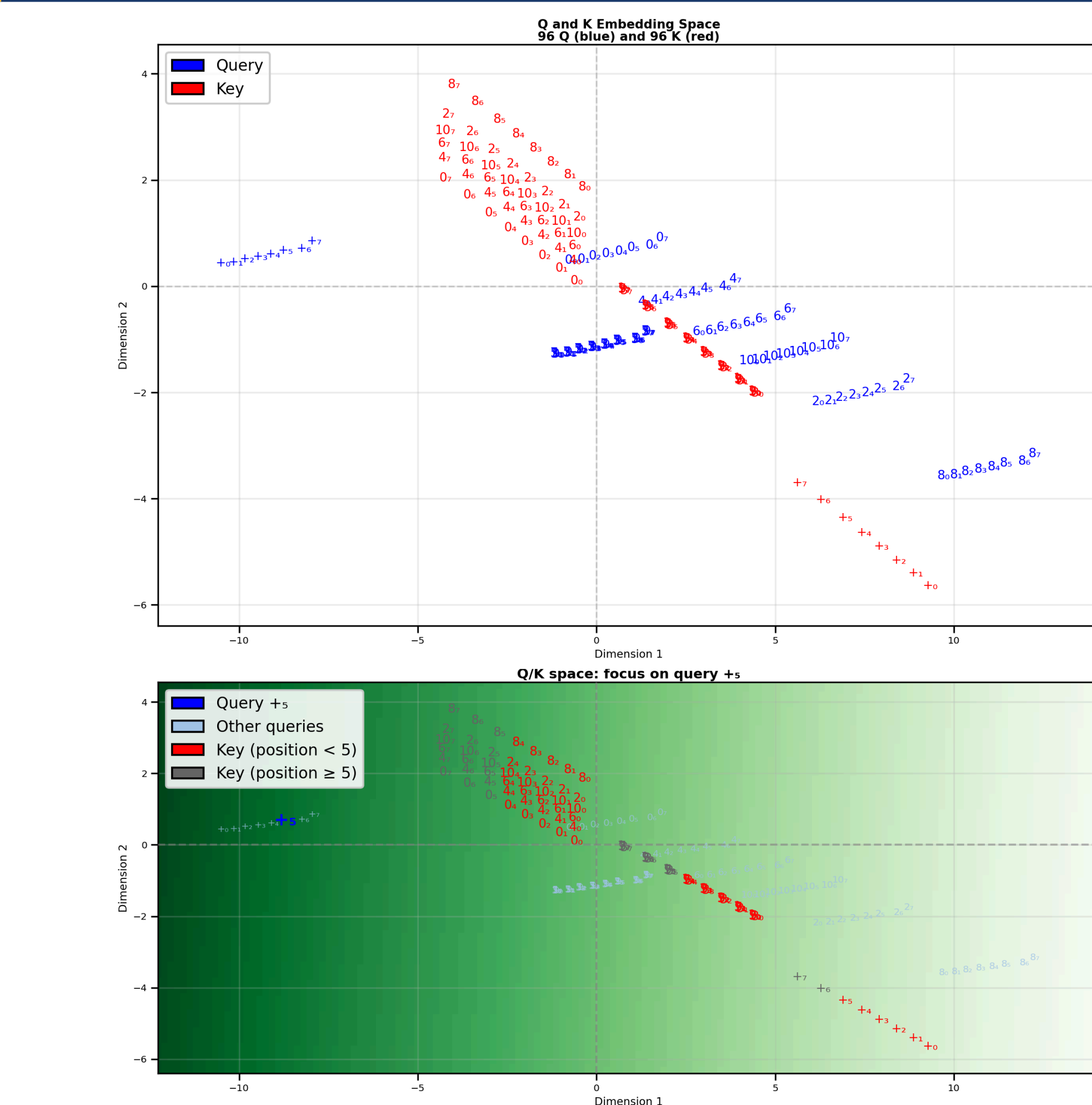
Figure 7. Query-key geometry in Q/K space. Top: joint query-key space (blue: queries; red: keys; labels show token and position). Bottom: Focus on the query +_5 (blue); background color indicates the dot product of the +_5 query with every point in space. Keys with position \geq 5 are grayed due to the causal mask.
