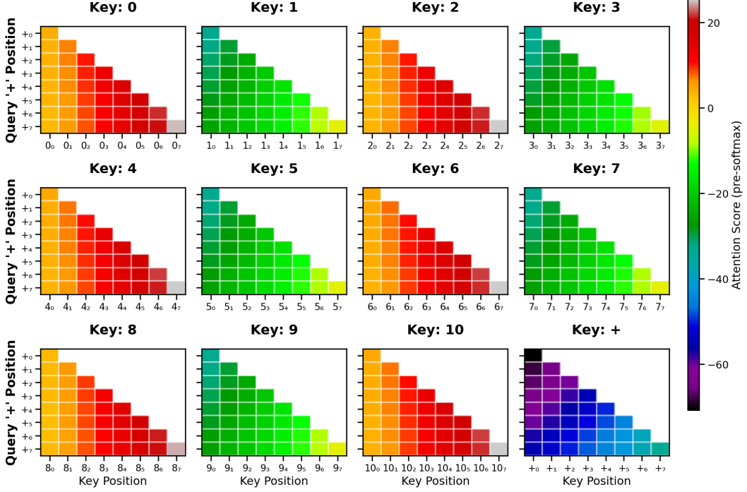
Figure 8. Pre-softmax query-key scores QK^\top , restricted to + queries. Each subplot shows an 8 \times 8 matrix of dot products: + query positions (rows) vs. key positions (columns) for a particular key token.
