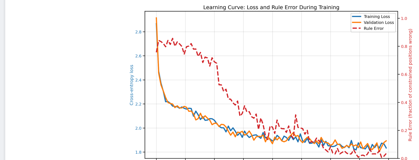
Figure 3. Training dynamics over 20,000 steps. Left axis: cross-entropy loss. Right axis: rule error — the fraction of constrained positions (tokens immediately following +) where the model's top predicted token is not the target (the most recent even number). Rule error near 90% is chance level; near 0% indicates the rule is learned.
