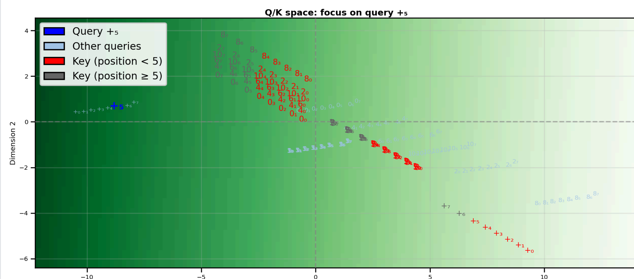
Figure 7. Query-key geometry in Q/K space. Top: joint query-key space (blue: queries; red: keys; labels show token and position). Bottom: Focus on the query +_5 (blue); background color indicates the dot product of the +_5 query with every point in space. Keys with position \ge 5 are grayed due to the causal mask.
