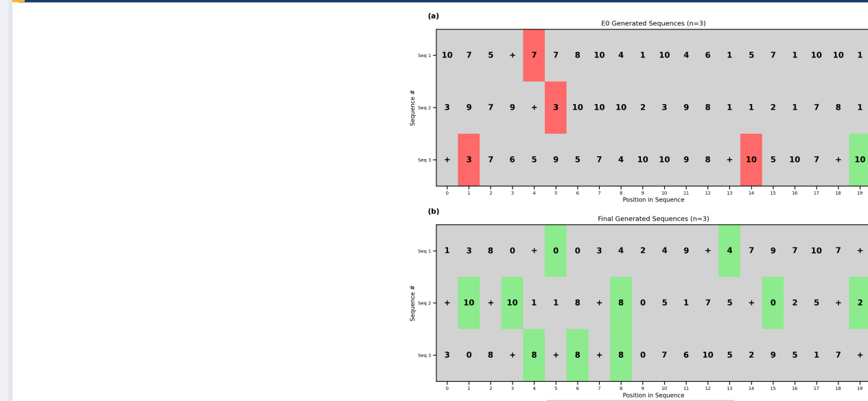
Figure 4. Model-generated sequences at initialization (top) vs. after training (bottom). Green = correct at constrained positions (after +), red = wrong at constrained positions, gray = unconstrained. Top: at step 0, constrained positions are mostly red (random predictions). Bottom: after training, constrained positions are mostly green (correct "last even" outputs).
