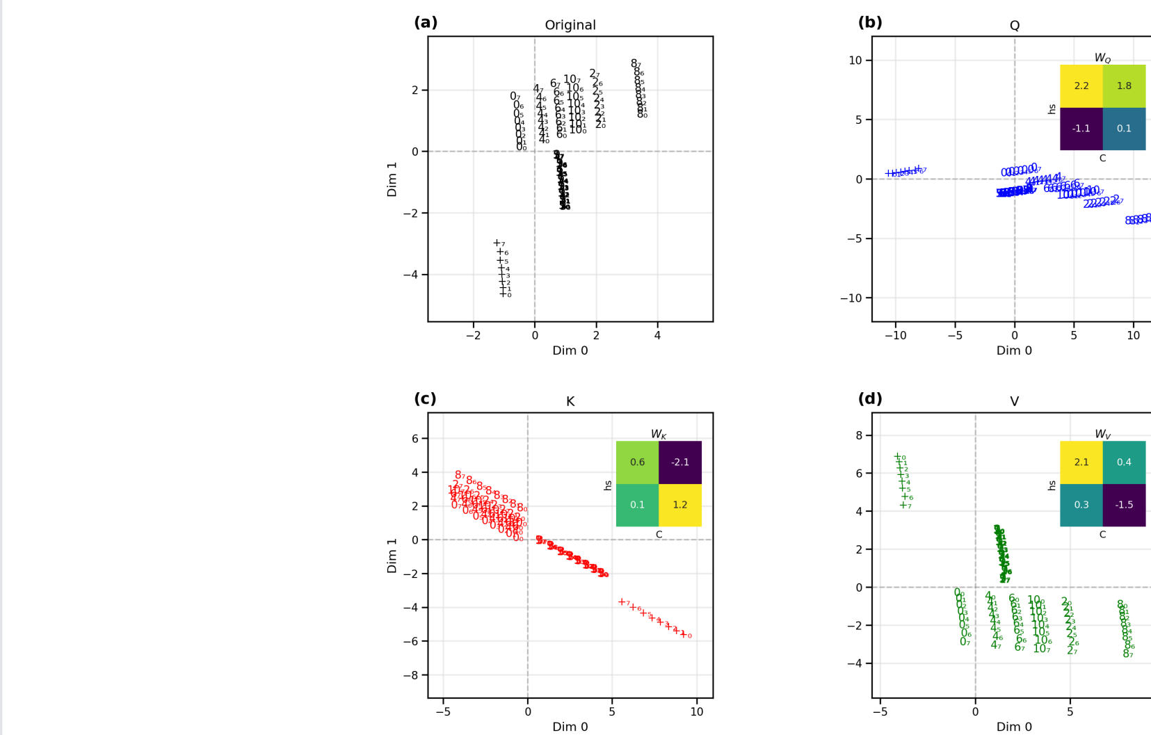
Figure 6. QKV projections. (a) Original combined token+position embeddings (as in Figure 5e). (b) Query-space (blue), with W_Q inset. (c) Key-space (red), with W_K inset. (d) Value-space (green), with W_V inset. All 96 token+position points in each panel.
