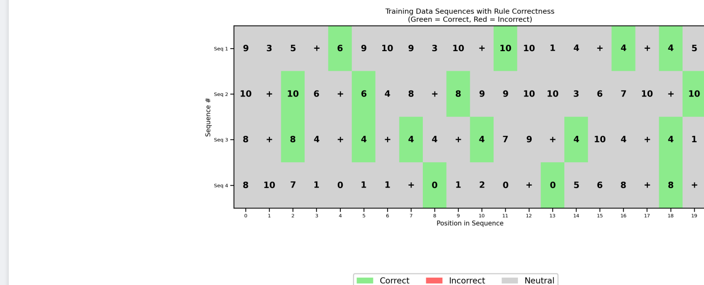
Figure 2. Sample training sequences as heatmaps. Green: constrained position (immediately after +) with the correct next token (the most recent even number). Gray: unconstrained position (any token is valid).
