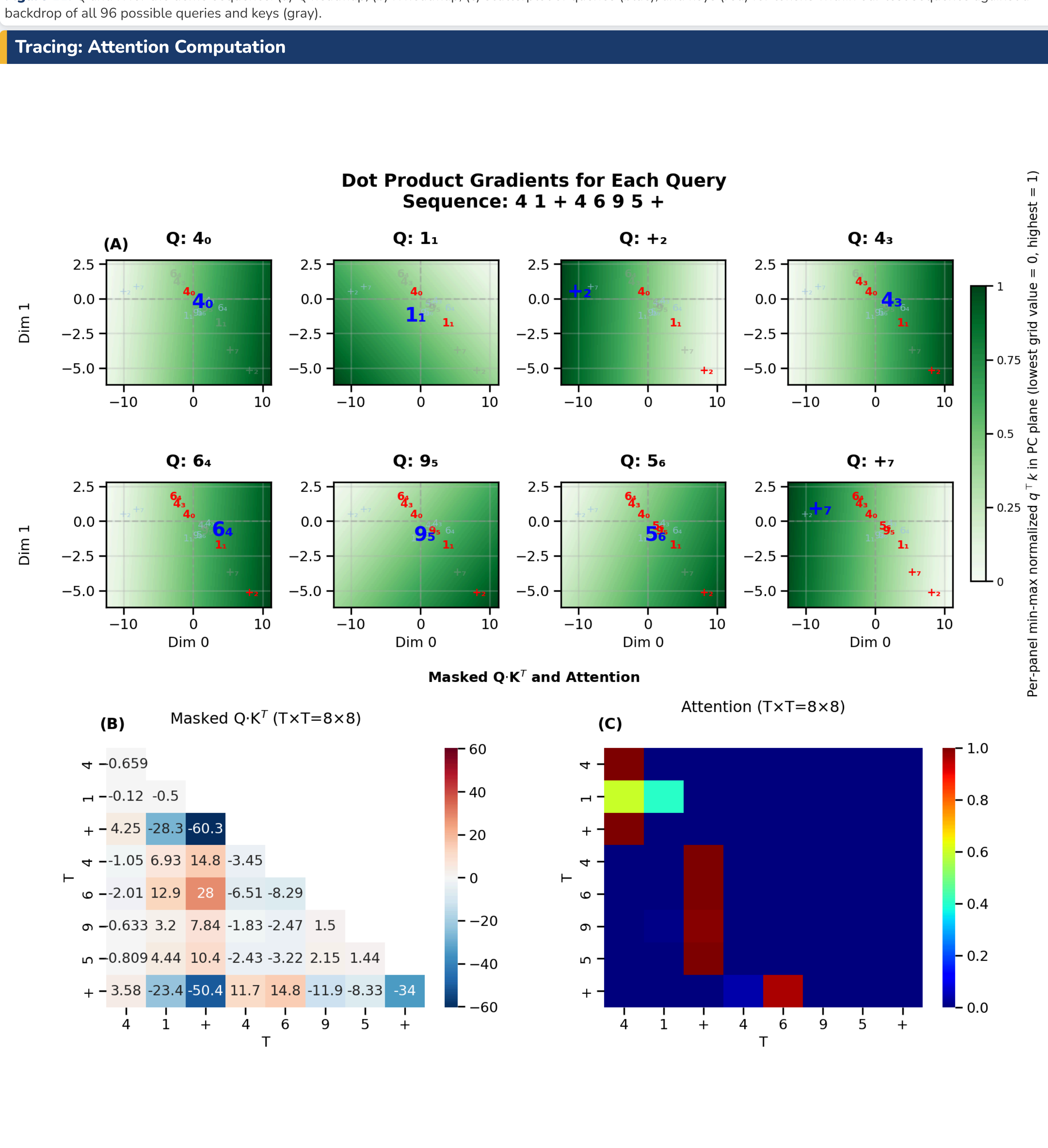
Figure 13. Attention computation for the demo sequence. (a) The background of each panel displays the dot product of a specific query (blue) in the test sequence with every point in space (green = high, white = low). The unmasked (red) and masked (gray) keys are overlaid on this space to show their dot products with the selected query. (b) The masked Q \cdot K^T matrix. (c) The attention matrix after normalization by \sqrt{d_k} and applying softmax.
