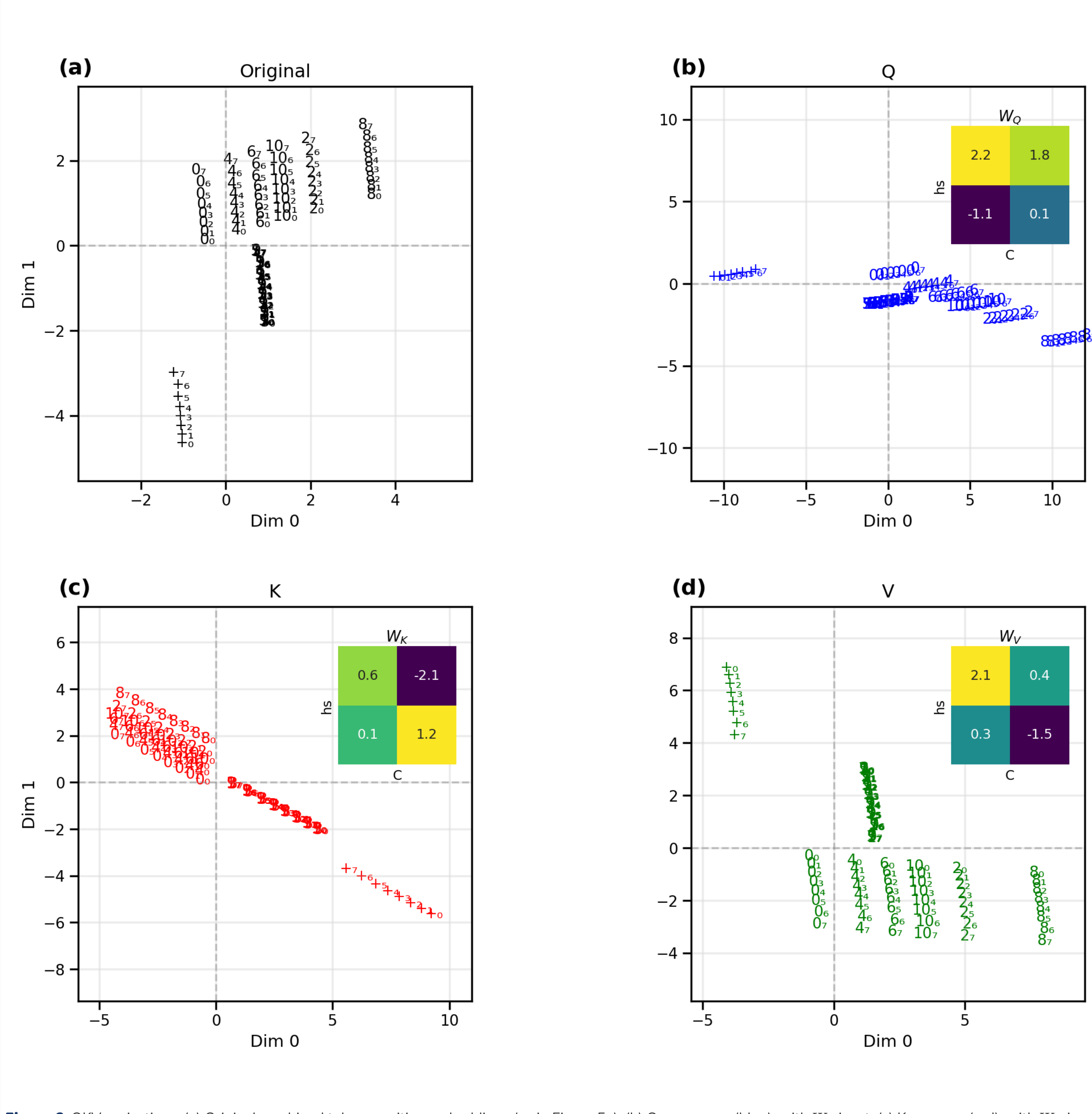
Figure 6. QKV projections. (a) Original combined token+position embeddings (as in Figure 5e). (b) Query-space (blue), with W_Q inset. (c) Key-space (red), with W_K inset. (d) Value-space (green), with W_V inset. All 96 token+position points in each panel.
