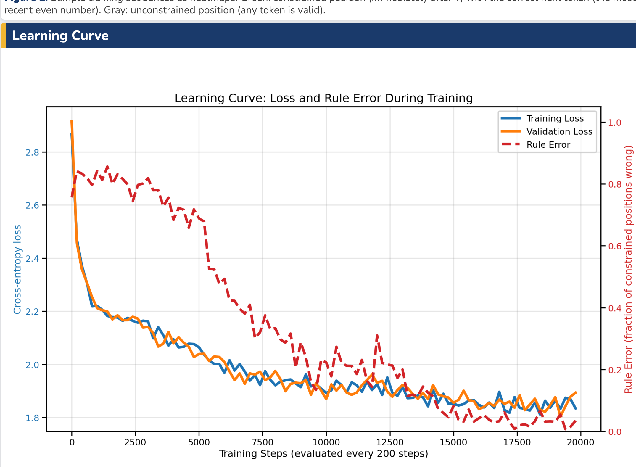
Figure 3. Training dynamics over 20,000 steps. Left axis: cross-entropy loss. Right axis: rule error — the fraction of constrained positions (tokens immediately following +) where the model's top predicted token is not the target (the most recent even number). Rule error near 90% is chance level; near 0% indicates the rule is learned.
