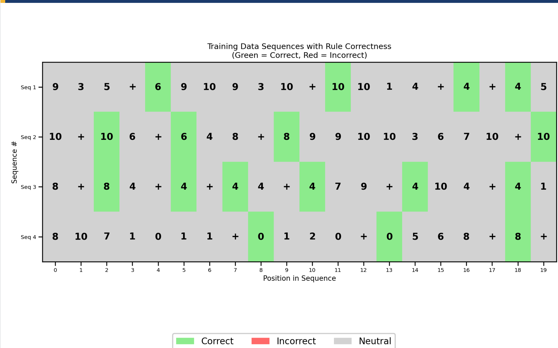
Figure 2. Sample training sequences as heatmaps. Green: constrained position (immediately after +) with the correct next token (the most recent even number). Gray: unconstrained position (any token is valid).
