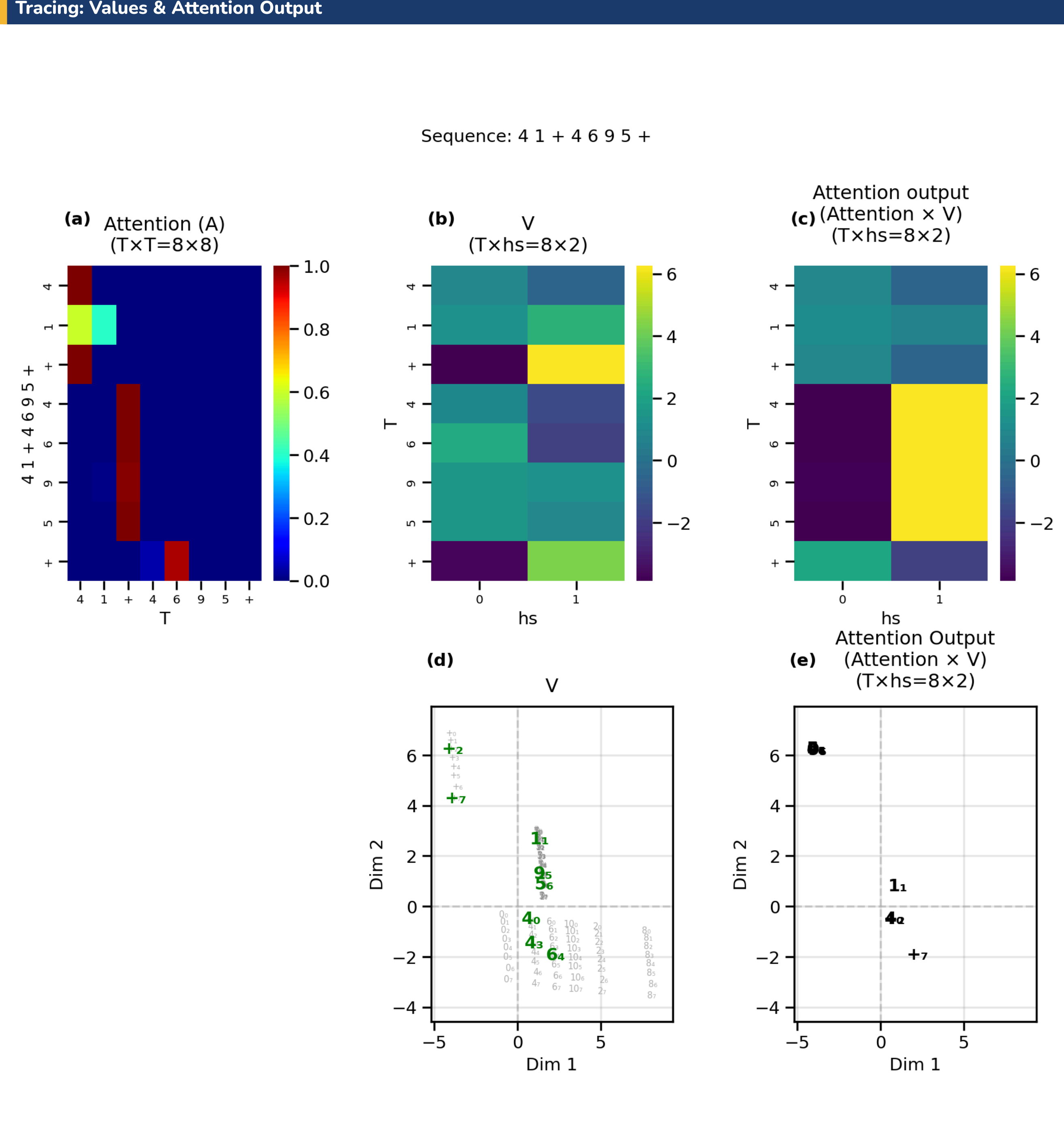
Figure 14. Values and attention output for the demo sequence. (a) Attention weight matrix as in Figure 13c. (b) Values for each digit shown as heatmaps. (c) Attention outputs shown as heatmaps. (d) Values shown as scatter plot. (e) Attention output shown as scatter plot.
