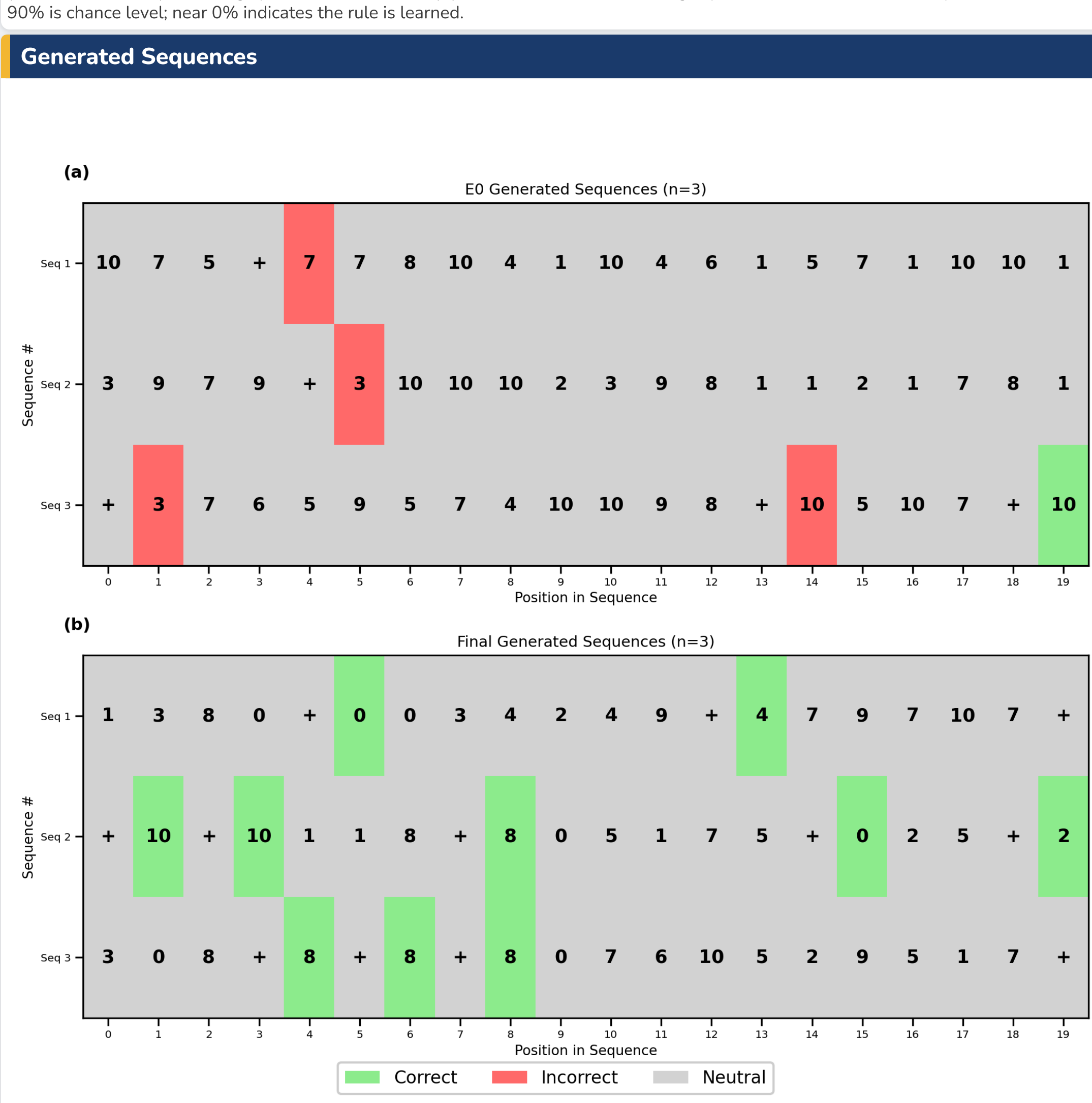
Figure 4. Model-generated sequences at initialization (top) vs. after training (bottom). Green = correct at constrained positions (after +), red = wrong at constrained positions, gray = unconstrained. Top: at step 0, constrained positions are mostly red (random predictions). Bottom: after training, constrained positions are mostly green (correct "last even" outputs).
