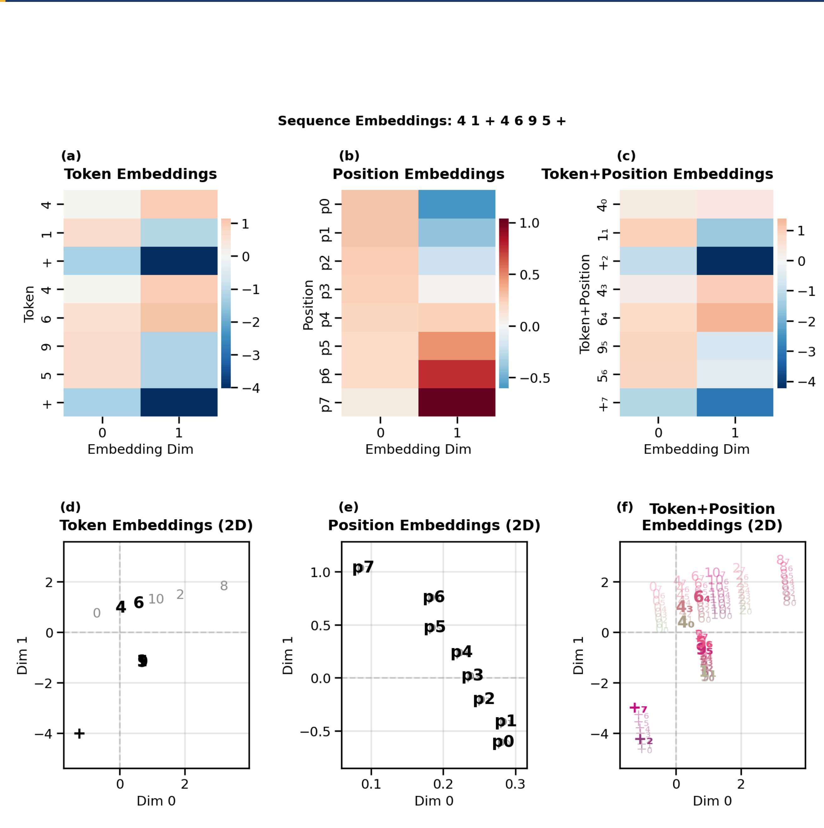
Figure 11. Embeddings for the demo sequence 4 1 + 4 6 9 5 +. a-c: Embedding heatmaps for tokens, positions and token+position. d-f: 2D scatter plot views of tokens, positions, and token+position combinations, shown over a backdrop of all possible tokens, positions, and token+position embeddings (light gray).
