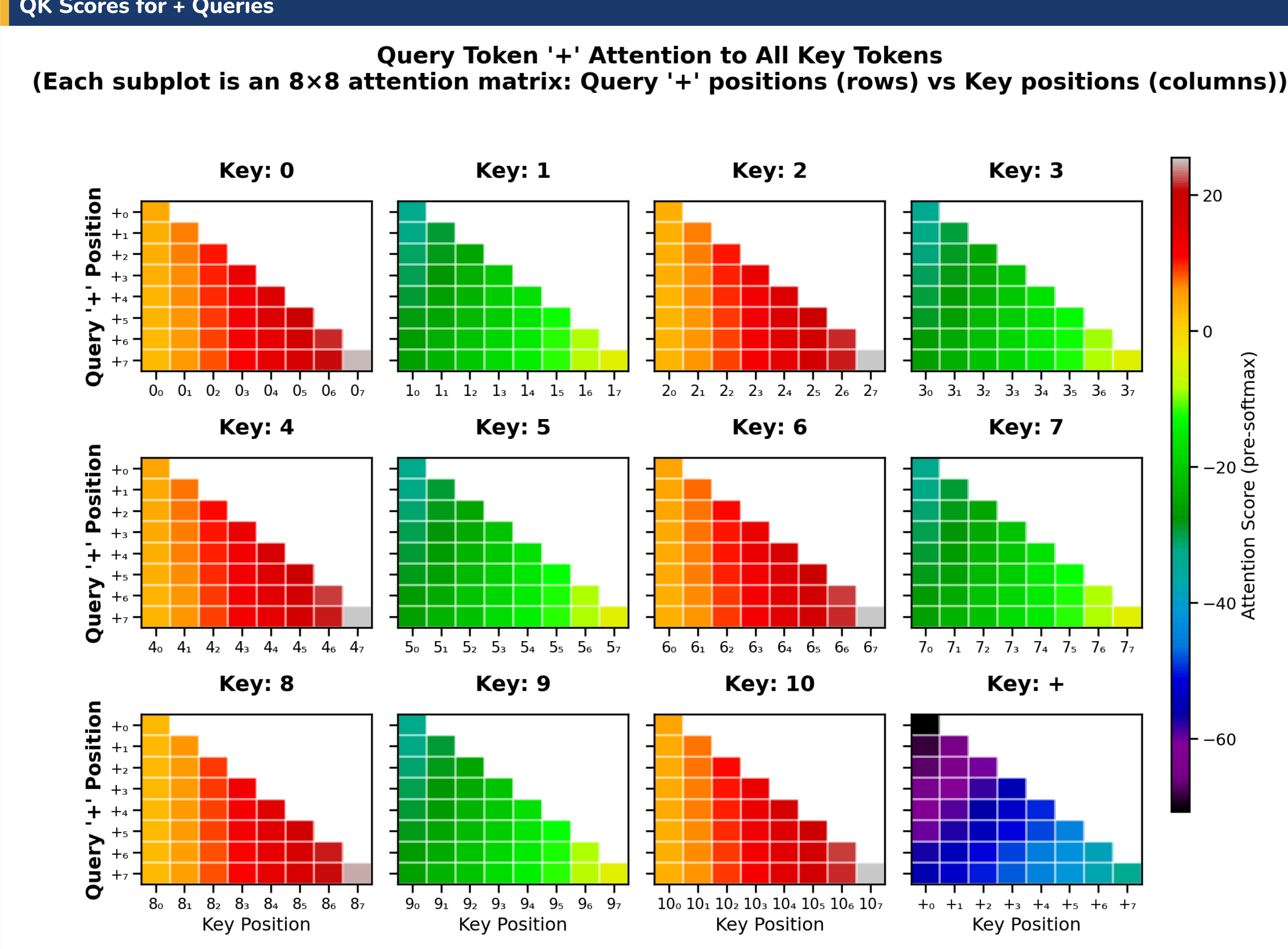
Figure 8. Pre-sorted query-key scores QK^T , restricted to + queries. Each subplot shows an 8x8 matrix of dot products: + query positions (rows) vs. key positions (columns) for a particular key token.
