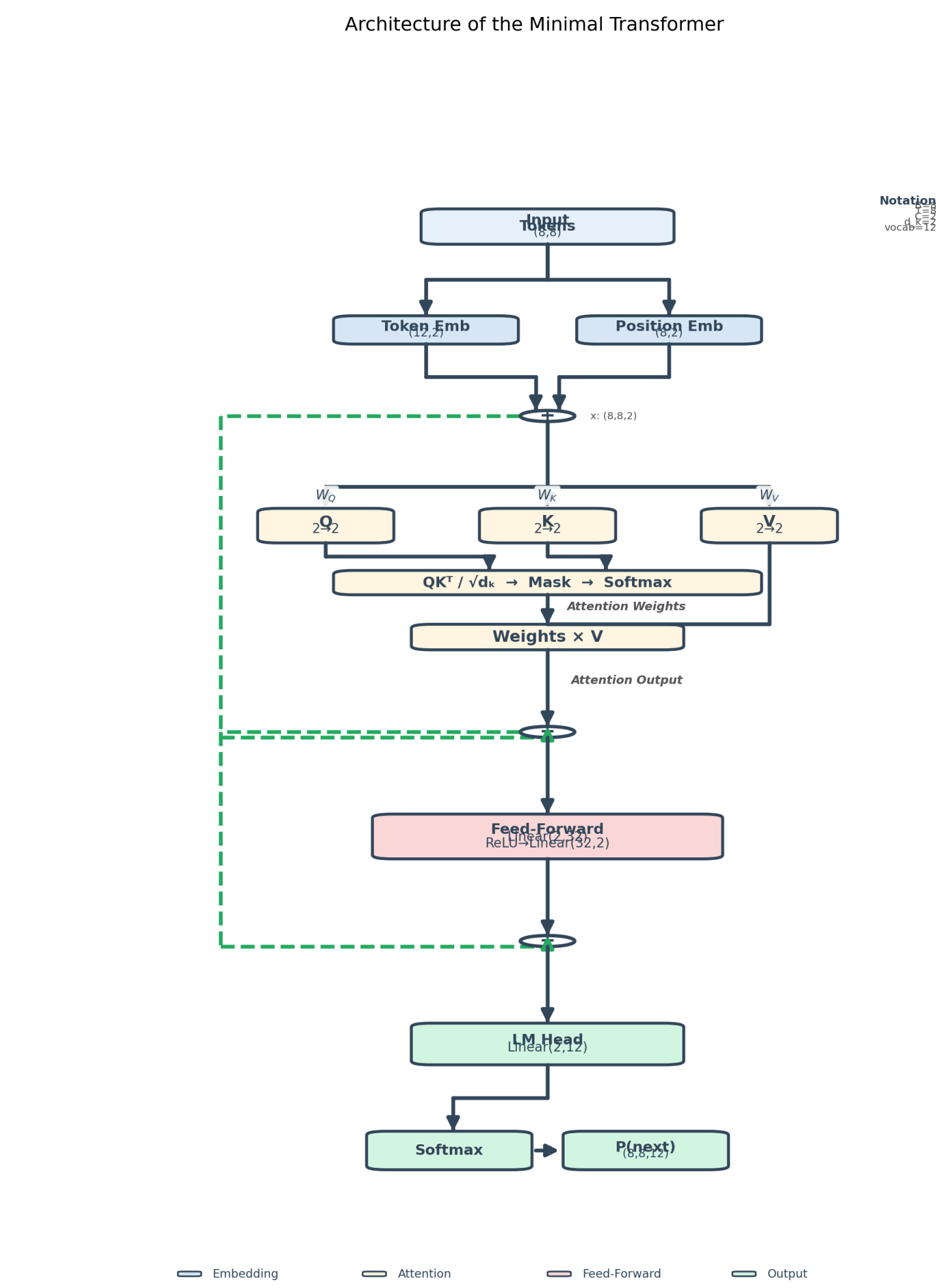
Figure 1. Architecture of the minimal transformer. Every component operates entirely in \mathbb{R}^2 .
