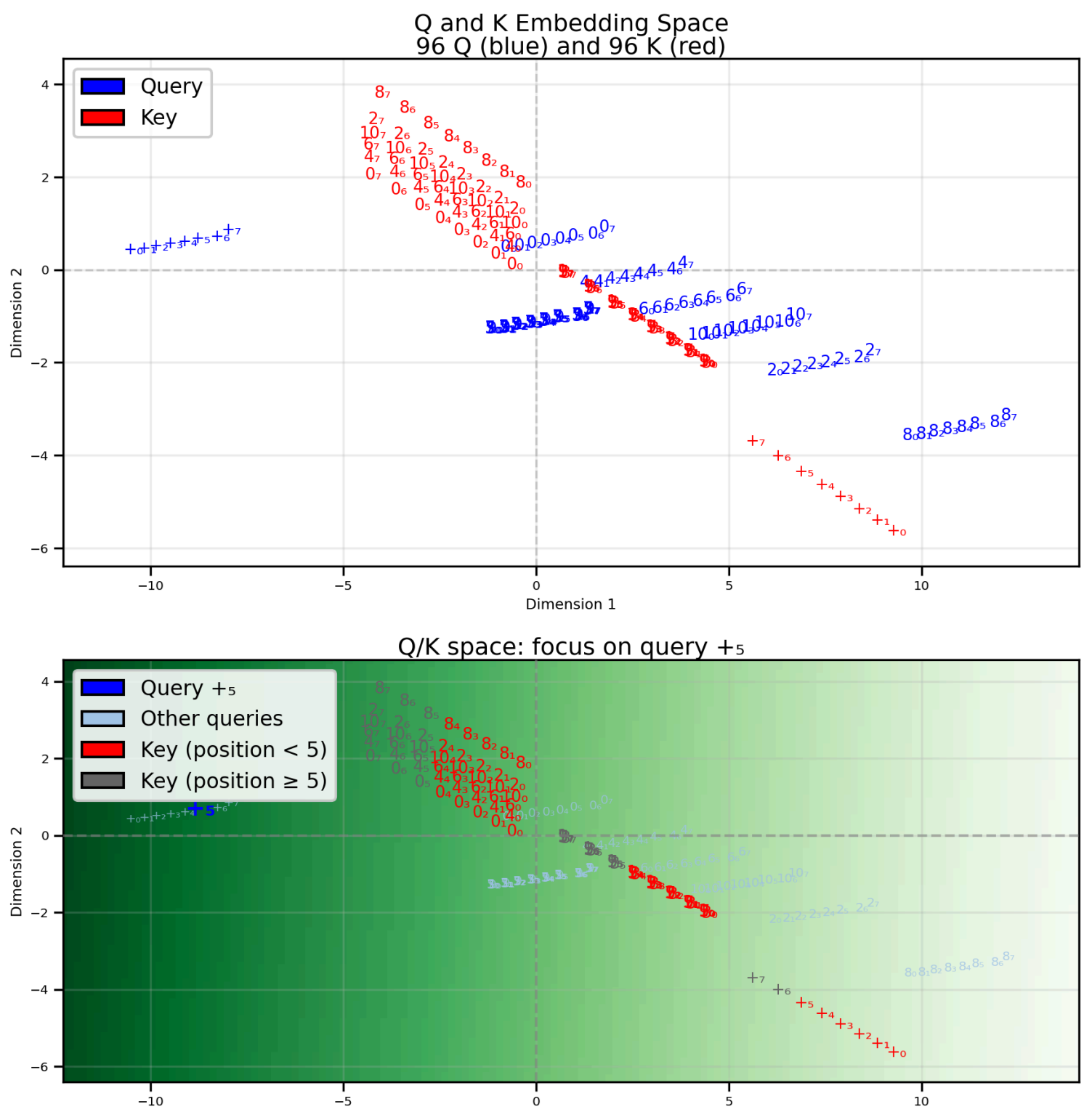
Figure 7. Query-key geometry in Q/K space. Top : joint query-key space (blue: queries; red: keys; labels show token and position). Bottom : Focus on the query +_5 (blue); background color indicates the dot product of the +_5 query with every point in space. Keys with position \geq 5 are grayed due to the causal mask.
