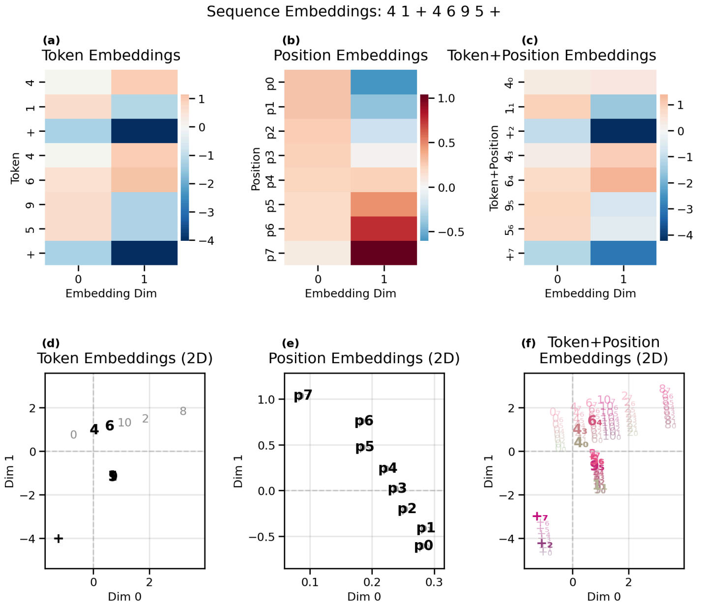
Figure 11. Embeddings for the demo sequence 4 1 + 4 6 9 5 +. a-c : Embedding heatmaps for tokens, positions and token+position. d-f : 2D scatter plot views of tokens, positions, and token+position combinations, shown over a backdrop of all possible tokens, positions, and token+position embeddings (light gray).
