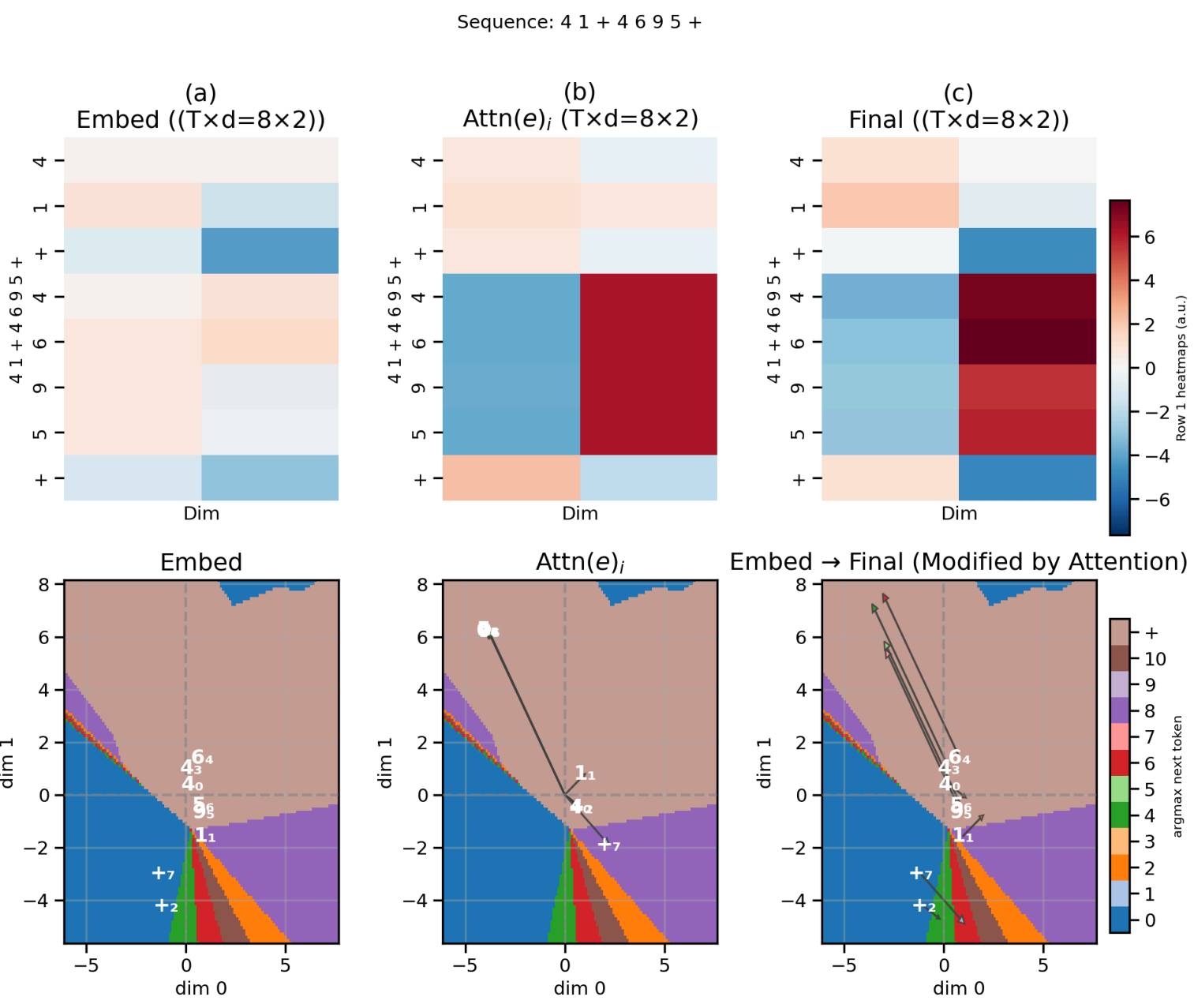
Figure 15. Predicting the next token by summing the input embeddings and attention vectors. (a) Top: Heatmaps illustrating the 2D values for the input embeddings (e) for each token in the test sequence. Bottom: Input embeddings in the 2D output space, where the background colors represent the most likely next-token prediction. (b) Top: The attention vectors (Attn(e)). Bottom: The attention weights shown as arrows from the origin. (c) Top: The sum of the input embeddings and the attention vectors ( e_i ) as heatmap. Bottom: Input embeddings (white annotations) are moved by the attention vectors (arrows) to the correct region for predicting the next token.
