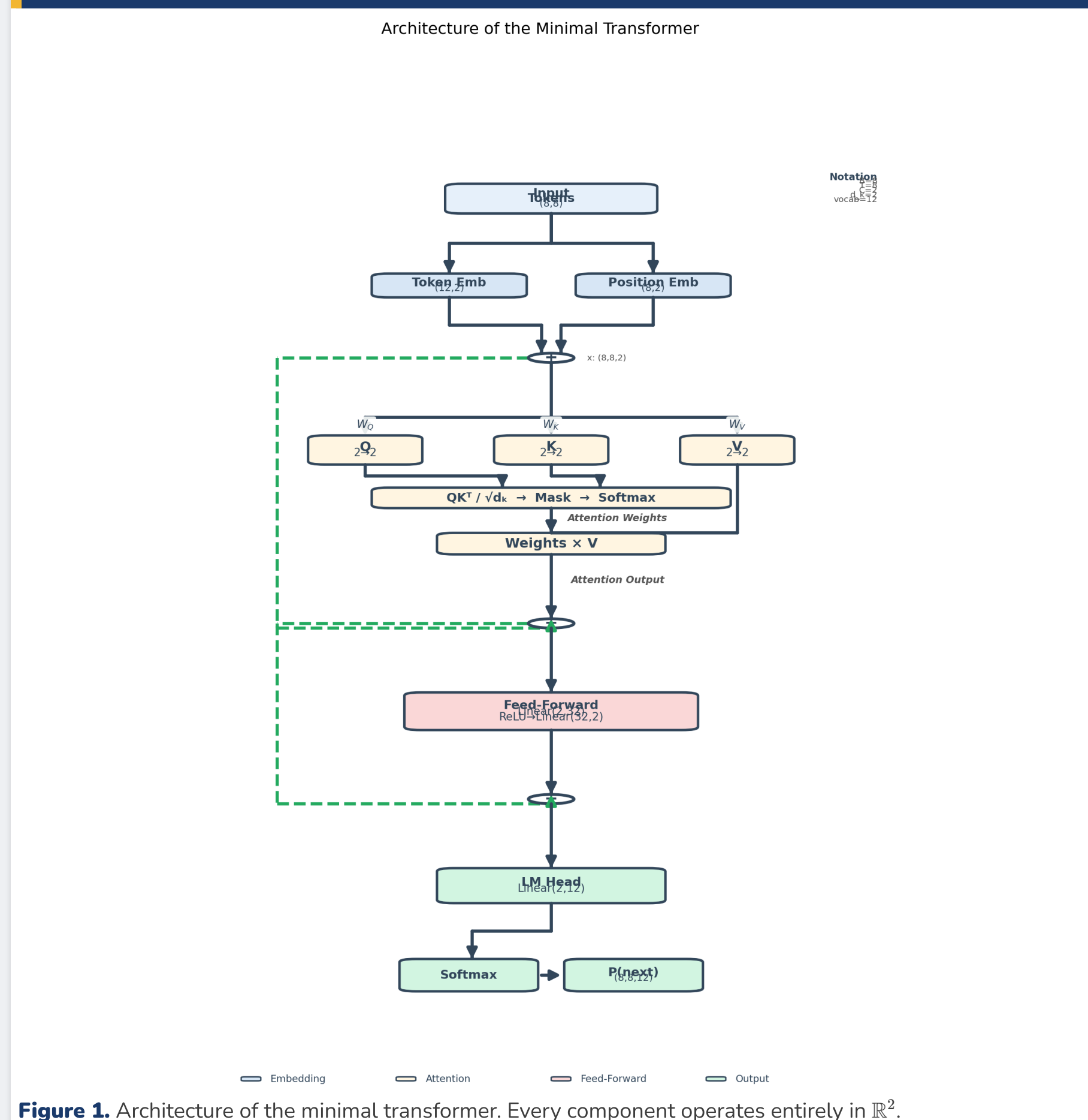
Figure 1. Architecture of the minimal transformer. Every component operates entirely in \mathbb{R}^2 .
