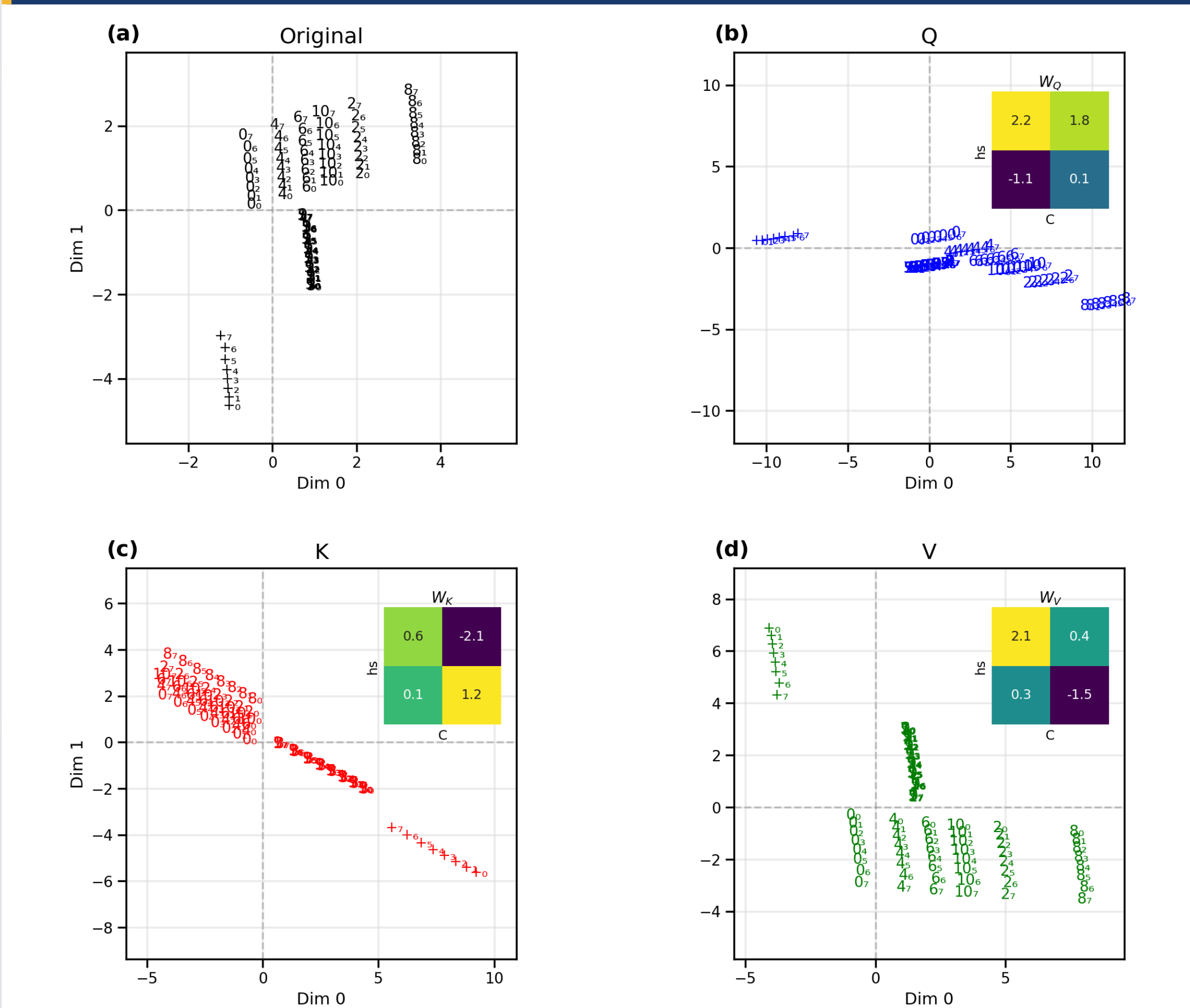
Figure 6. QKV projections. (a) Original combined token+position embeddings (as in Figure 5e). (b) Query-space (blue), with W_Q inset. (c) Key-space (red), with W_K inset. (d) Value-space (green), with W_V inset. All 96 token+position points in each panel.
