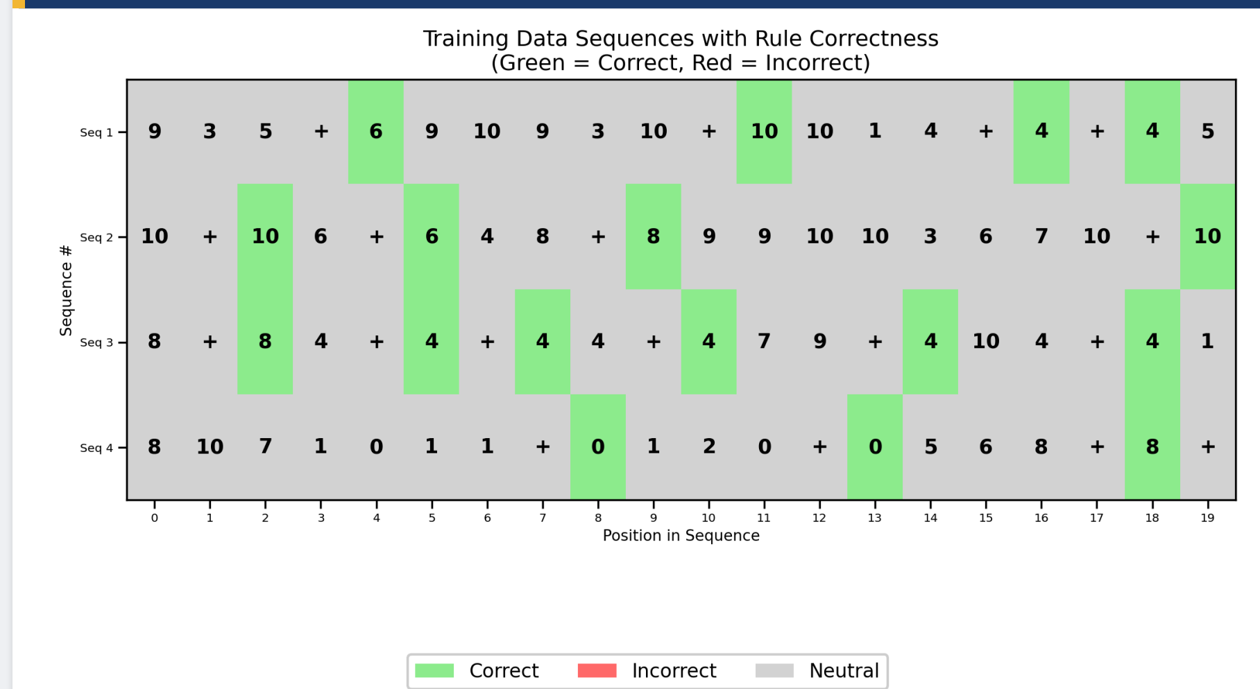
Figure 2. Sample training sequences as heatmaps. Green: constrained position (immediately following +) with the correct next token (the most recent even number). Gray: unconstrained position (any token is valid).
