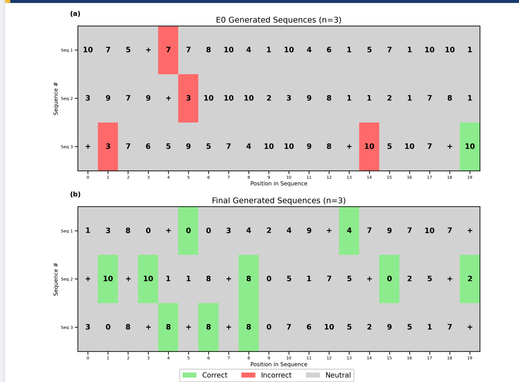
Figure 4. Model-generated sequences at initialization (top) vs. after training (bottom). Green = correct at constrained positions (after +), red = wrong at constrained positions, gray = unconstrained. Top: at step 0, constrained positions are mostly red (random predictions). Bottom: after training, constrained positions are mostly green (correct "last even" outputs).
