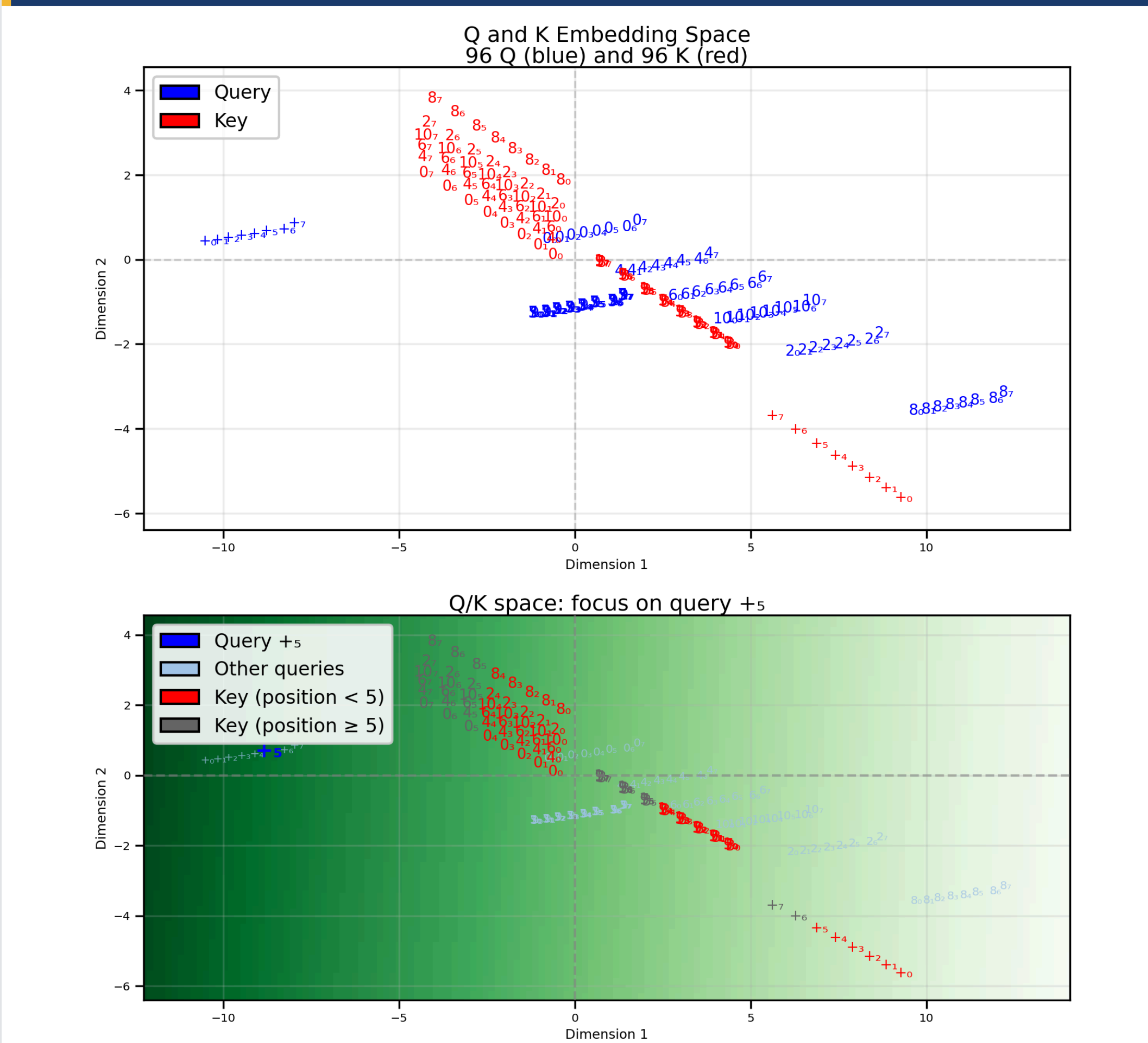
Figure 7. Query-key geometry in Q/K space. Top: joint query-key space (blue: queries; red: keys; labels show token and position). Bottom: Focus on the query +_5 (blue); background color indicates the dot product of the +_5 query with every point in space. Keys with position \geq 5 are grayed due to the causal mask.
