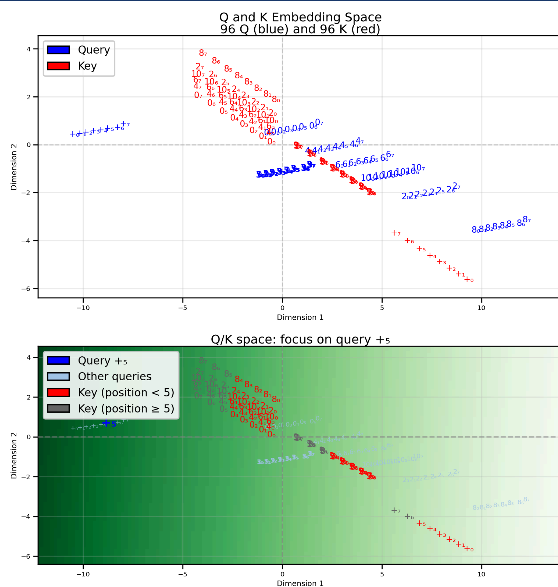
Figure 7. Query-key geometry in Q/K space. Top: joint query-key space (blue: queries; red: keys; labels show token and position). Bottom: Focus on the query +_5 (blue); background color indicates the dot product of the +_5 query with every point in space. Keys with position \geq 5 are grayed due to the causal mask.
