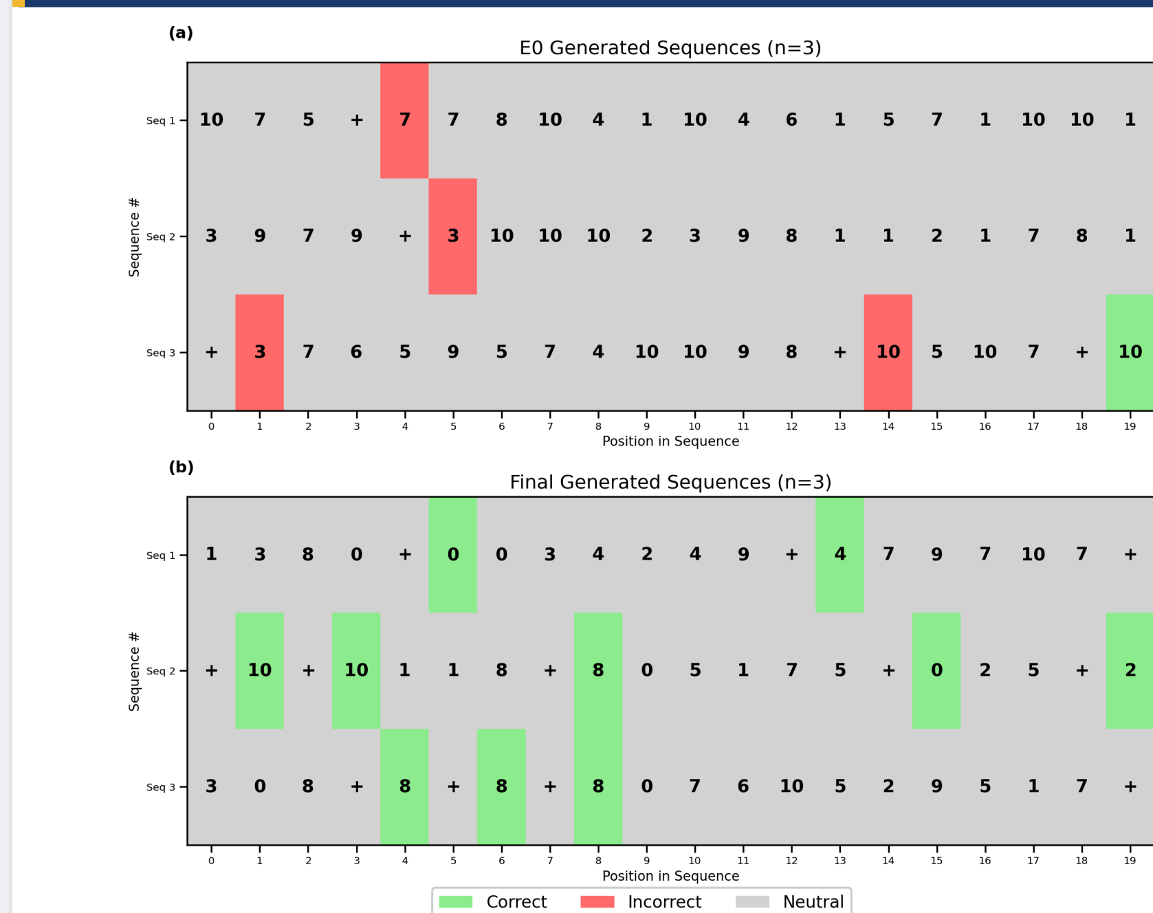
Figure 4. Model-generated sequences at initialization (top) vs. after training (bottom). Green = correct at constrained positions (after +), red = wrong at constrained positions, gray = unconstrained. Top: at step 0, constrained positions are mostly red (random predictions). Bottom: after training, constrained positions are mostly green (correct "last even" outputs).
