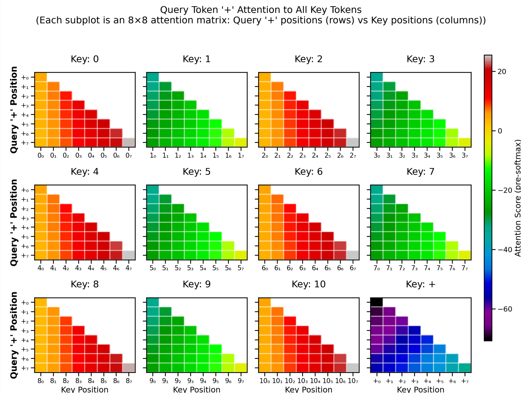
Figure 8. Pre-softmax query-key scores QK^T , restricted to + queries. Each subplot shows an 8x8 matrix of dot products: + query positions (rows) vs. key positions (columns) for a particular key token.
