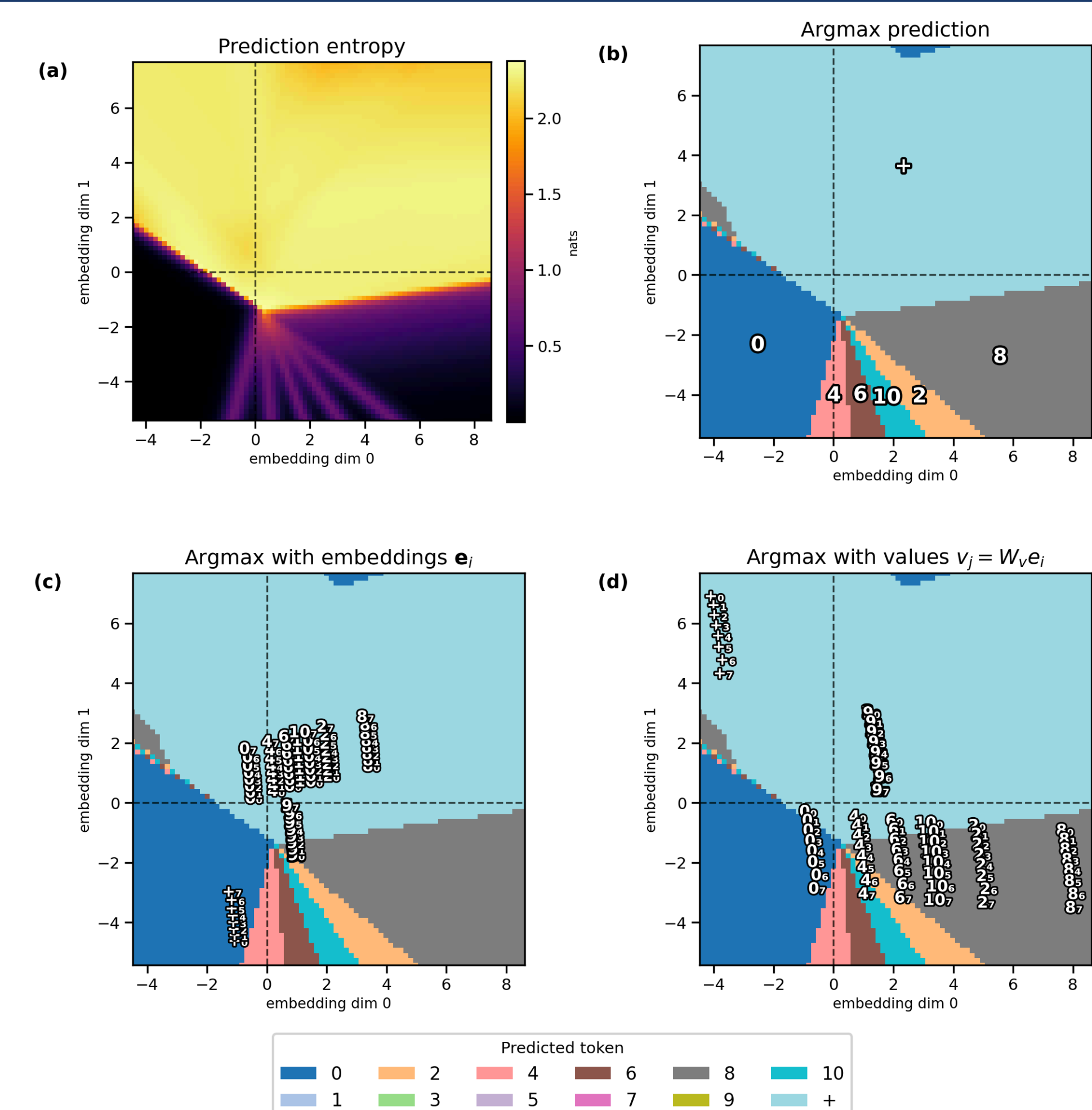
Figure 10. Output landscape summary (summary of Figure 9). (a) Entropy of the output distribution (nats); high in the indifference region (top half), near zero in even-number target zones (bottom half). (b) Argmax prediction map: color and annotation indicate which token has the highest predicted probability at each point. (c) Argmax map with combined embeddings e_i overlaid. (d) Argmax map with value-transformed vectors v_j overlaid.
