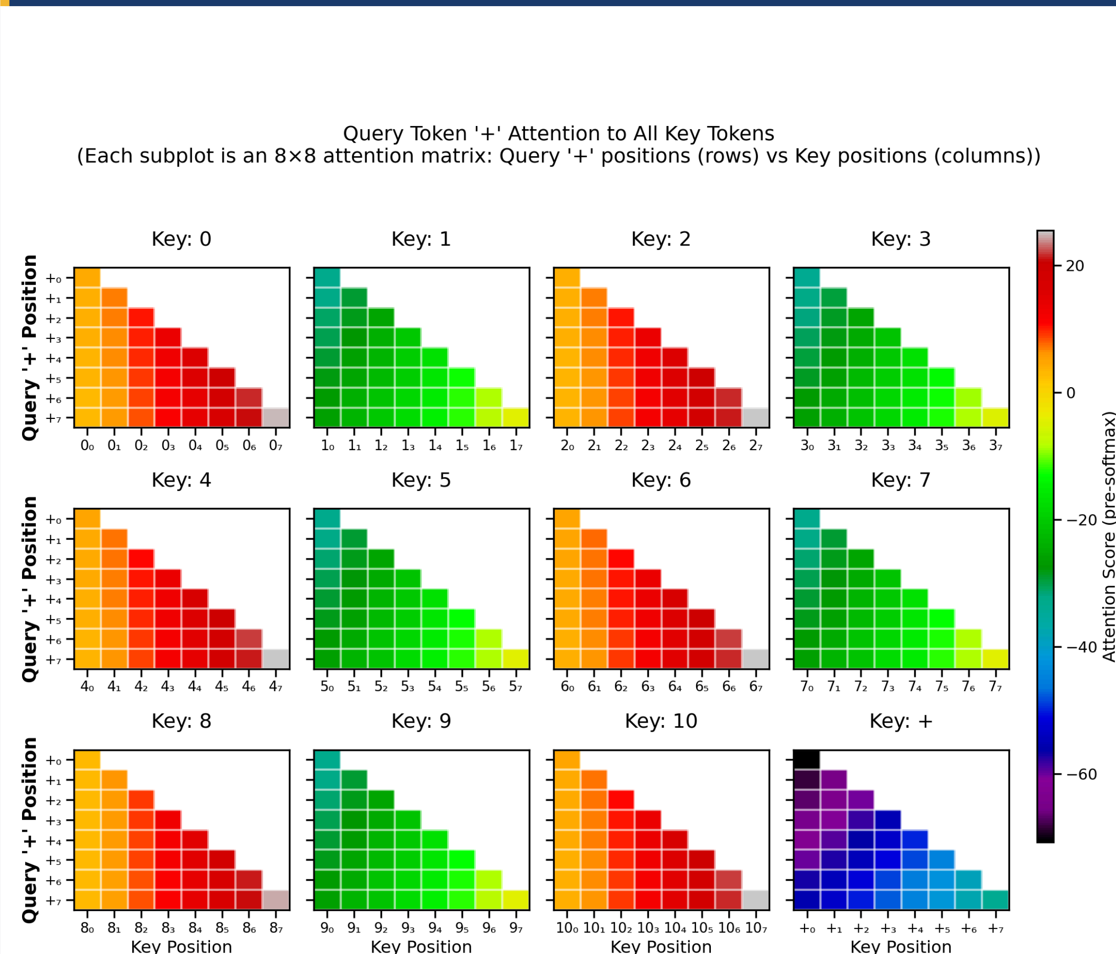
Figure 8. Pre-softmax query-key scores QK^T , restricted to + queries. Each subplot shows an 8x8 matrix of dot products: + query positions (rows) vs. key positions (columns) for a particular key token.
