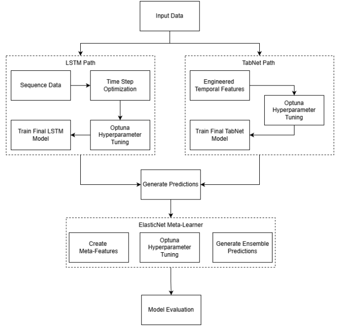
Figure 1. Proposed Ensemble Architecture.
