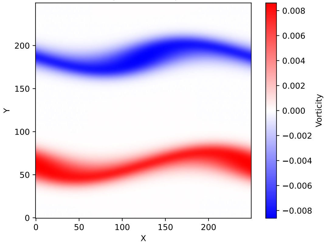
Vorticity at time step 3750
