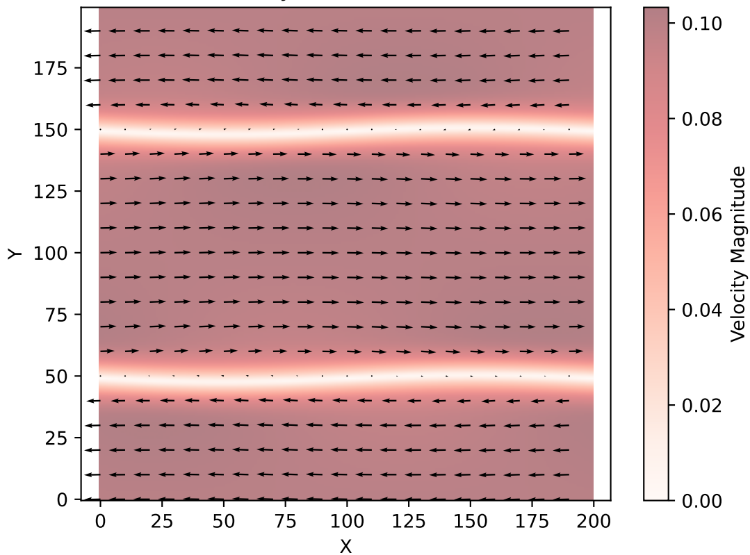
Velocity Field at t = 2000
