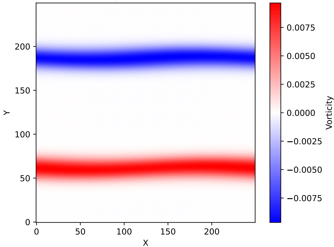
Vorticity at time step 2500
