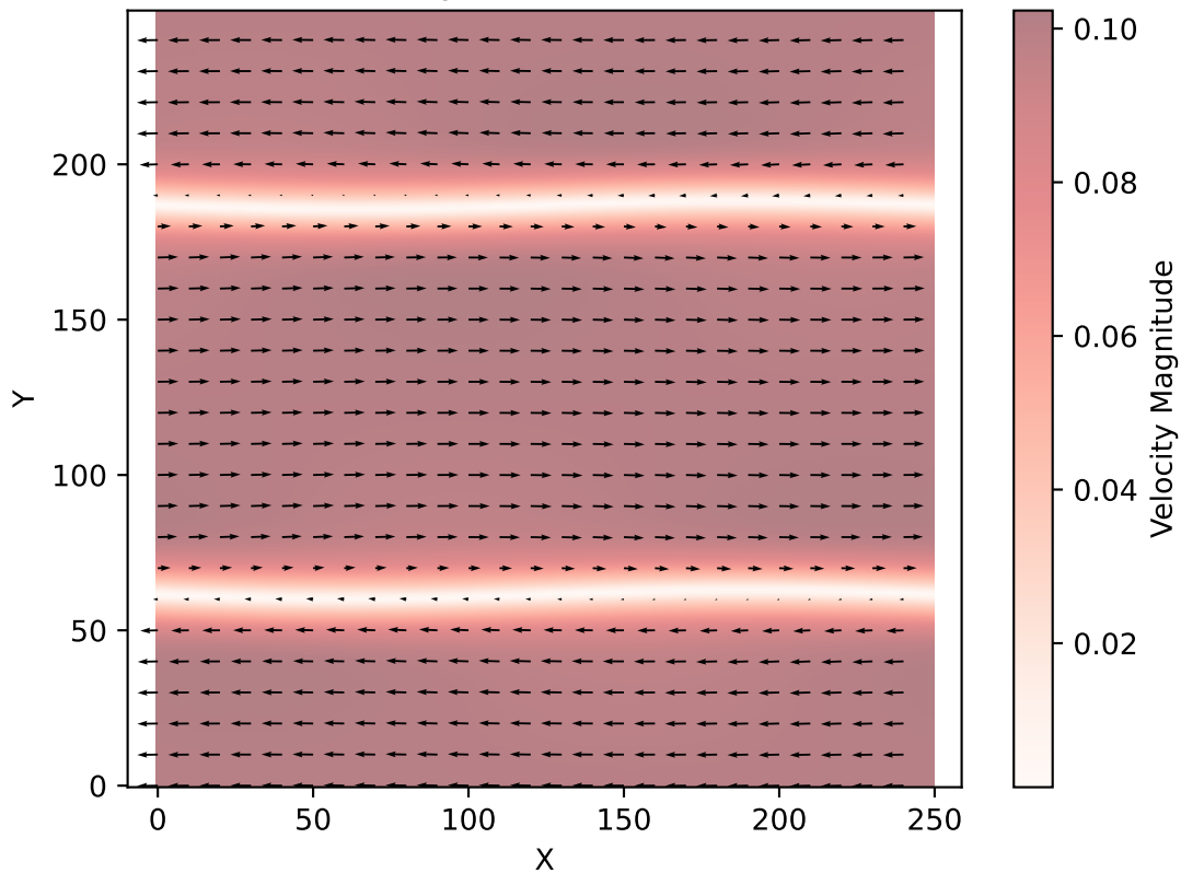
Velocity Field at t = 2500
