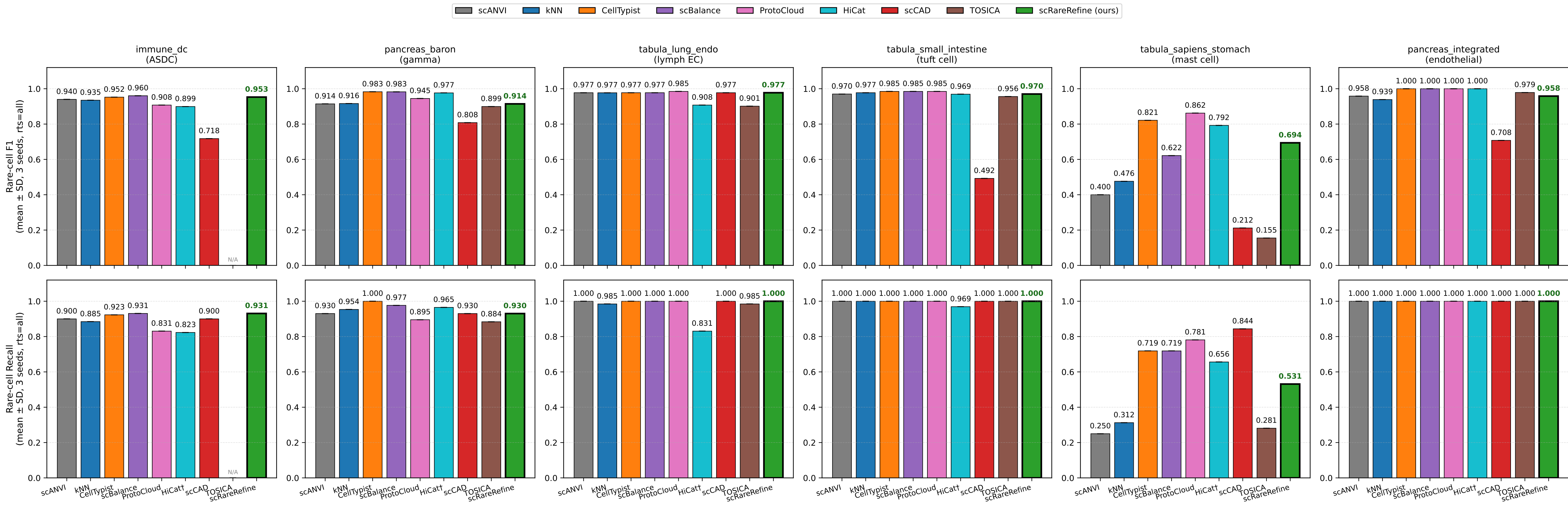
Comparison of rare-cell identification methods across 6 datasets (seed=42, rts=all)
