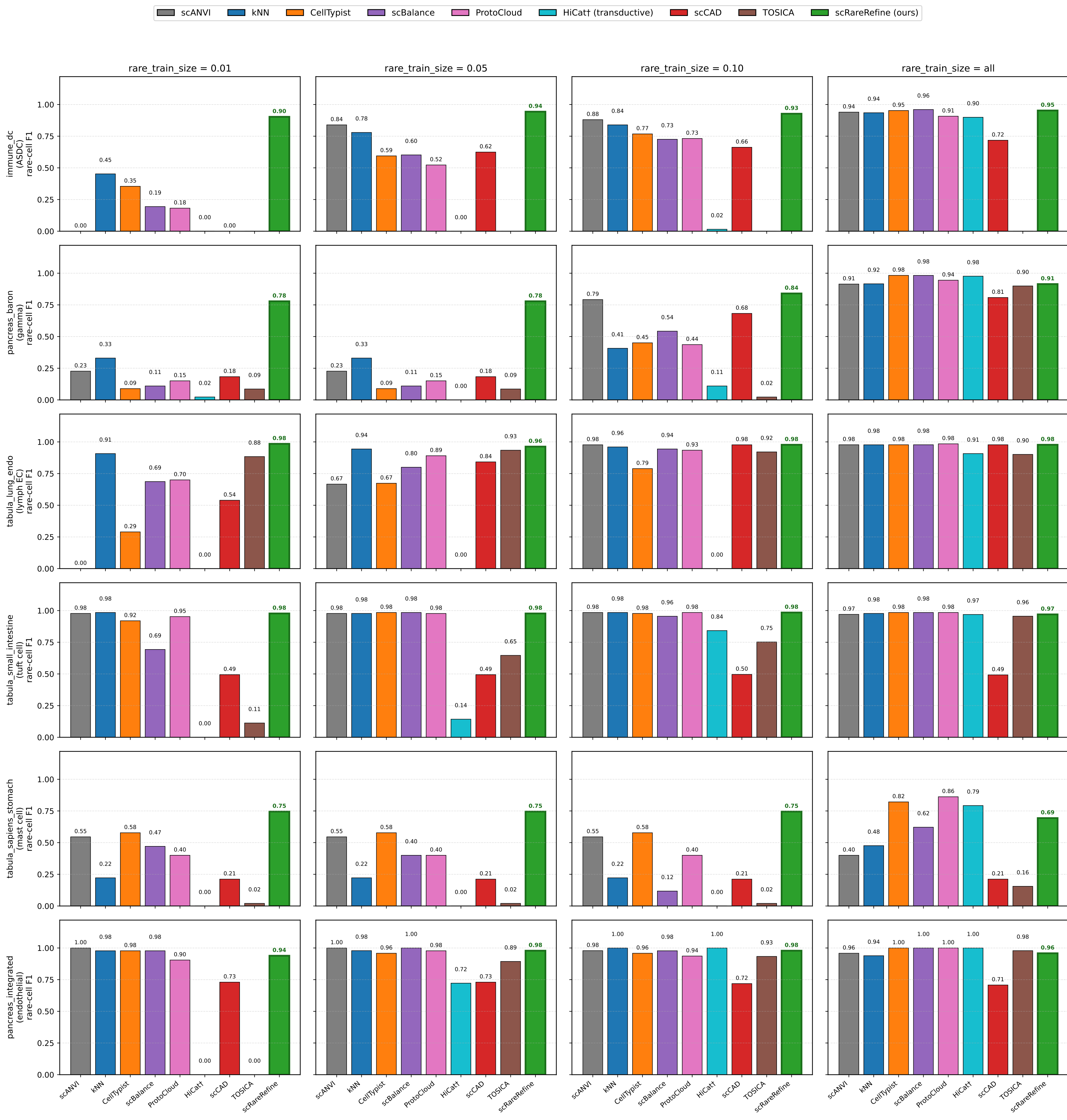
Rare-cell F1 by dataset (rows) × rare_train_size (cols) — scRareRefine vs. 8 baselines (seed=42)
