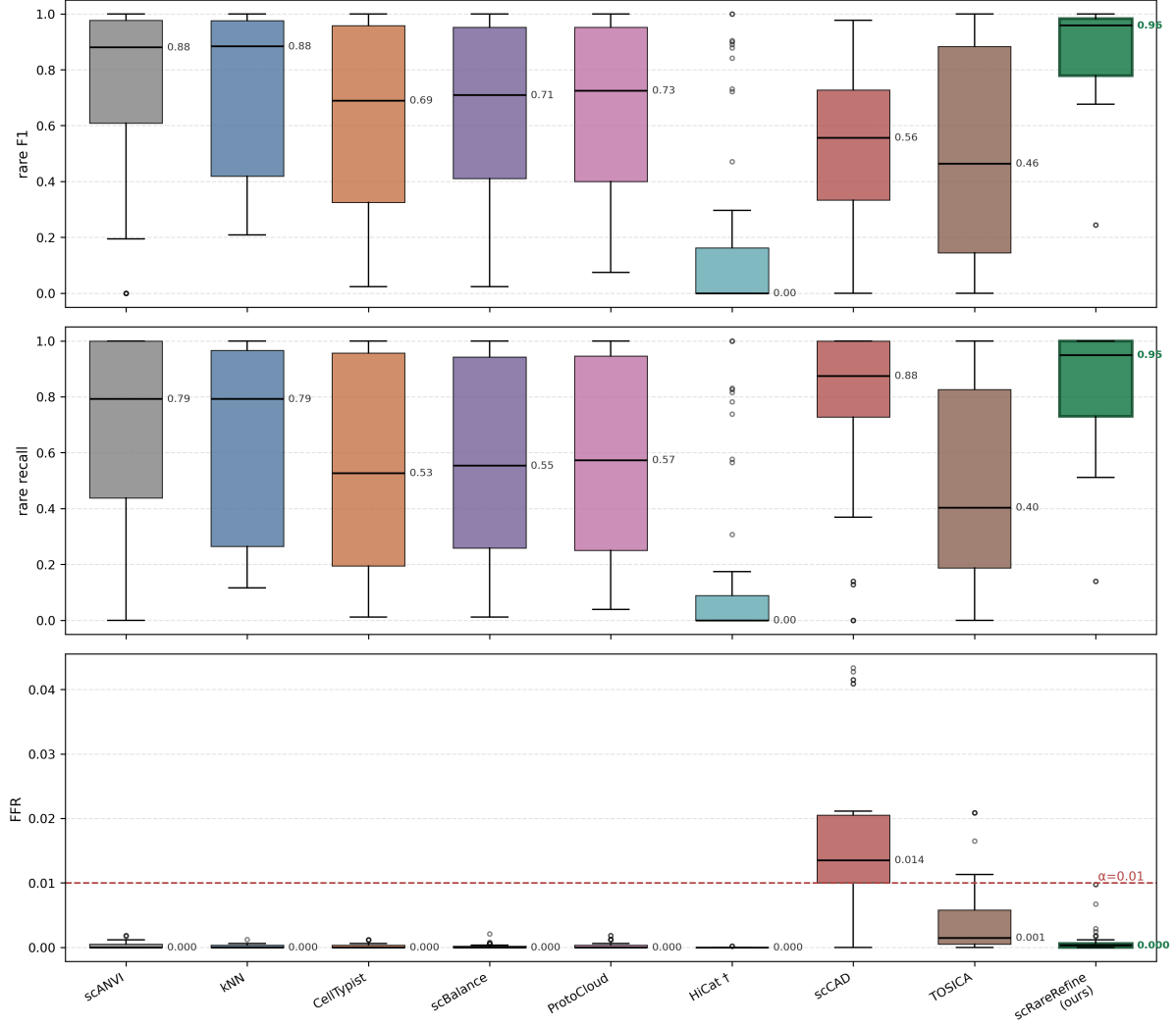
Figure 4: Across-dataset distribution in the label-scarce regime. Each box summarises a method over 54 scarce configurations (six datasets \times three fractions \times three seeds); the median is labelled. Top to bottom: rare-cell F1, rare-cell recall, FFR (dashed line is the budget \alpha = 0.01 ). scRareRefine has the highest and tightest F1/recall distributions and is the only method whose FFR box stays at zero, below the budget. † HiCat is transductive.
