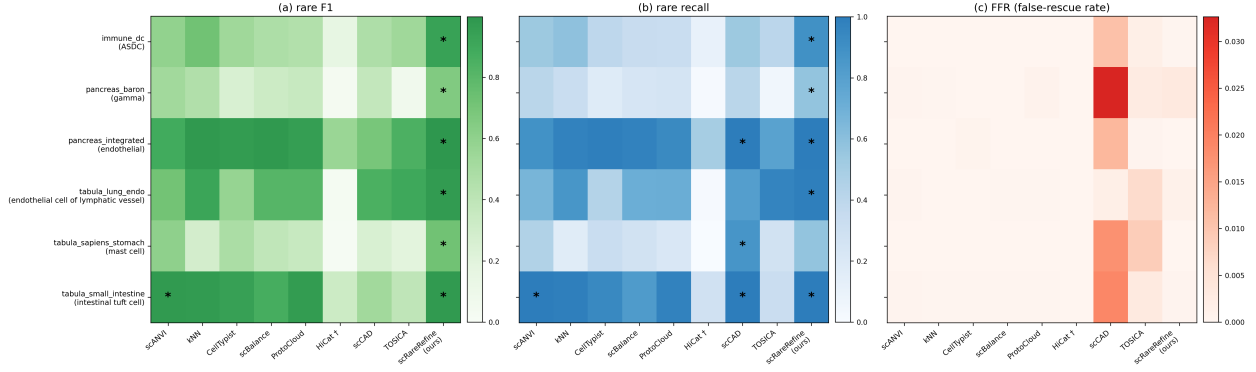
Figure 3: Per-method \times per-dataset comparison in the label-scarce regime ( p \leq 0.10 , mean over three fractions and three seeds). (a) rare-cell F1 and (b) rare-cell recall, with * marking the best method on each dataset; (c) FFR, where darker shading means more false rescues. scRareRefine (boxed column) is best or tied-best in F1 on five of six datasets while its FFR shading stays light throughout, whereas scCAD and TOSICA show the darkest FFR cells. † HiCat is transductive (upper-bound reference).
