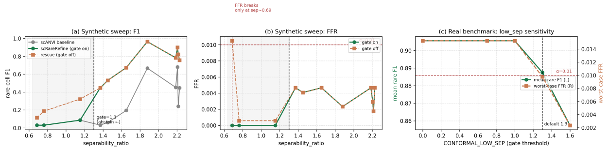
Figure 6: Separability-gate analysis. (a,b) Controlled semi-synthetic stress test (entangling a rare type toward its nearest majority): rescue stays FFR-safe well below the gate at 1.3. (c) Benchmark-wide sensitivity of the gate threshold: 1.3 is the smallest threshold that keeps worst-case FFR \leq \alpha on real data.
