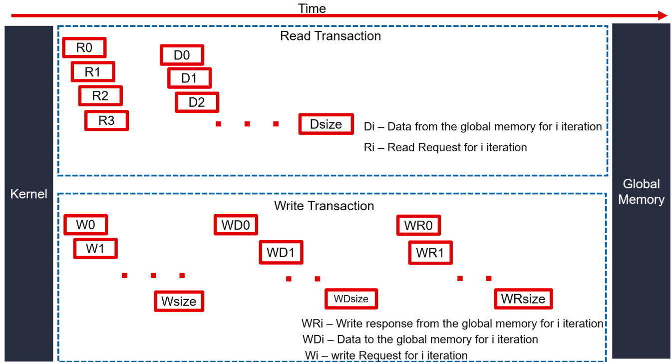
Figure 64: Pipeline Burst
