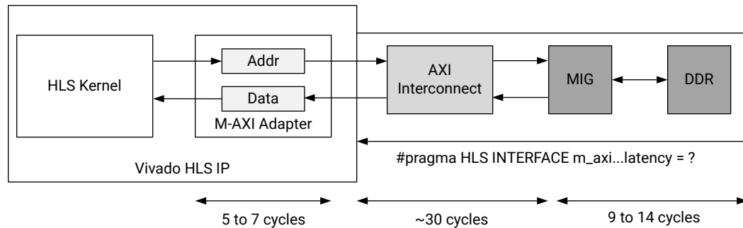
Figure 66: Burst Transaction Diagram
