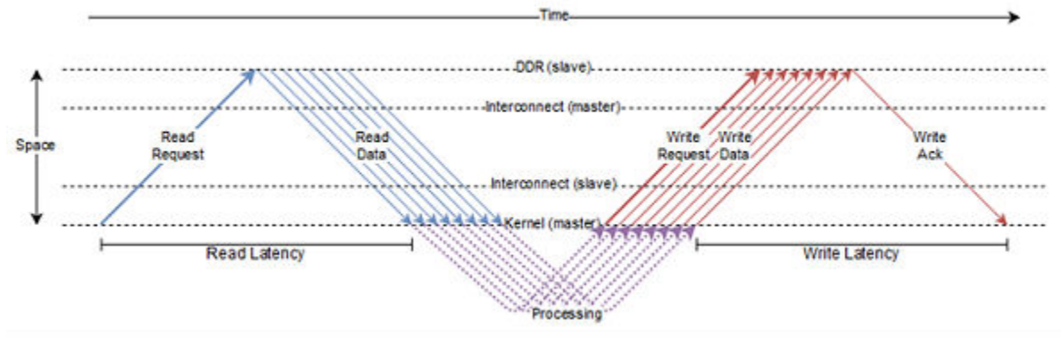
Figure 63: AXI Protocol
