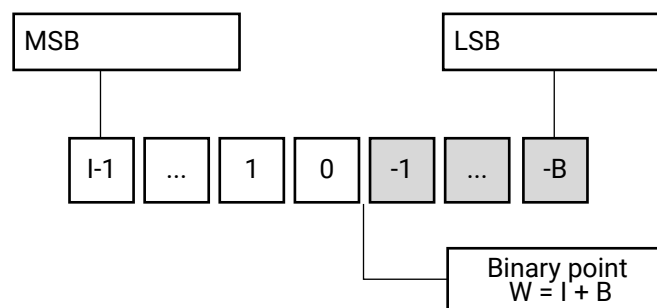
Figure 145: Fixed-Point Data Type
