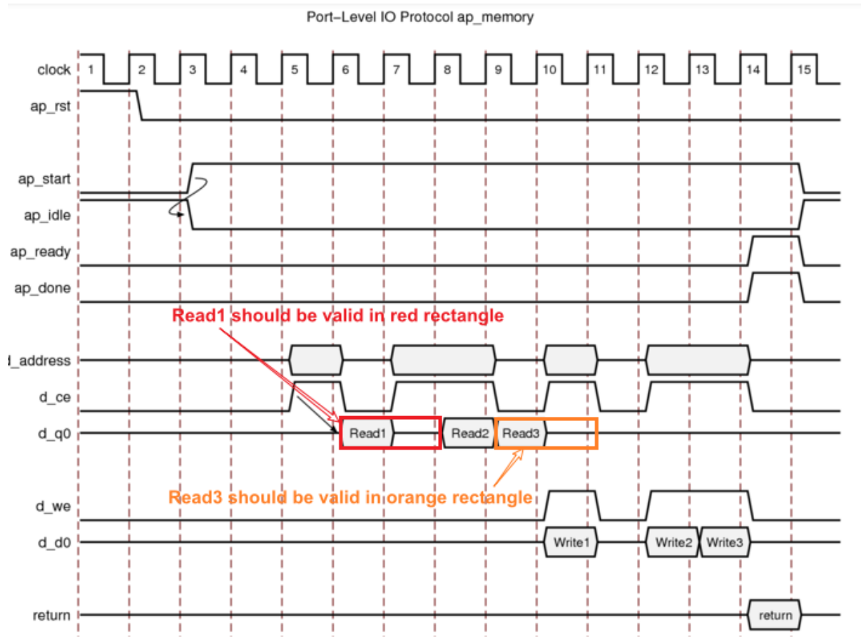
Figure 51: Behavior of ap_memory Interface with Latency 1
