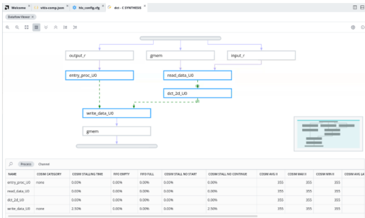
Figure 128: Dataflow Viewer
