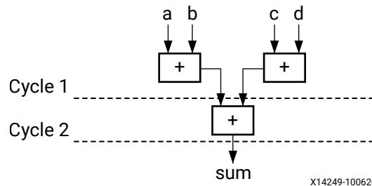
Figure 62: Adder Tree After Balancing
