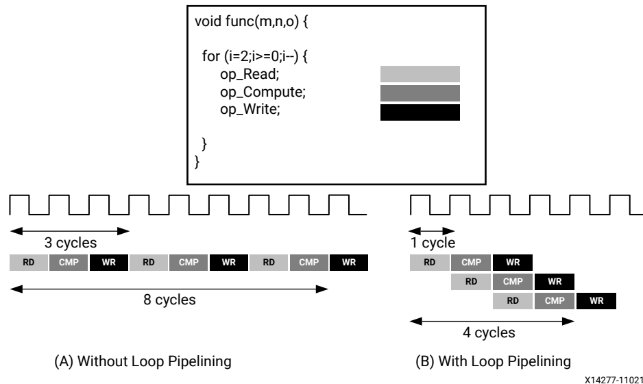
Figure 144: Loop Pipeline
