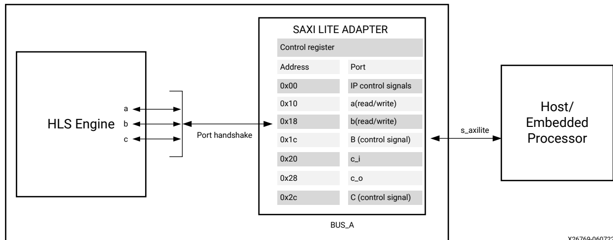
Figure 43: S_AXILITE Adapter
