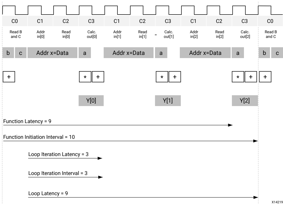
Figure 60: Latency and Initiation Interval Example
