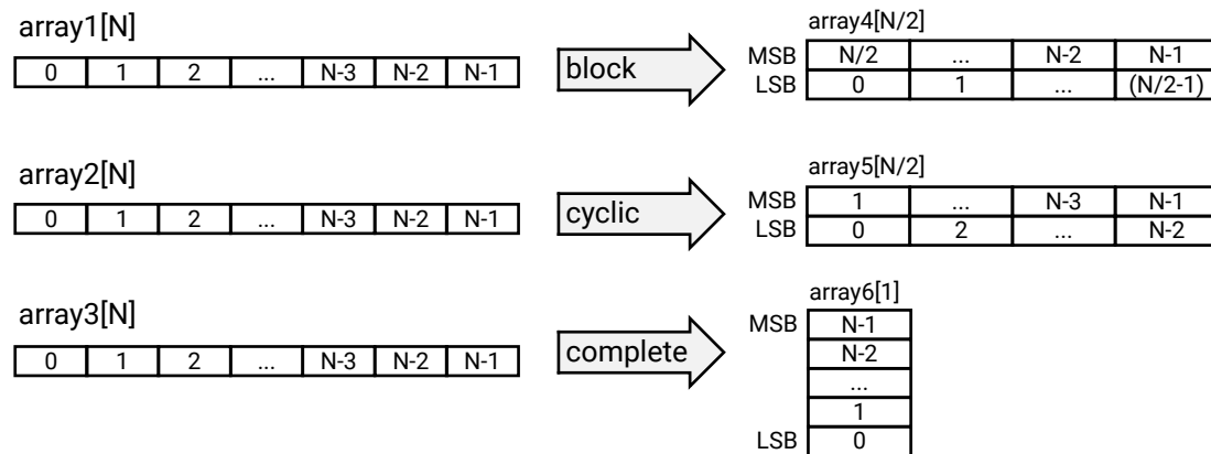
Figure 142: ARRAY_RESHAPE Pragma
