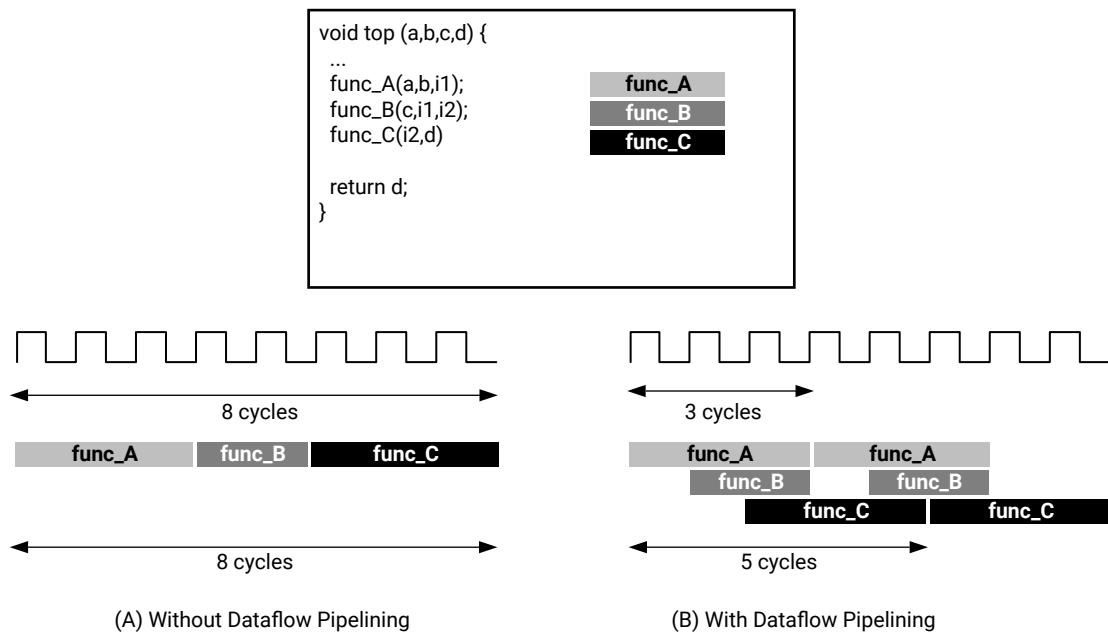
Figure 143: DATAFLOW Pragma
