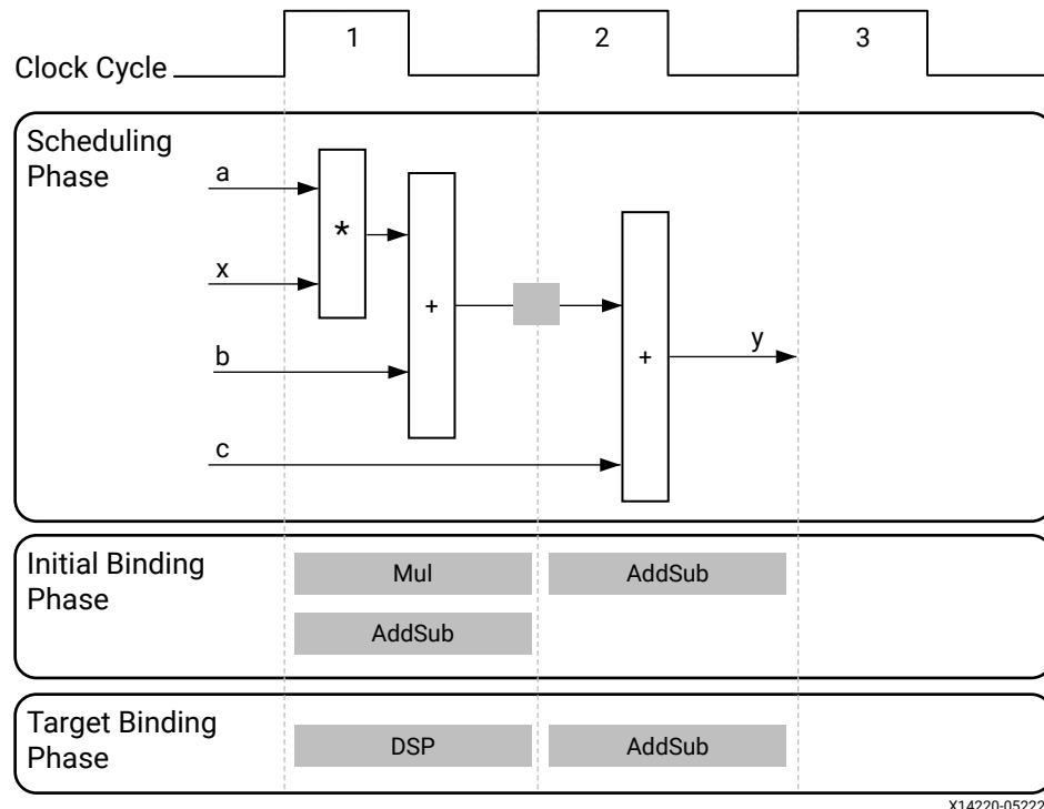
Figure 58: Scheduling and Binding Example
