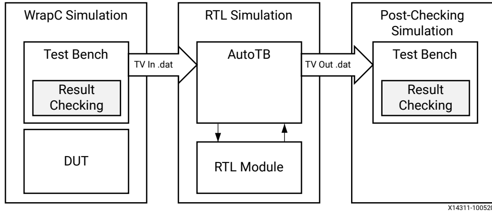
Figure 131: C/RTL Verification Flow
