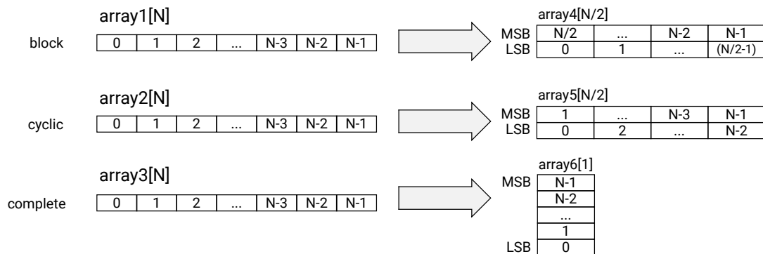
Figure 29: Array Reshaping
