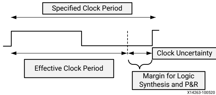
Figure 102: Clock Period and Margin
