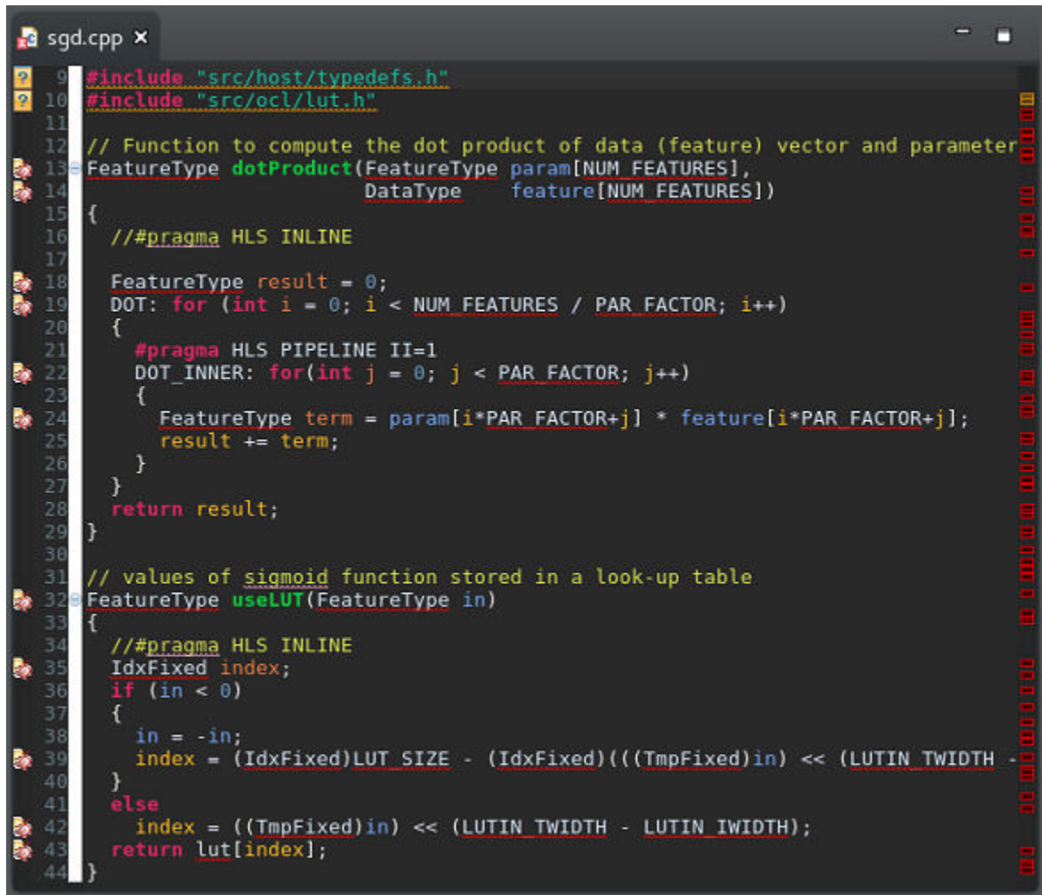
Figure 93: Unresolved References
