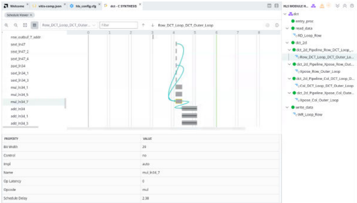
Figure 125: Schedule Viewer
