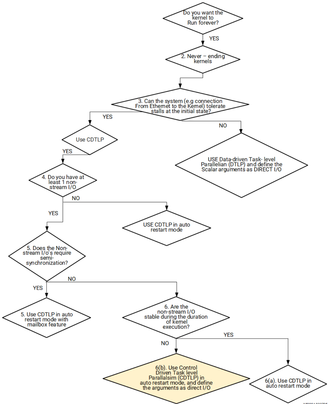
Figure 55: Kernel Flow Chart
