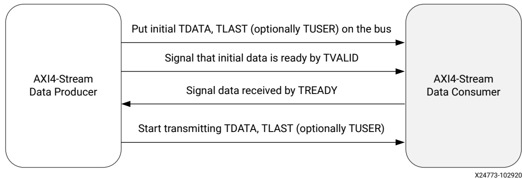
Figure 45: AXI4-Stream Handshake
