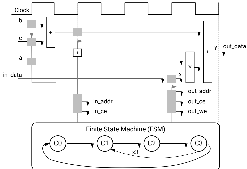
Figure 59: Control Logic Extraction and I/O Port Implementation Example
