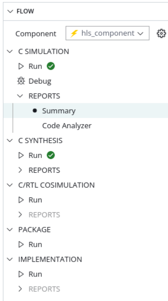
Figure 84: Flow Navigator
