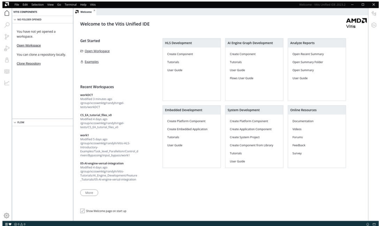
Figure 82: Welcome Screen
