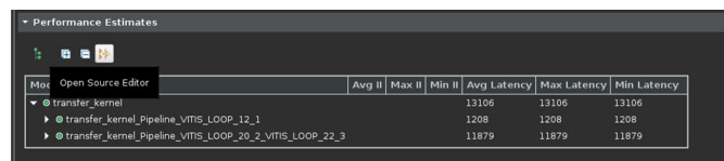
Figure 74: Performance Estimates
