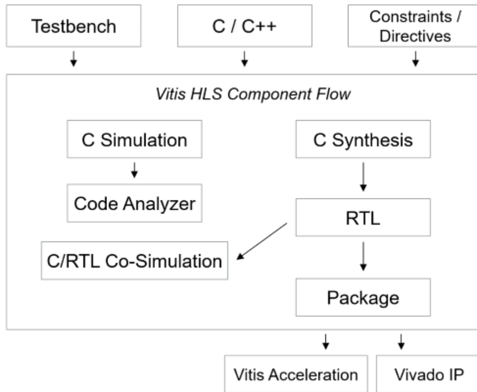
Figure 85: Vitis HLS Development Flow
