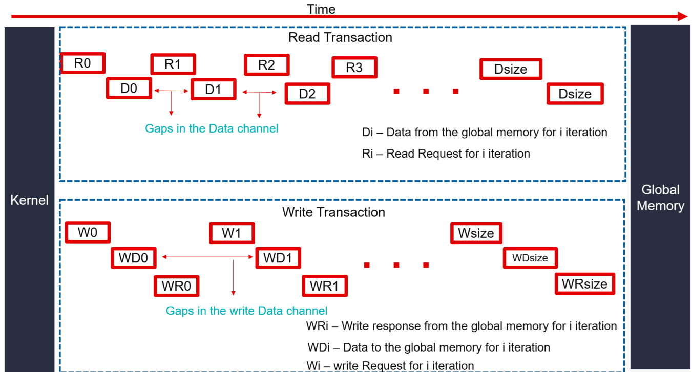
Figure 65: Sequential Burst
