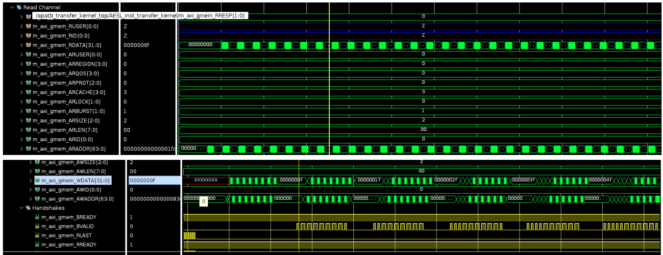
Figure 73: Performance Impacts
