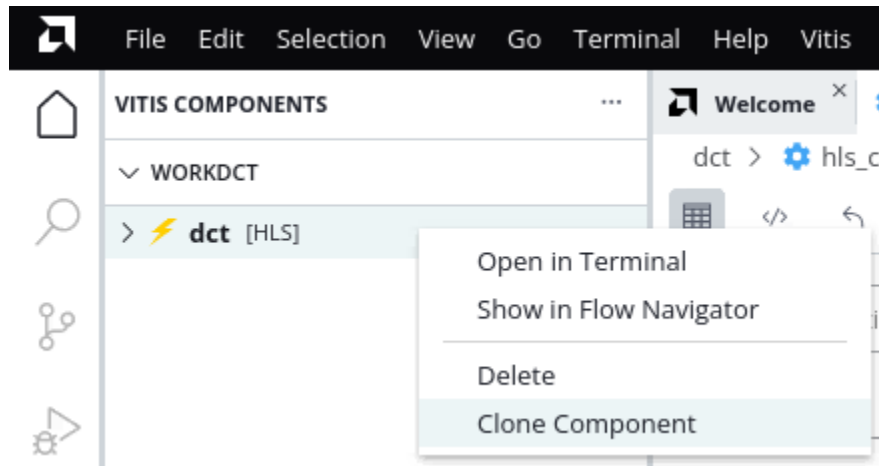
Figure 140: Clone Component
