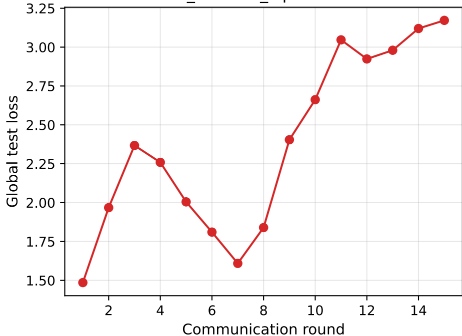
ablation_dirichlet_alpha0.01 — loss
