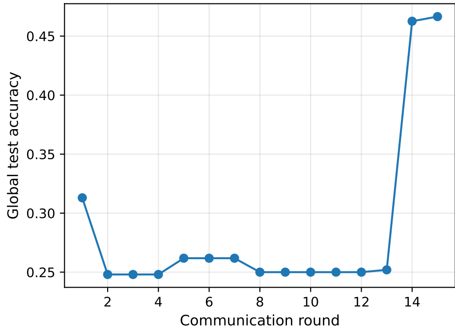
ablation_dirichlet_alpha0.01 — accuracy
