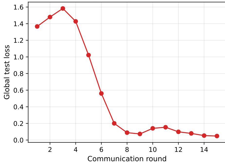
ablation_dirichlet_alpha0.5 — loss
