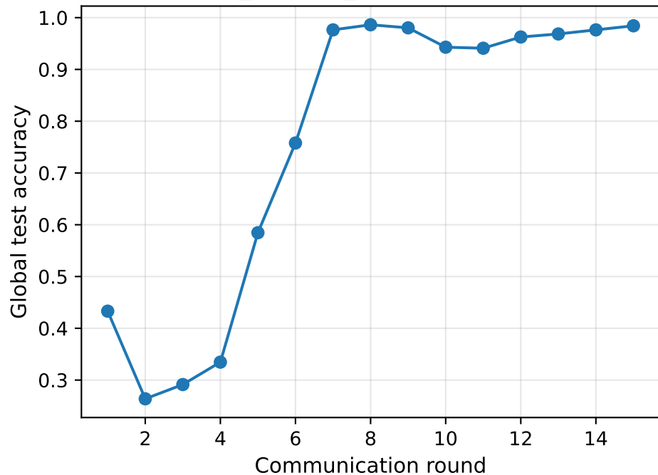
ablation_dirichlet_alpha0.5 — accuracy
