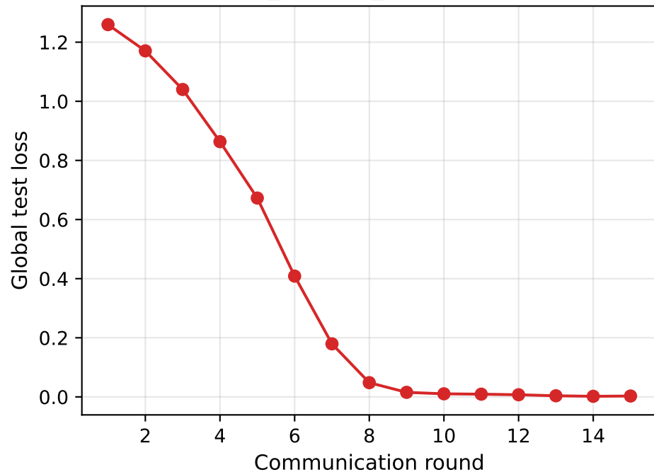
ablation_dirichlet_alpha1.0 — loss
