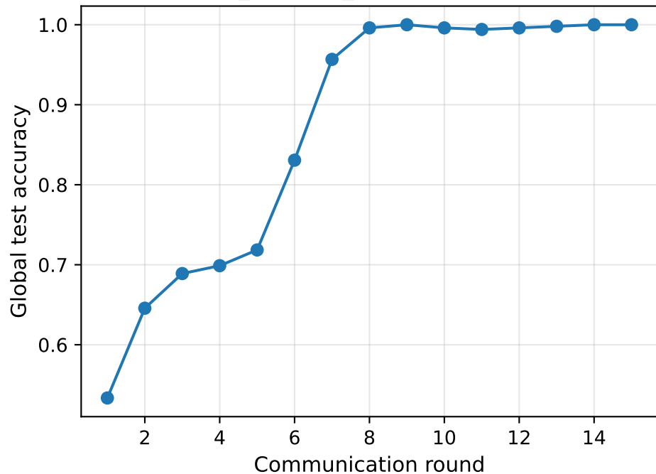
ablation_dirichlet_alpha1.0 — accuracy
