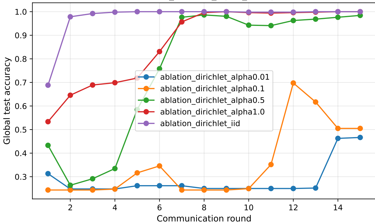
ablation_dirichlet_alpha_sweep
