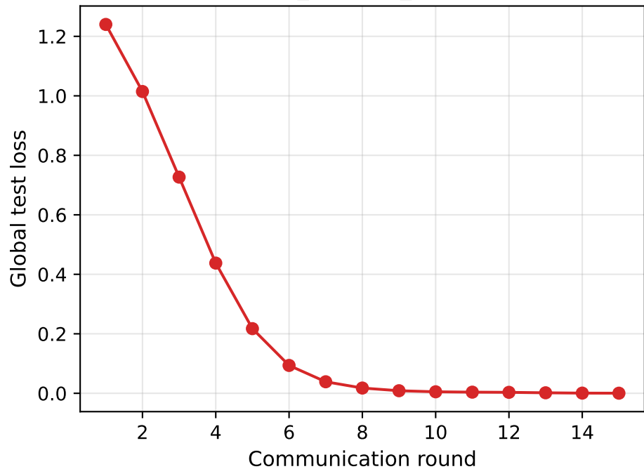
ablation_dirichlet_iid — loss
