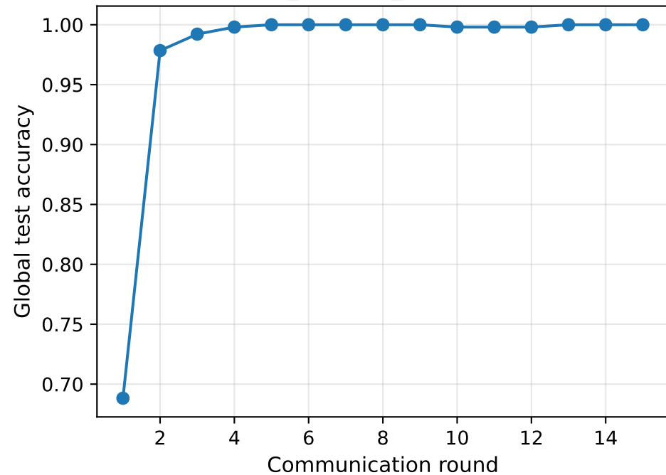
ablation_dirichlet_iid — accuracy
