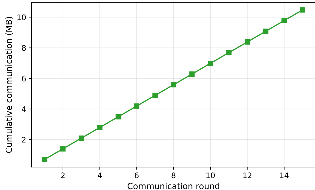
ablation_dirichlet_iid — communication cost
