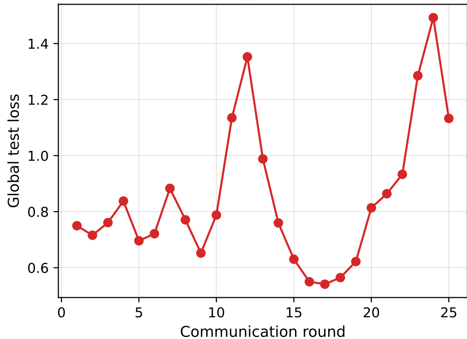
fatellm_lora_sent140 — loss
