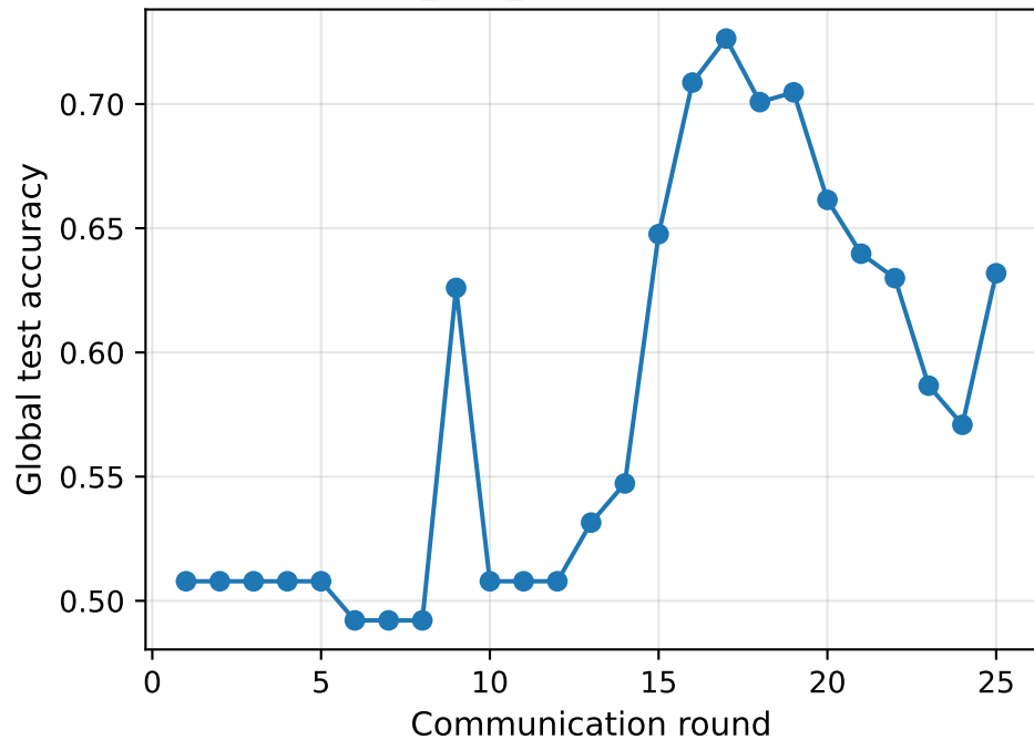
fatellm_lora_sent140 — accuracy
