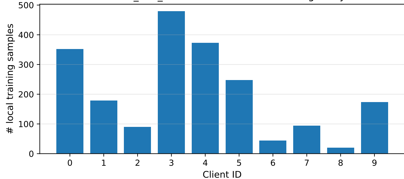
fatellm_lora_sent140 — client data heterogeneity
