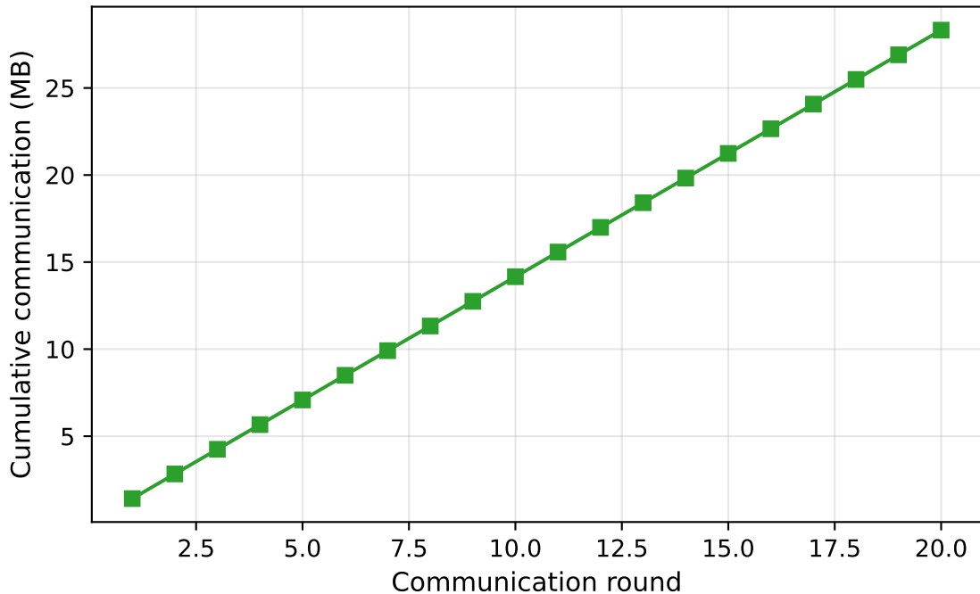
fatellm_lora_synthetic — communication cost
