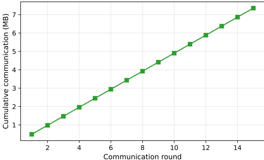
fedpeptao_shakespeare — communication cost
