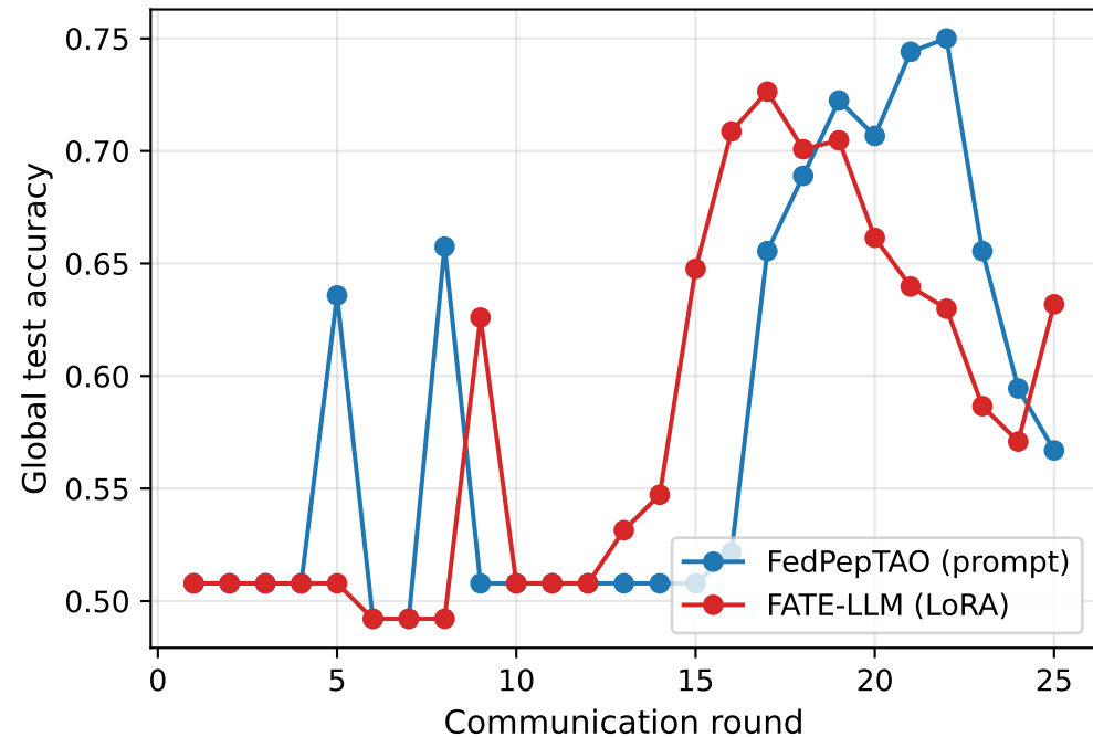
Sent140 — accuracy
