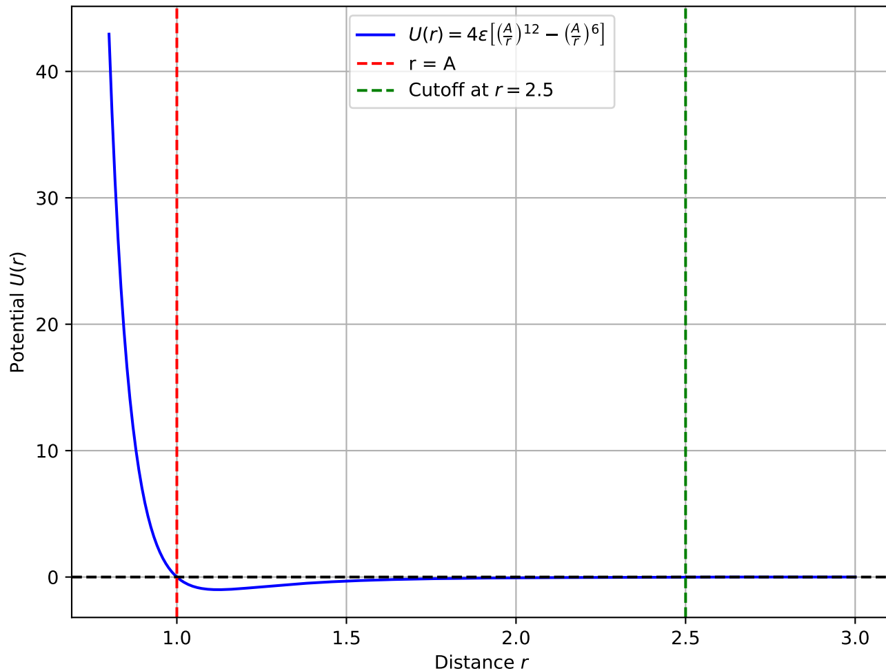
Lennard-Jones Potential with Cutoff
