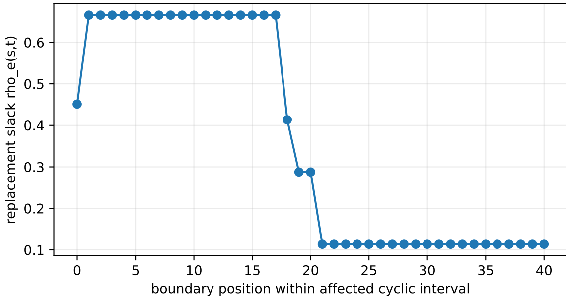
Replacement-slack profile from the pre-proof falsification suite
