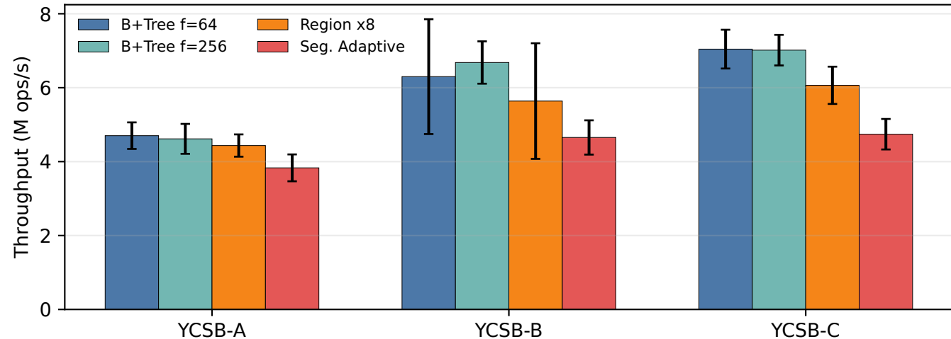
Stationary YCSB Workloads
