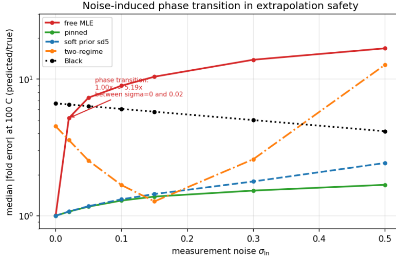
Figure 2: Noise-induced phase transition in extrapolation safety. The free corrected equation (red) is exact at \sigma_{\text{ln}} = 0 and collapses discontinuously at \sigma_{\text{ln}} = 0.02 ; pinned (green) and soft-prior (blue) variants are flat and graceful; the two-regime incumbent (orange) shows a false-confidence minimum near \sigma_{\text{ln}} = 0.15 and collapses at \sigma_{\text{ln}} = 0.5 ; Black’s equation (black) is uniformly wrong and noise-insensitive.
