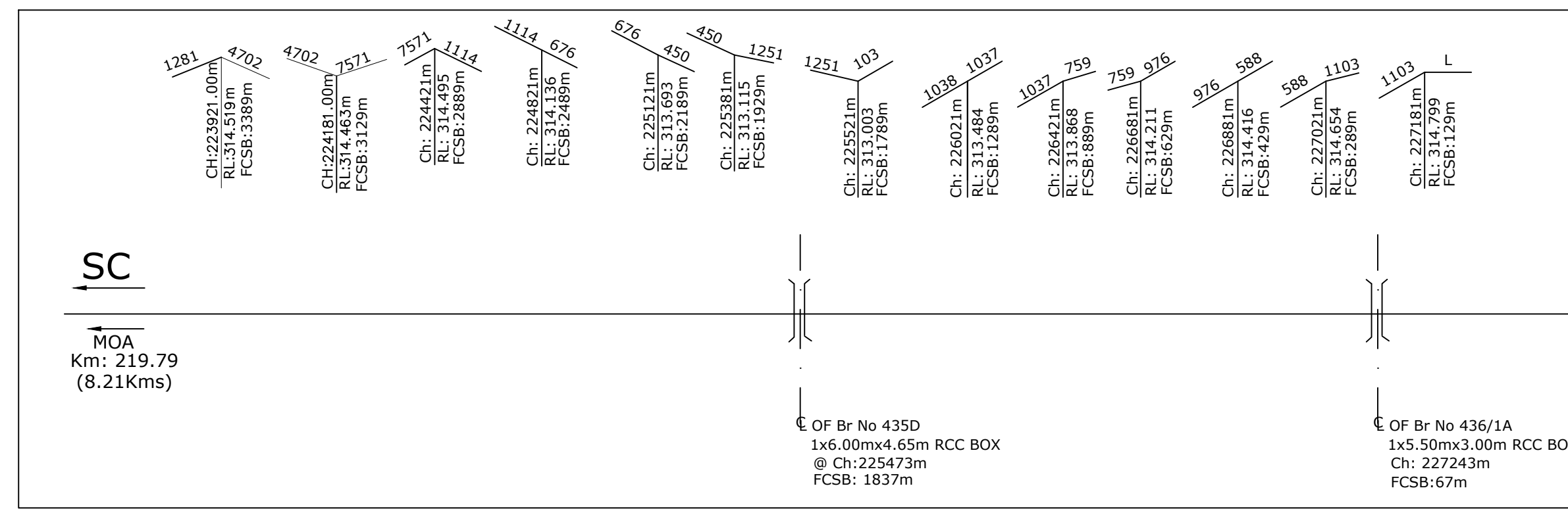
3 Km DETAILS ON SC END
