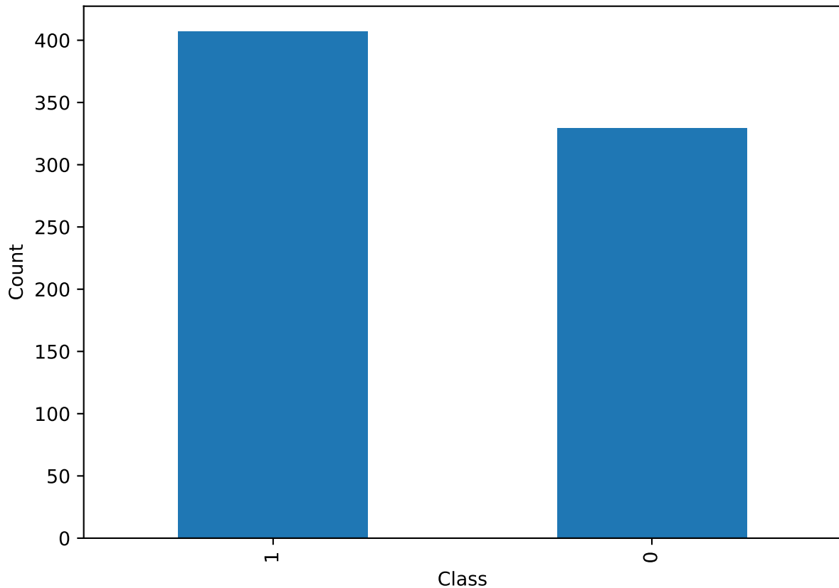
Target Variable Distribution
