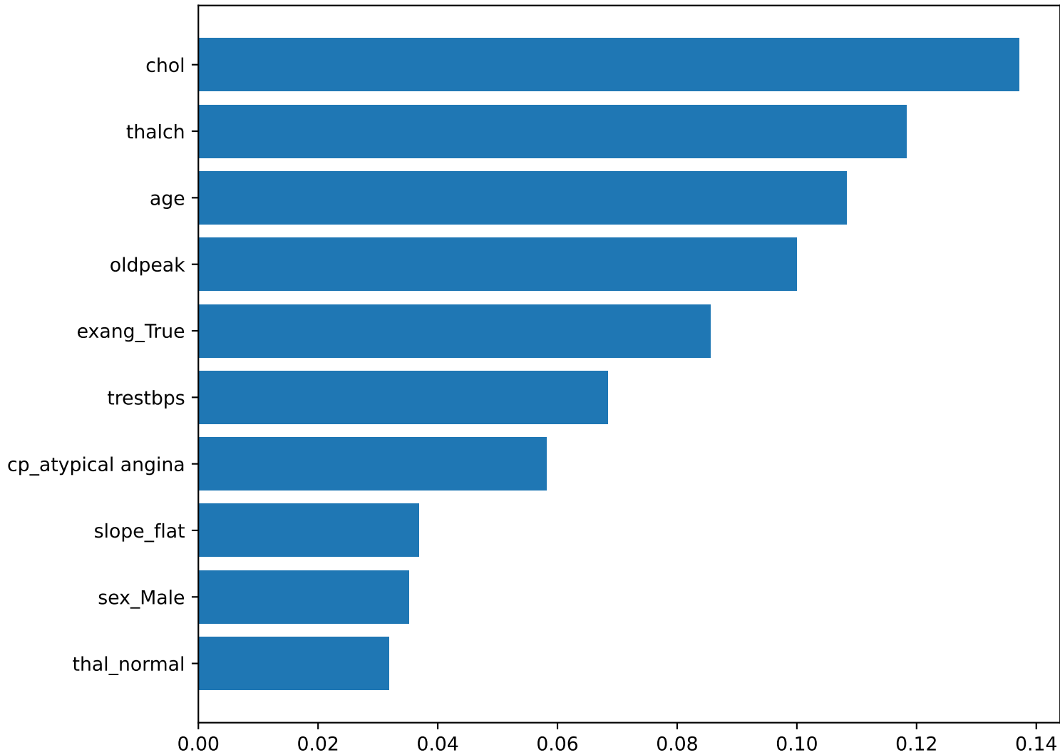
Top 10 Feature Importances (Random Forest)
