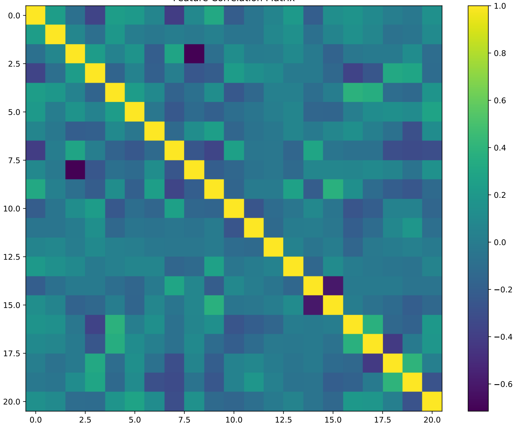
Feature Correlation Matrix
