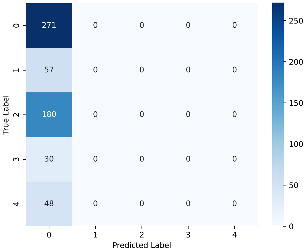
CNN Confusion Matrix (RQ1)
