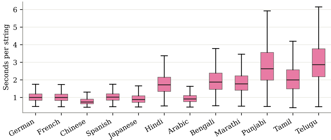
Qwen2.5-Coder-7B latency by target language (outliers hidden)
