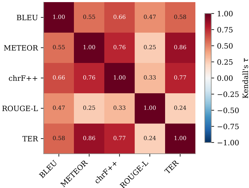
Metric agreement (66 system-language pairs)
