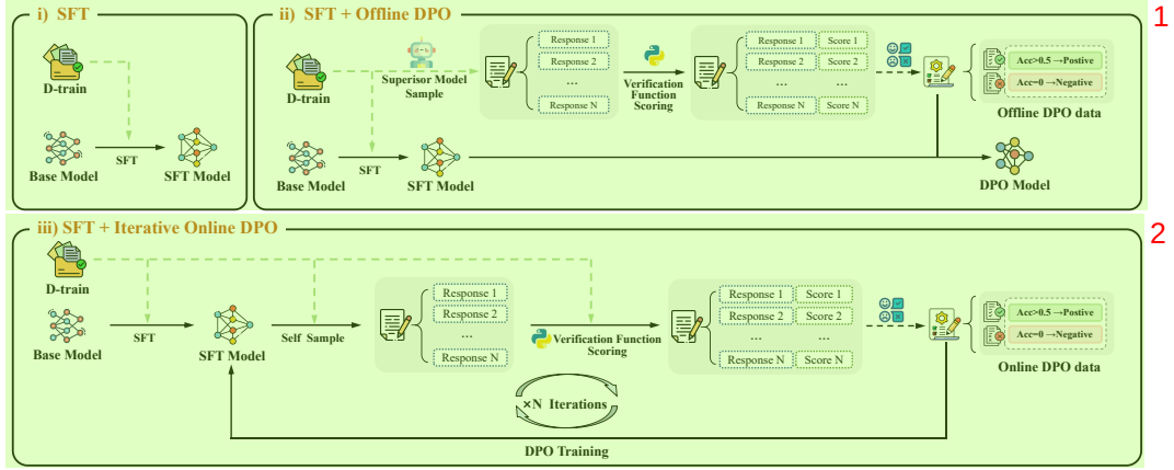
Figure 3: Different training strategies that can be adapted with synthetic dataset generated by AUTOIF. 3
