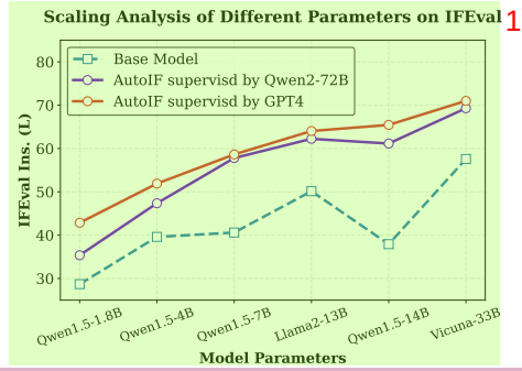
Figure 5: The scaling analysis of various parameter sizes between the base model and different supervision models on the IFEval benchmark.
