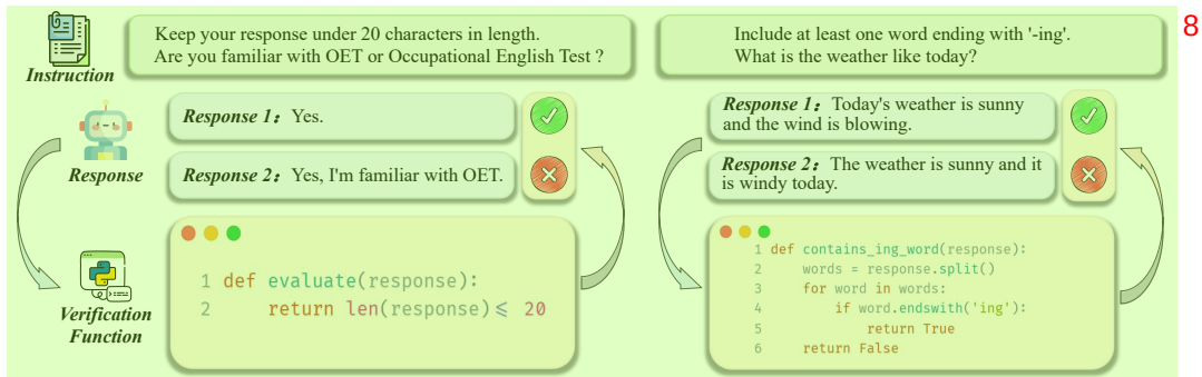
Figure 1: An example of the verification function automatically assesses the adherence of responses to the instruction’s constraints. 8
