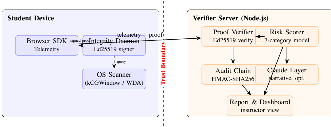
Fig. 1. Simurgh system architecture. The student device runs a browser SDK (telemetry collection) and a local integrity daemon (Ed25519-signed proofs of OS metadata). The daemon queries OS-level window-state metadata without accessing content. All proof material crosses the trust boundary to the Node.js verifier, which checks signatures, scores risk, appends to the audit chain, optionally invokes the Claude narrative layer, and exposes a read-only instructor dashboard and report.
