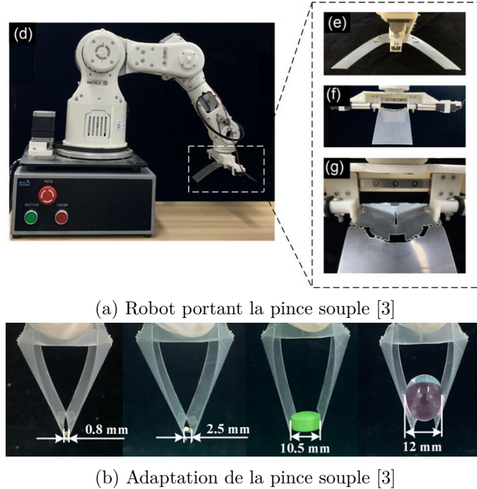
FIGURE 2.1 – Pince en PVC souple
