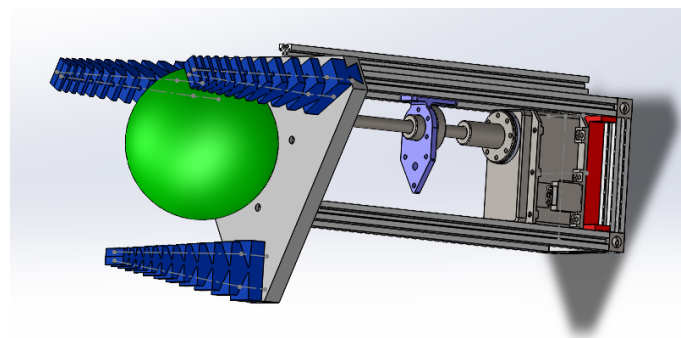
FIGURE III.10 – Accouplement de notre pince
